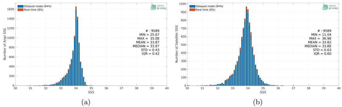
Figure 2: Histograms of SSS from Argo (a) and SMOS SSS L3 v8 - 9 Days (CATDS-CECOS-LOCEAN) (b) considering all match-up pairs per bins of 0.1 over the Sea of Japan Pi-MEP region and for the full satellite product period.
