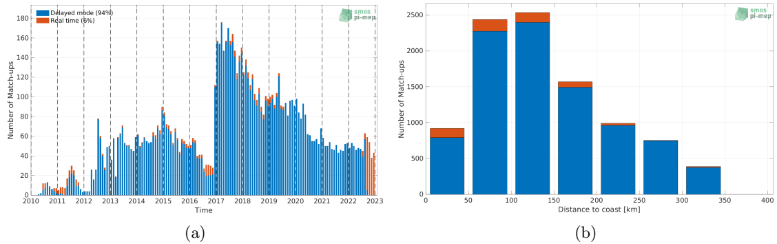
Figure 1: Number of match-ups between Argo and SMOS SSS L3 v8 - 9 Days (CATDS-CECOS-LOCEAN) SSS as a function of time (a) and as function of the distance to coast (b) over the Sea of Japan Pi-MEP region and for the full satellite product period.
