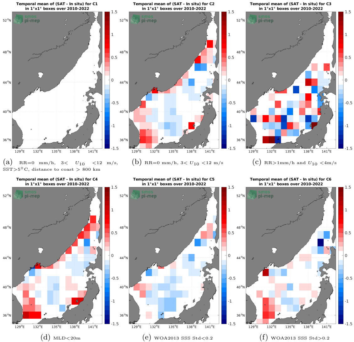
Figure 12: Temporal mean gridded over spatial boxes of size 1^\circ \times 1^\circ of \Delta SSS (SMOS SSS L3 v8 - 9 Days (CATDS-CECOS-LOCEAN) - Argo) for 6 different subdatasets corresponding to: RR=0 mm/h, 3 < U_{10} < 12 m/s, SST > 5^\circ\text{C} , distance to coast > 800 km (a), RR=0 mm/h, 3 < U_{10} < 12 m/s (b), RR > 1 mm/h and U_{10} < 4 m/s (c), MLD < 20 m (d), WOA2013 SSS Std < 0.2 (e), WOA2013 SSS Std > 0.2 (f).
