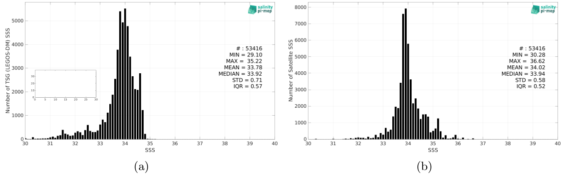
Figure 2: Histograms of SSS from TSG (LEGOS-DM) (a) and SMOS SSS L3 v8 - 18 Days (CATDS-CEC-LOCEAN) (b) considering all match-up pairs per bins of 0.1 over the Sea of Japan Pi-MEP region and for the full satellite product period.
