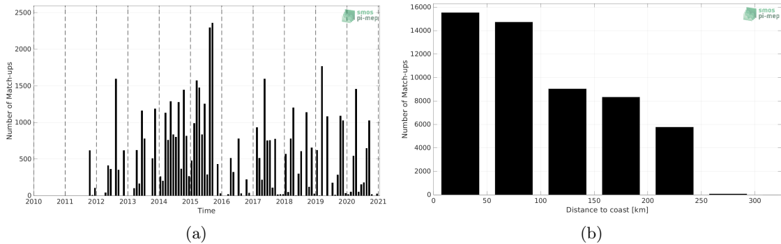
Figure 1: Number of match-ups between TSG (LEGOS-DM) and SMOS SSS L3 v8 - 18 Days (CATDS-CECOS-LOCEAN) SSS as a function of time (a) and as function of the distance to coast (b) over the Sea of Japan Pi-MEP region and for the full satellite product period.
