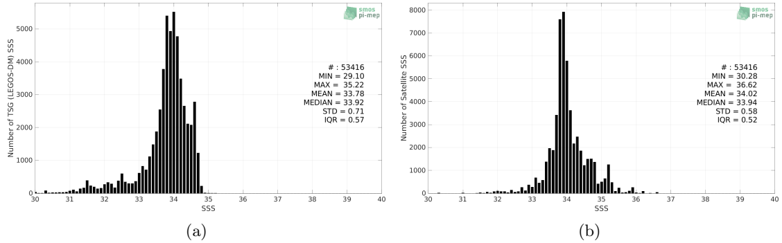
Figure 2: Histograms of SSS from TSG (LEGOS-DM) (a) and SMOS SSS L3 v8 - 18 Days (CATDS-CECOS-LOCEAN) (b) considering all match-up pairs per bins of 0.1 over the Sea of Japan Pi-MEP region and for the full satellite product period.
