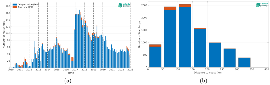
Figure 1: Number of match-ups between Argo and SMOS SSS L3 v8 - 18 Days (CATDS-CEC-LOCEAN) SSS as a function of time (a) and as function of the distance to coast (b) over the Sea of Japan Pi-MEP region and for the full satellite product period.
