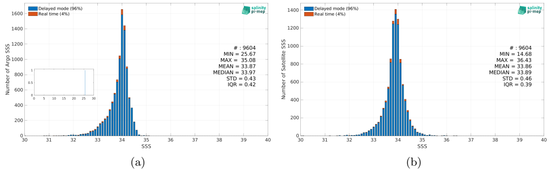
Figure 2: Histograms of SSS from Argo (a) and SMOS SSS L3 v8 - 18 Days (CATDS-CEC-LOCEAN) (b) considering all match-up pairs per bins of 0.1 over the Sea of Japan Pi-MEP region and for the full satellite product period.
