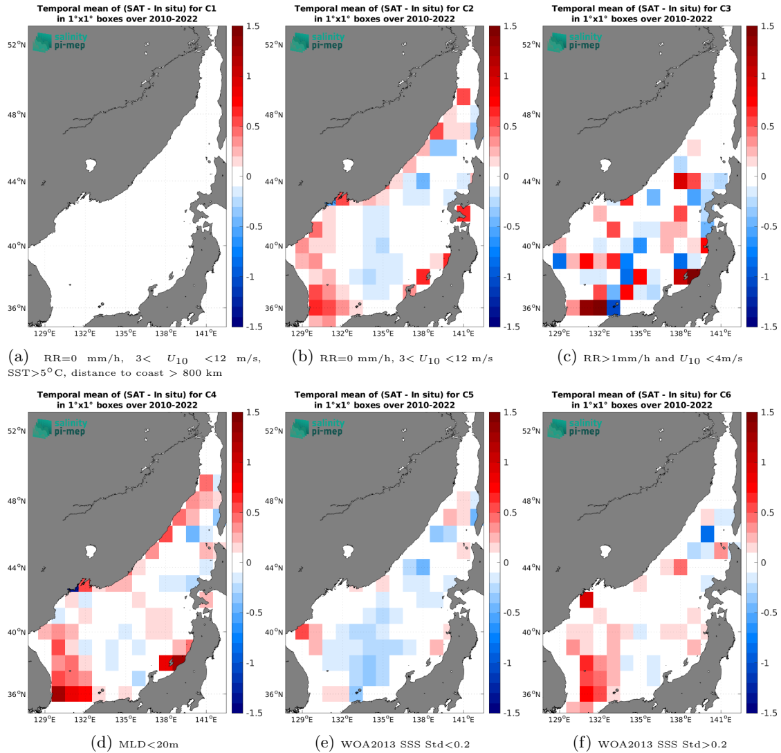
Figure 12: Temporal mean gridded over spatial boxes of size 1^\circ \times 1^\circ of \Delta SSS (SMOS SSS L3 v8 - 18 Days (CATDS-CEC-LOCEAN) - Argo) for 6 different subdatasets corresponding to: RR=0 mm/h, 3 < U_{10} < 12 m/s, SST > 5°C, distance to coast > 800 km (a), RR=0 mm/h, 3 < U_{10} < 12 m/s (b), RR > 1mm/h and U_{10} < 4 m/s (c), MLD < 20m (d), WOA2013 SSS Std < 0.2 (e), WOA2013 SSS Std > 0.2 (f).
