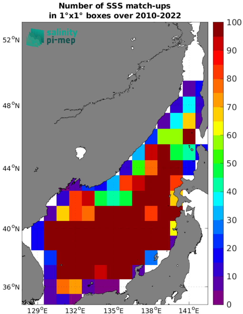
Figure 4: Number of SSS match-ups between Argo SSS and the SMOS SSS L3 v8 - 18 Days (CATDS-CEC-LOCEAN) SSS product for the Sea of Japan Pi-MEP region over 1°x1° boxes and for the full satellite product period.
