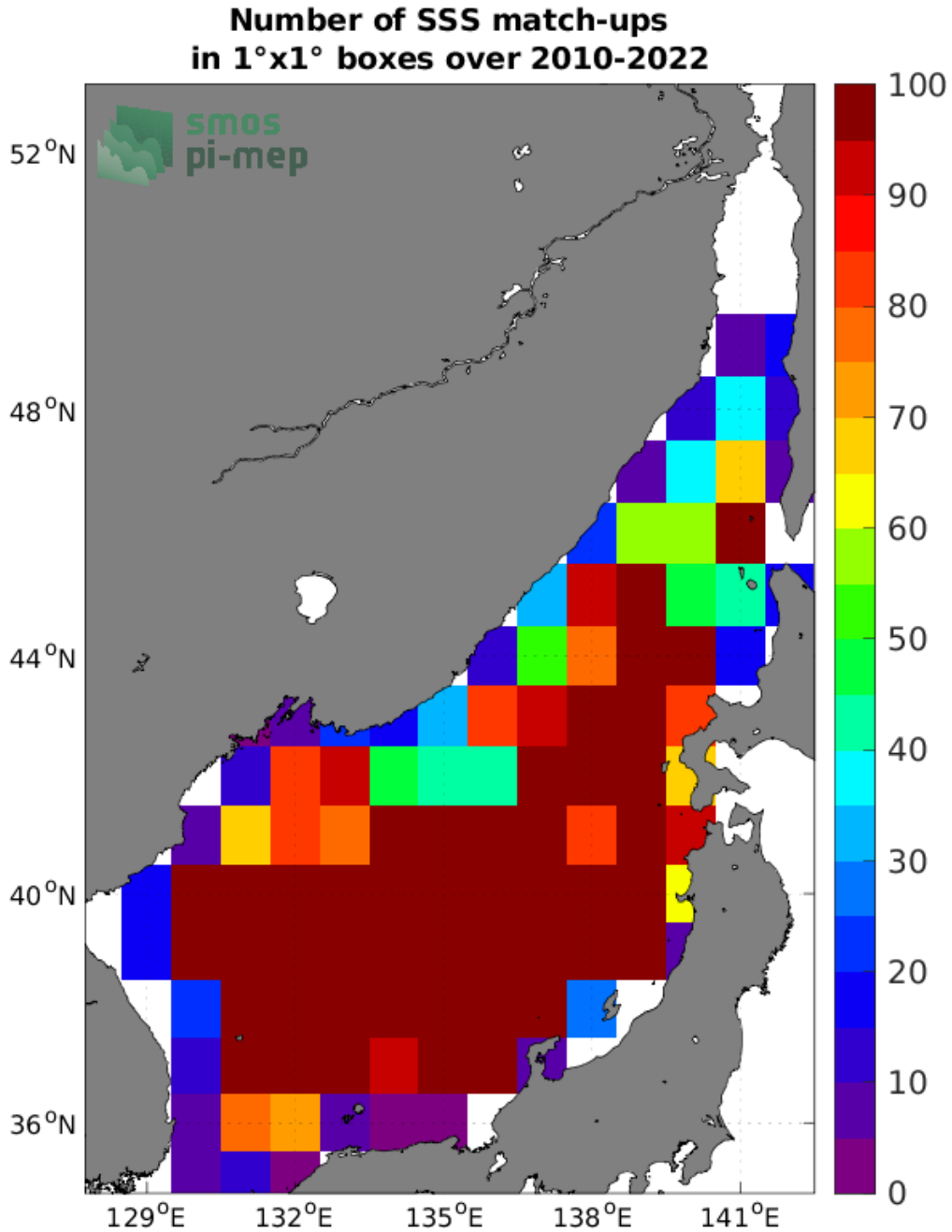
Figure 4: Number of SSS match-ups between Argo SSS and the SMOS SSS L3 v8 - 18 Days (CATDS-CECOS-LOCEAN) SSS product for the Sea of Japan Pi-MEP region over 1°×1° boxes and for the full satellite product period.
