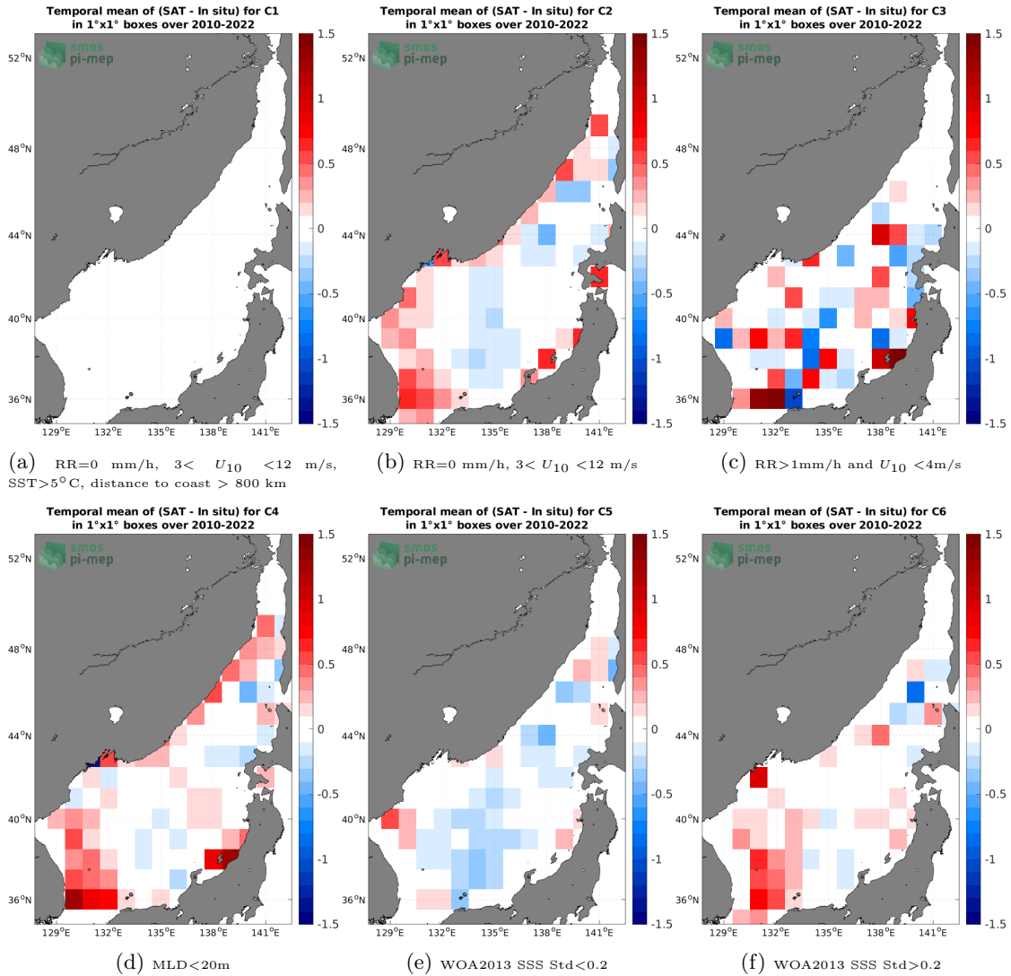
Figure 12: Temporal mean gridded over spatial boxes of size 1^\circ \times 1^\circ of \Delta\text{SSS} (SMOS SSS L3 v8 - 18 Days (CATDS-CECOS-LOCEAN) - Argo) for 6 different subdatasets corresponding to: RR=0 mm/h, 3 < U_{10} < 12 m/s, SST > 5^\circ\text{C} , distance to coast > 800 km (a), RR=0 mm/h, 3 < U_{10} < 12 m/s (b), RR > 1 mm/h and U_{10} < 4 m/s (c), MLD < 20 m (d), WOA2013 SSS Std < 0.2 (e), WOA2013 SSS Std > 0.2 (f).
