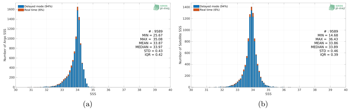
Figure 2: Histograms of SSS from Argo (a) and SMOS SSS L3 v8 - 18 Days (CATDS-CECOS-LOCEAN) (b) considering all match-up pairs per bins of 0.1 over the Sea of Japan Pi-MEP region and for the full satellite product period.
