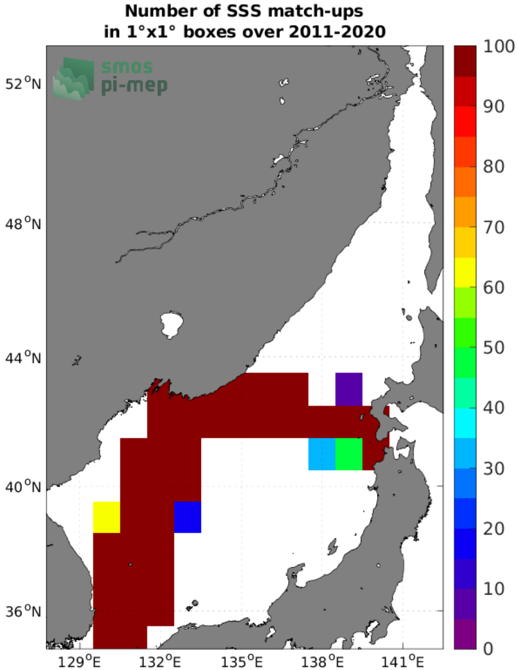
Figure 4: Number of SSS match-ups between TSG (LEGOS-DM) SSS and the SMOS SSS L3 v7 - 9 Days (CATDS-CECOS-LOCEAN) SSS product for the Sea of Japan Pi-MEP region over 1°x1° boxes and for the full satellite product period.
