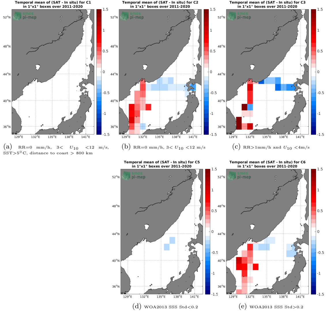
Figure 12: Temporal mean gridded over spatial boxes of size 1^\circ \times 1^\circ of \Delta SSS (SMOS SSS L3 v7 - 9 Days (CATDS-CECOS-LOCEAN) - TSG (LEGOS-DM)) for 5 different subdatasets corresponding to: RR=0 mm/h, 3 < U_{10} < 12 m/s, SST > 5^\circ\text{C} , distance to coast > 800 km (a), RR=0 mm/h, 3 < U_{10} < 12 m/s (b), RR > 1 mm/h and U_{10} < 4 m/s (c), WOA2013 SSS Std < 0.2 (d), WOA2013 SSS Std > 0.2 (e).
