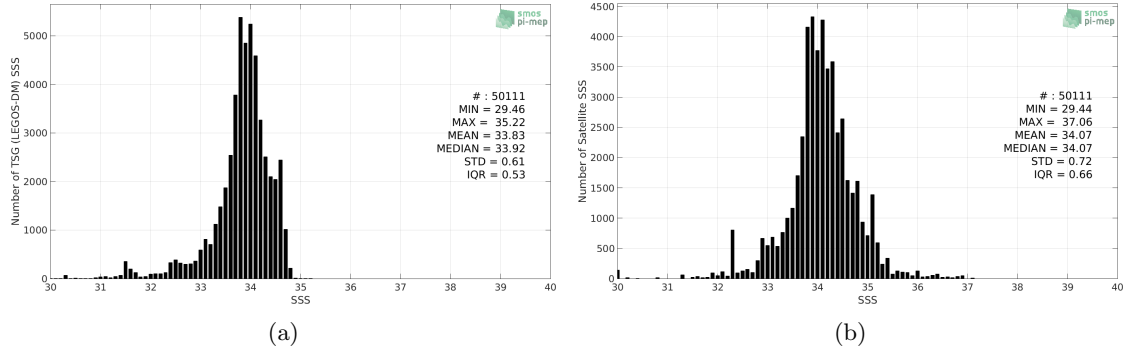
Figure 2: Histograms of SSS from TSG (LEGOS-DM) (a) and SMOS SSS L3 v7 - 9 Days (CATDS-CECOS-LOCEAN) (b) considering all match-up pairs per bins of 0.1 over the Sea of Japan Pi-MEP region and for the full satellite product period.
