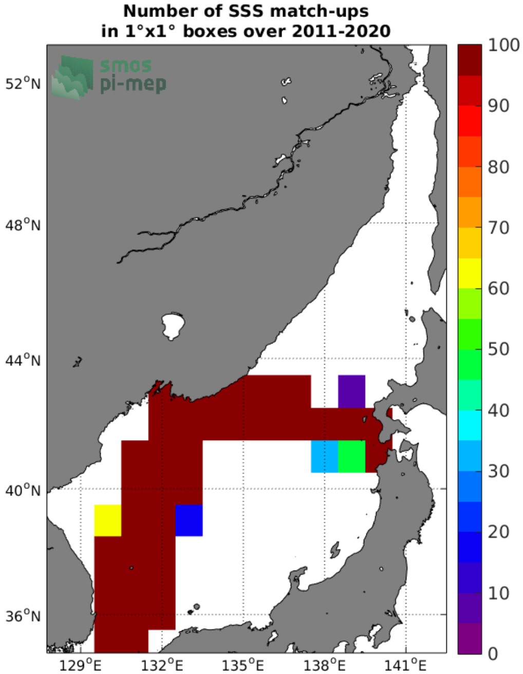
Figure 4: Number of SSS match-ups between TSG (LEGOS-DM) SSS and the SMOS SSS L3 v7 - 9 Days (CATDS-CECOS-LOCEAN) SSS product for the Sea of Japan Pi-MEP region over 1^\circ \times 1^\circ boxes and for the full satellite product period.
