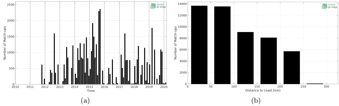
Figure 1: Number of match-ups between TSG (LEGOS-DM) and SMOS SSS L3 v7 - 9 Days (CATDS-CECOS-LOCEAN) SSS as a function of time (a) and as function of the distance to coast (b) over the Sea of Japan Pi-MEP region and for the full satellite product period.
