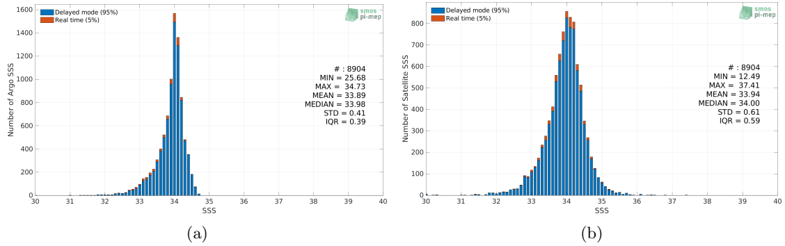
Figure 2: Histograms of SSS from Argo (a) and SMOS SSS L3 v7 - 9 Days (CATDS-CECOS-LOCEAN) (b) considering all match-up pairs per bins of 0.1 over the Sea of Japan Pi-MEP region and for the full satellite product period.
