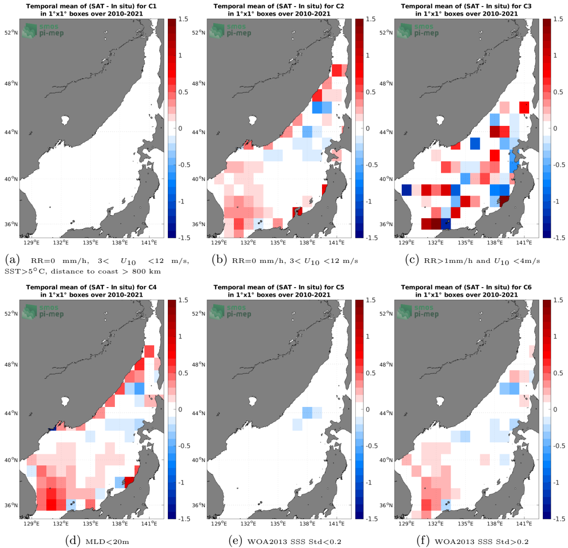
Figure 12: Temporal mean gridded over spatial boxes of size 1^\circ \times 1^\circ of \Delta SSS (SMOS SSS L3 v7 - 9 Days (CATDS-CECOS-LOCEAN) - Argo) for 6 different subdatasets corresponding to: RR=0 mm/h, 3 < U_{10} < 12 m/s, SST > 5^\circ\text{C} , distance to coast > 800 km (a), RR=0 mm/h, 3 < U_{10} < 12 m/s (b), RR > 1 mm/h and U_{10} < 4 m/s (c), MLD < 20 m (d), WOA2013 SSS Std < 0.2 (e), WOA2013 SSS Std > 0.2 (f).
