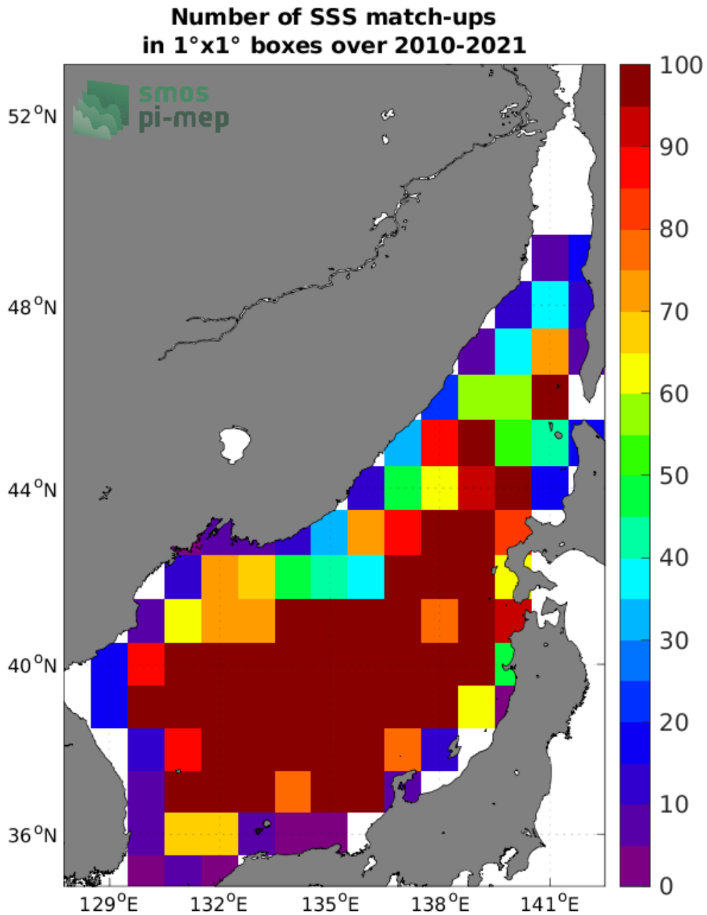
Figure 4: Number of SSS match-ups between Argo SSS and the SMOS SSS L3 v7 - 9 Days (CATDS-CECOS-LOCEAN) SSS product for the Sea of Japan Pi-MEP region over 1°×1° boxes and for the full satellite product period.
