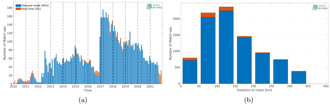
Figure 1: Number of match-ups between Argo and SMOS SSS L3 v7 - 9 Days (CATDS-CECOS-LOCEAN) SSS as a function of time (a) and as function of the distance to coast (b) over the Sea of Japan Pi-MEP region and for the full satellite product period.
