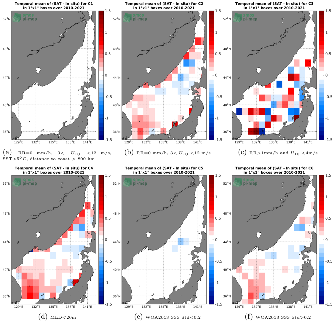
Figure 12: Temporal mean gridded over spatial boxes of size 1^\circ \times 1^\circ of \Delta\text{SSS} (SMOS SSS L3 v7 - 9 Days (CATDS-CECOS-LOCEAN) - Argo) for 6 different subdatasets corresponding to: RR=0 mm/h, 3 < U_{10} < 12 m/s, SST > 5^\circ\text{C} , distance to coast > 800 km (a), RR=0 mm/h, 3 < U_{10} < 12 m/s (b), RR > 1 mm/h and U_{10} < 4 m/s (c), MLD < 20 m (d), WOA2013 SSS Std < 0.2 (e), WOA2013 SSS Std > 0.2 (f).
