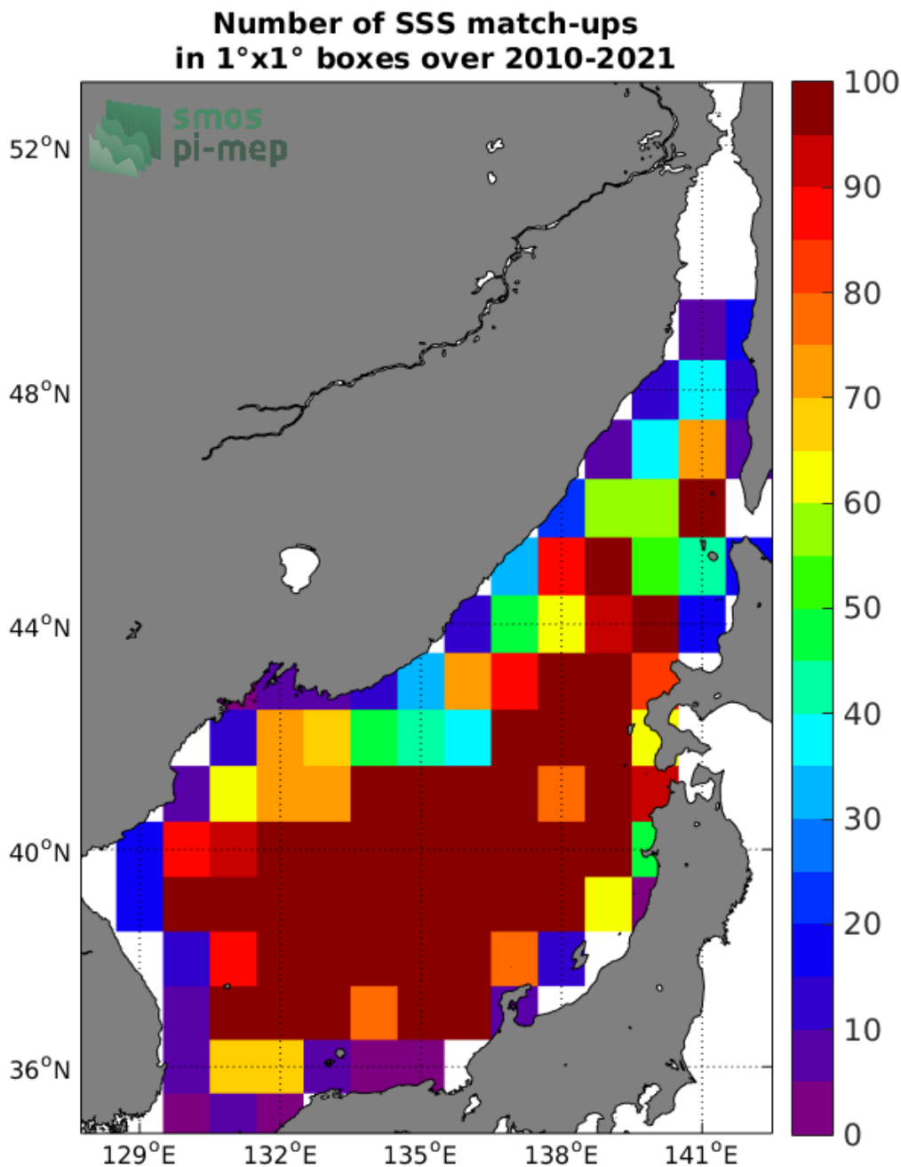
Figure 4: Number of SSS match-ups between Argo SSS and the SMOS SSS L3 v7 - 9 Days (CATDS-CECOS-LOCEAN) SSS product for the Sea of Japan Pi-MEP region over 1°x1° boxes and for the full satellite product period.
