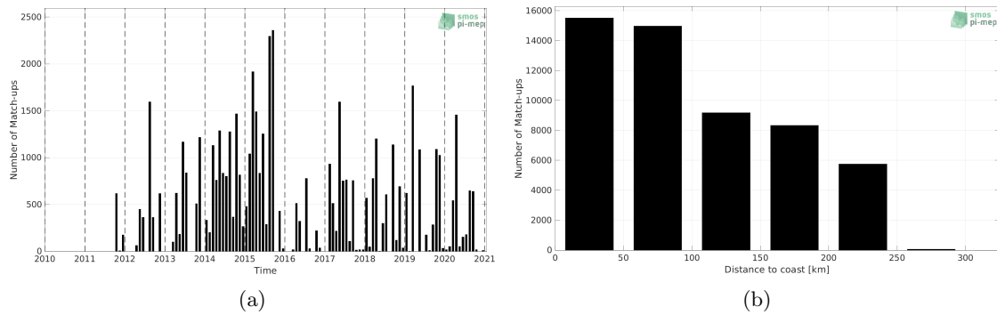
Figure 1: Number of match-ups between TSG (LEGOS-DM) and SMOS SSS L3 v7 - 18 Days (CATDS-CECOS-LOCEAN) SSS as a function of time (a) and as function of the distance to coast (b) over the Sea of Japan Pi-MEP region and for the full satellite product period.
