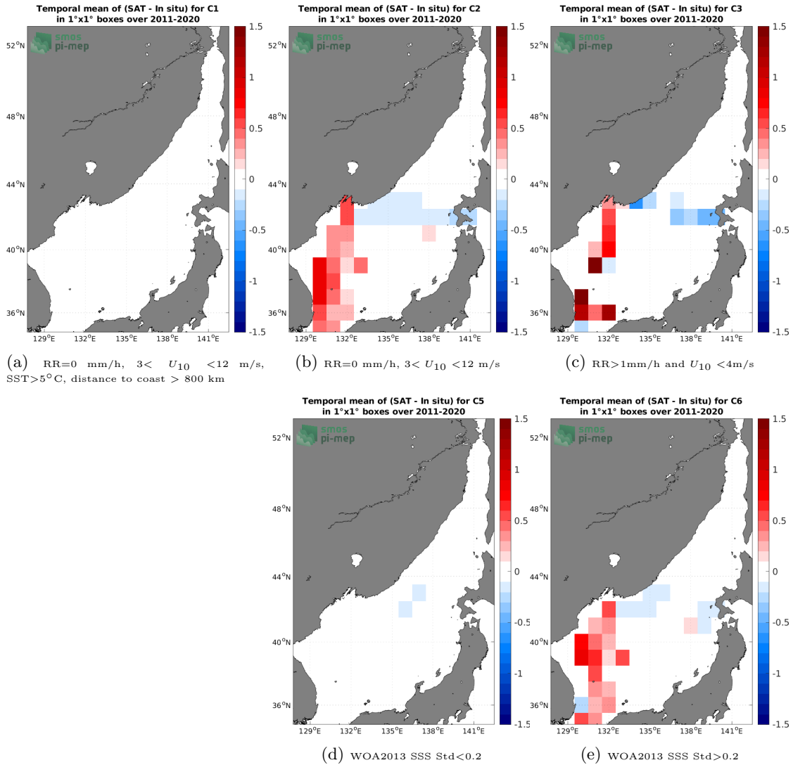
Figure 12: Temporal mean gridded over spatial boxes of size 1^\circ \times 1^\circ of \Delta SSS (SMOS SSS L3 v7 - 18 Days (CATDS-CECOS-LOCEAN) - TSG (LEGOS-DM)) for 5 different subdatasets corresponding to:RR=0 mm/h, 3 < U_{10} < 12 m/s, SST>5°C, distance to coast > 800 km (a), RR=0 mm/h, 3 < U_{10} < 12 m/s (b), RR>1mm/h and U_{10} < 4 m/s (c), WOA2013 SSS Std<0.2 (d), WOA2013 SSS Std>0.2 (e).
