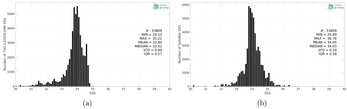
Figure 2: Histograms of SSS from TSG (LEGOS-DM) (a) and SMOS SSS L3 v7 - 18 Days (CATDS-CECOS-LOCEAN) (b) considering all match-up pairs per bins of 0.1 over the Sea of Japan Pi-MEP region and for the full satellite product period.
