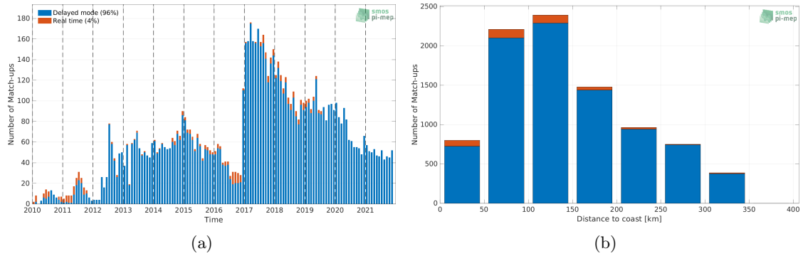
Figure 1: Number of match-ups between Argo and SMOS SSS L3 v7 - 18 Days (CATDS-CECOS-LOCEAN) SSS as a function of time (a) and as function of the distance to coast (b) over the Sea of Japan Pi-MEP region and for the full satellite product period.
