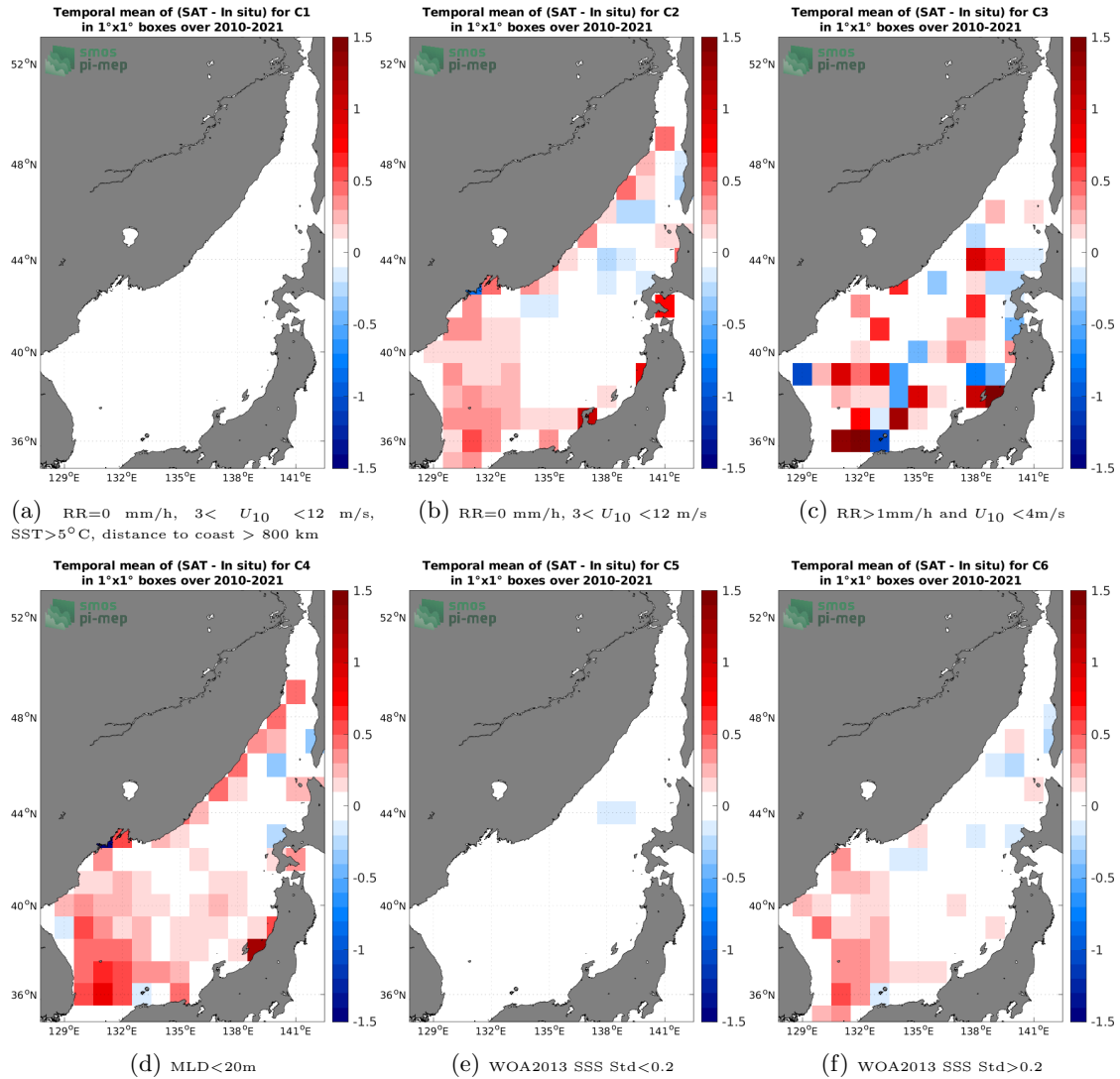
Figure 12: Temporal mean gridded over spatial boxes of size 1^\circ \times 1^\circ of \Delta SSS (SMOS SSS L3 v7 - 18 Days (CATDS-CECOS-LOCEAN) - Argo) for 6 different subdatasets corresponding to: RR=0 mm/h, 3 < U_{10} < 12 m/s, SST > 5^\circ\text{C} , distance to coast > 800 km (a), RR=0 mm/h, 3 < U_{10} < 12 m/s (b), RR > 1 mm/h and U_{10} < 4 m/s (c), MLD < 20 m (d), WOA2013 SSS Std < 0.2 (e), WOA2013 SSS Std > 0.2 (f).
