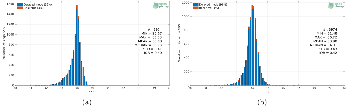
Figure 2: Histograms of SSS from Argo (a) and SMOS SSS L3 v7 - 18 Days (CATDS-CECOS-LOCEAN) (b) considering all match-up pairs per bins of 0.1 over the Sea of Japan Pi-MEP region and for the full satellite product period.
