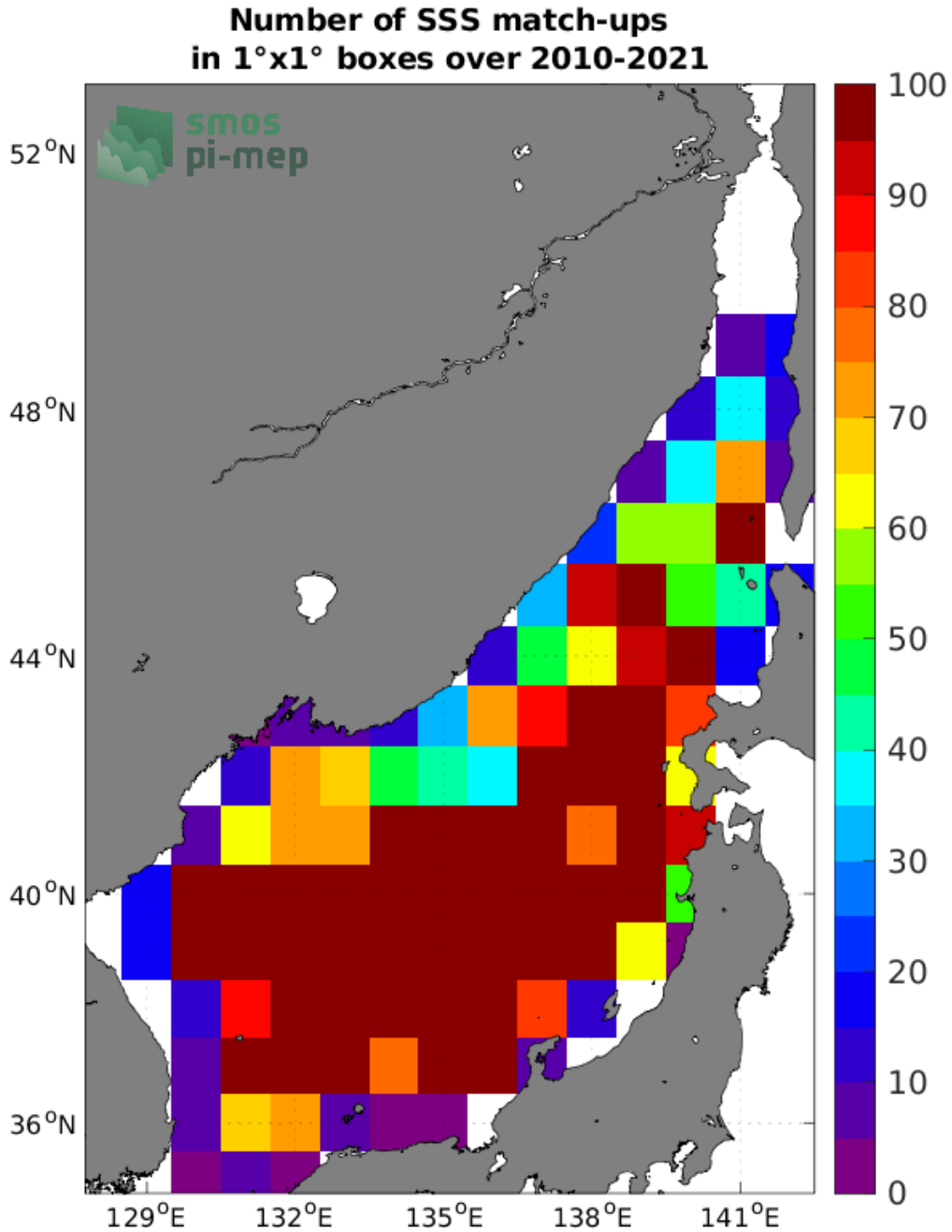
Figure 4: Number of SSS match-ups between Argo SSS and the SMOS SSS L3 v7 - 18 Days (CATDS-CECOS-LOCEAN) SSS product for the Sea of Japan Pi-MEP region over 1°x1° boxes and for the full satellite product period.
