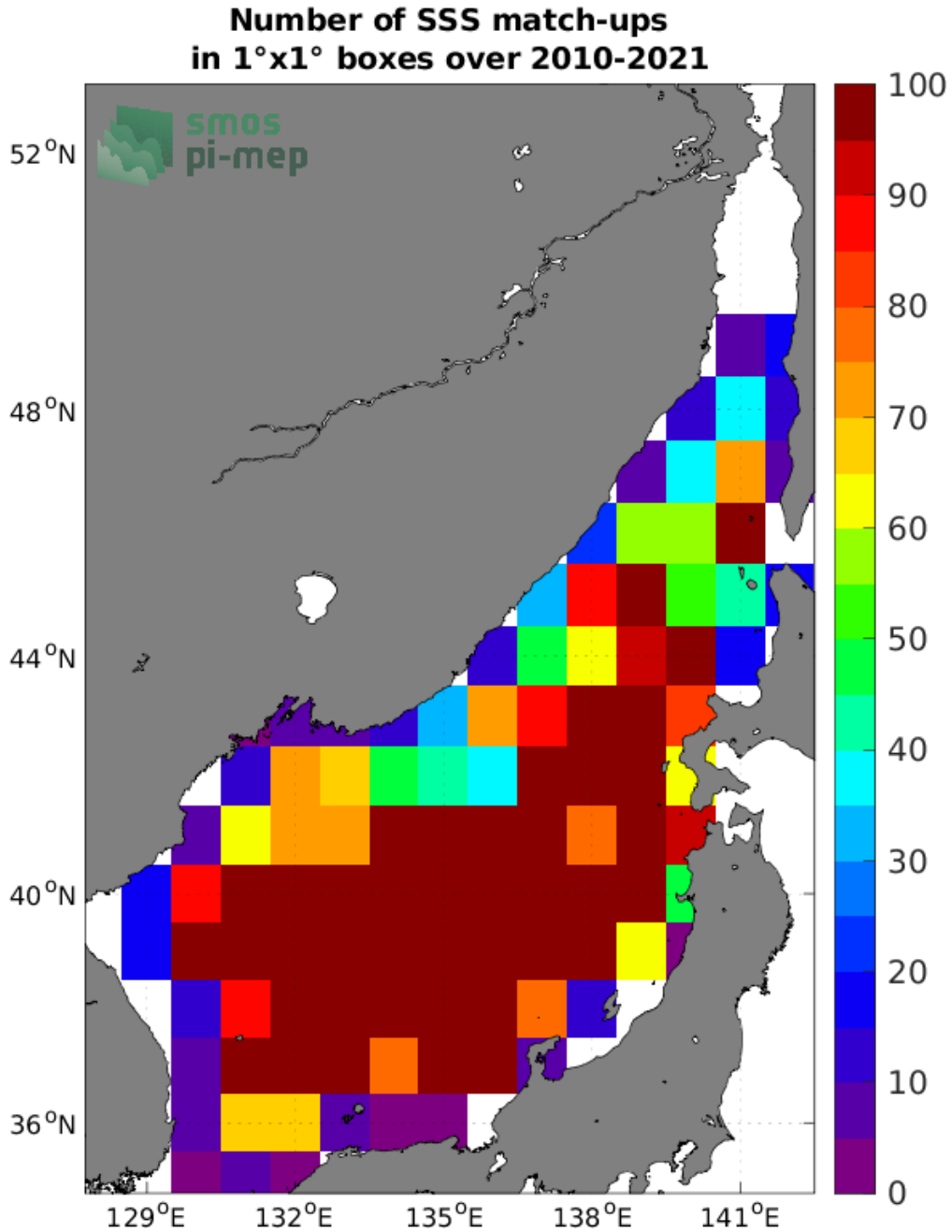
Figure 4: Number of SSS match-ups between Argo SSS and the SMOS SSS L3 v7 - 18 Days (CATDS-CECOS-LOCEAN) SSS product for the Sea of Japan Pi-MEP region over 1°×1° boxes and for the full satellite product period.
