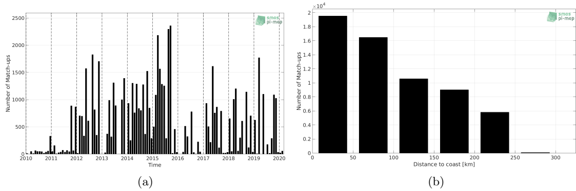
Figure 1: Number of match-ups between TSG (LEGOS-DM) and SMOS SSS L3 v5 - 9 Days (CATDS-CECOS-LOCEAN) SSS as a function of time (a) and as function of the distance to coast (b) over the Sea of Japan Pi-MEP region and for the full satellite product period.
