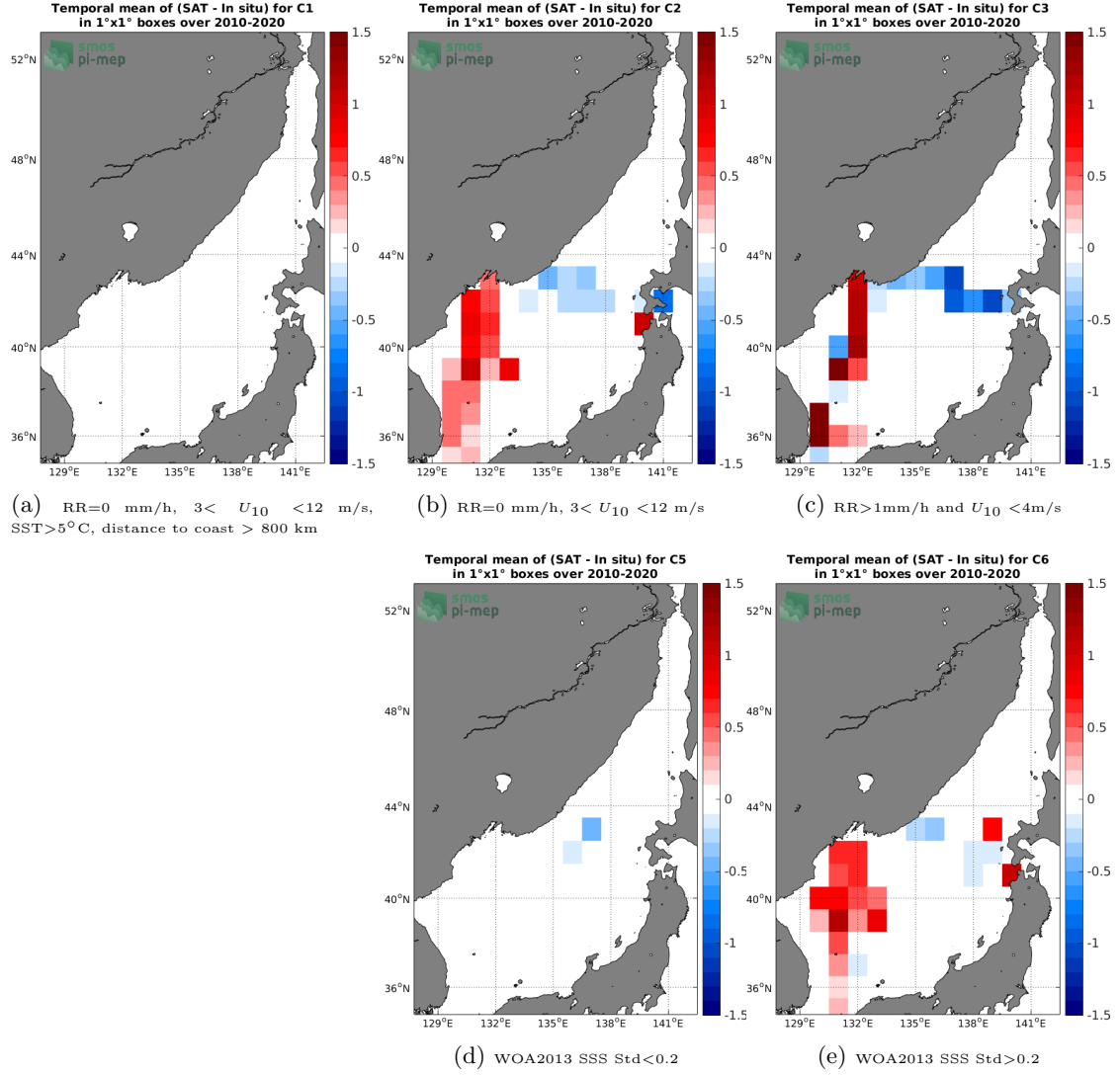
Figure 12: Temporal mean gridded over spatial boxes of size 1^\circ \times 1^\circ of \Delta\text{SSS} (SMOS SSS L3 v5 - 9 Days (CATDS-CECOS-LOCEAN) - TSG (LEGOS-DM)) for 5 different subdatasets corresponding to: RR=0 mm/h, 3 < U_{10} < 12 m/s, SST > 5^\circ\text{C} , distance to coast > 800 km (a), RR=0 mm/h, 3 < U_{10} < 12 m/s (b), RR > 1 mm/h and U_{10} < 4 m/s (c), WOA2013 SSS Std < 0.2 (d), WOA2013 SSS Std > 0.2 (e).
