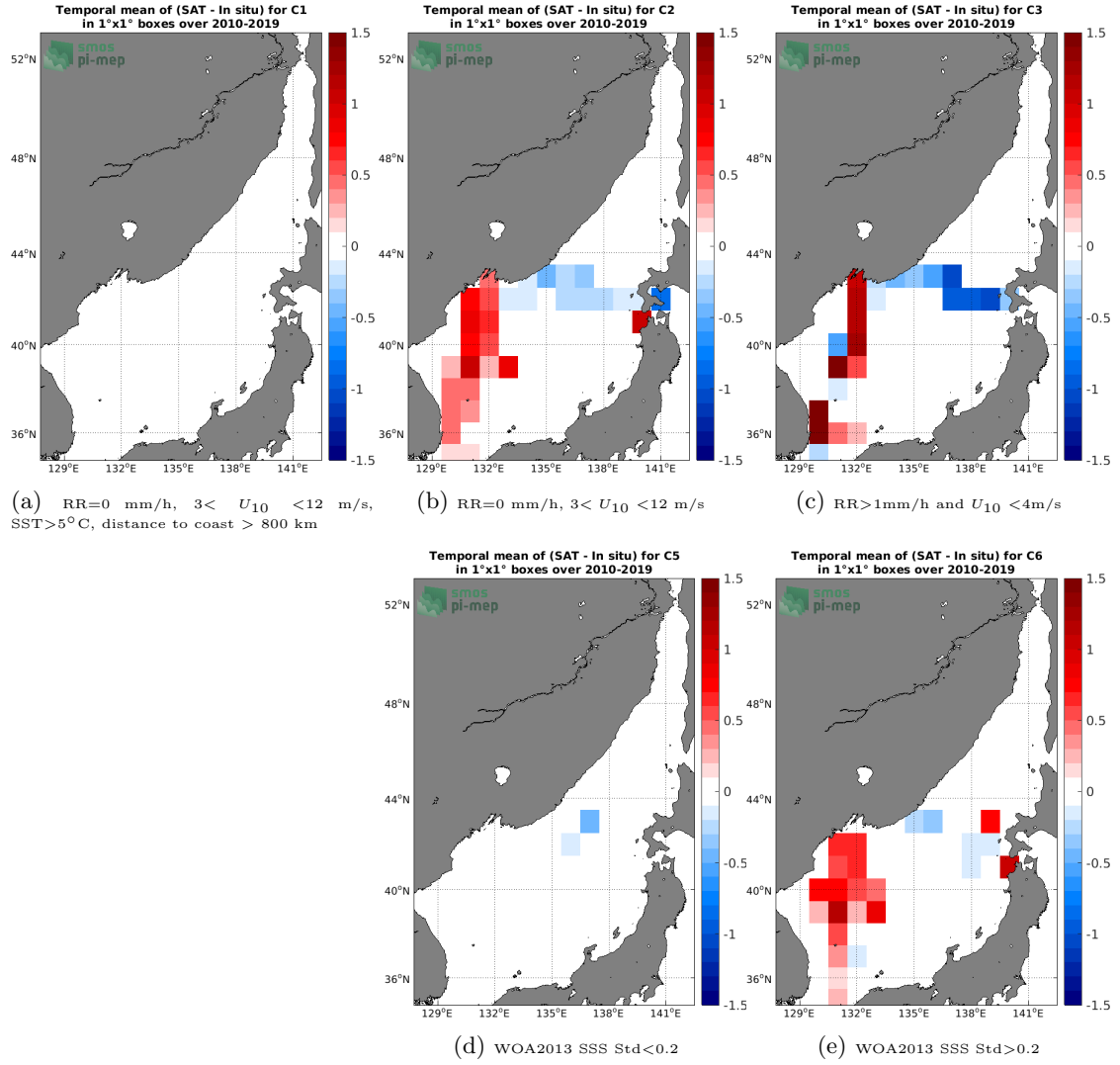
Figure 12: Temporal mean gridded over spatial boxes of size 1^\circ \times 1^\circ of \Delta SSS (SMOS SSS L3 v5 - 9 Days (CATDS-CECOS-LOCEAN) - TSG (LEGOS-DM)) for 5 different subdatasets corresponding to: RR=0 mm/h, 3 < U_{10} < 12 m/s, SST>5°C, distance to coast > 800 km (a), RR=0 mm/h, 3 < U_{10} < 12 m/s (b), RR>1mm/h and U_{10} < 4 m/s (c), WOA2013 SSS Std<0.2 (d), WOA2013 SSS Std>0.2 (e).
