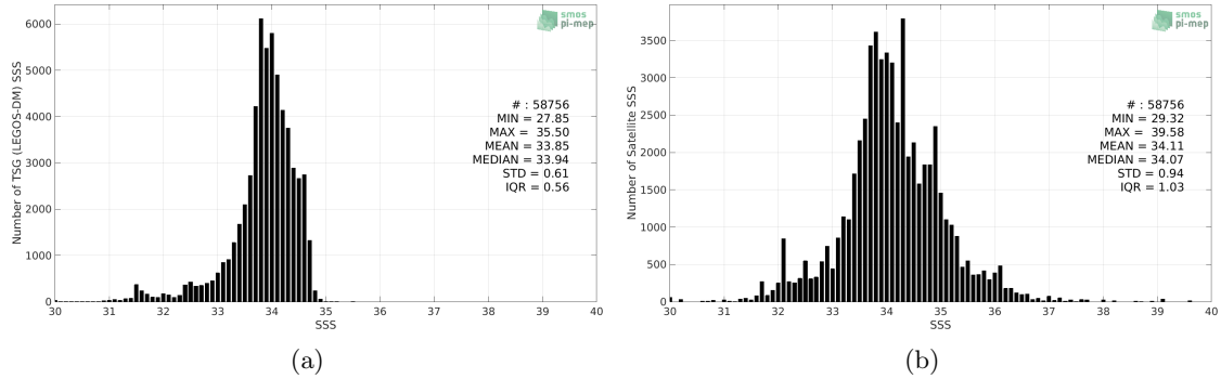
Figure 2: Histograms of SSS from TSG (LEGOS-DM) (a) and SMOS SSS L3 v5 - 9 Days (CATDS-CECOS-LOCEAN) (b) considering all match-up pairs per bins of 0.1 over the Sea of Japan Pi-MEP region and for the full satellite product period.
