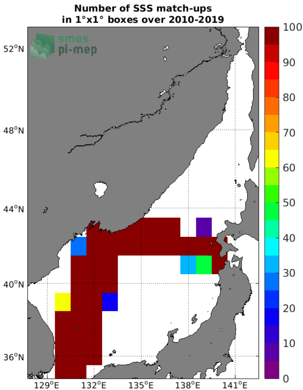
Figure 4: Number of SSS match-ups between TSG (LEGOS-DM) SSS and the SMOS SSS L3 v5 - 9 Days (CATDS-CECOS-LOCEAN) SSS product for the Sea of Japan Pi-MEP region over 1°x1° boxes and for the full satellite product period.
