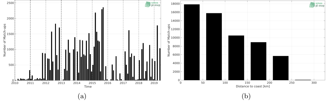
Figure 1: Number of match-ups between TSG (LEGOS-DM) and SMOS SSS L3 v5 - 9 Days (CATDS-CECOS-LOCEAN) SSS as a function of time (a) and as function of the distance to coast (b) over the Sea of Japan Pi-MEP region and for the full satellite product period.
