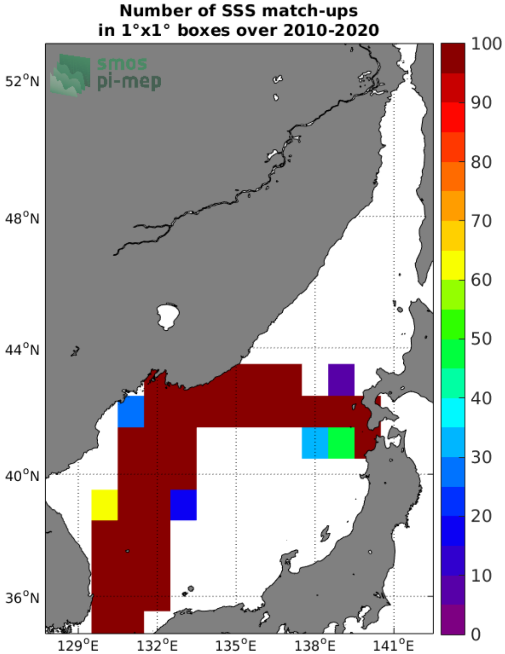
Figure 4: Number of SSS match-ups between TSG (LEGOS-DM) SSS and the SMOS SSS L3 v5 - 18 Days (CATDS-CECOS-LOCEAN) SSS product for the Sea of Japan Pi-MEP region over 1^\circ \times 1^\circ boxes and for the full satellite product period.
