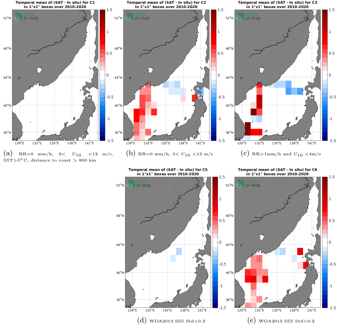
Figure 12: Temporal mean gridded over spatial boxes of size 1^\circ \times 1^\circ of \Delta\text{SSS} (SMOS SSS L3 v5 - 18 Days (CATDS-CECOS-LOCEAN) - TSG (LEGOS-DM)) for 5 different subdatasets corresponding to: RR=0 mm/h, 3 < U_{10} < 12 m/s, SST > 5^\circ\text{C} , distance to coast > 800 km (a), RR=0 mm/h, 3 < U_{10} < 12 m/s (b), RR > 1 mm/h and U_{10} < 4 m/s (c), WOA2013 SSS Std < 0.2 (d), WOA2013 SSS Std > 0.2 (e).
