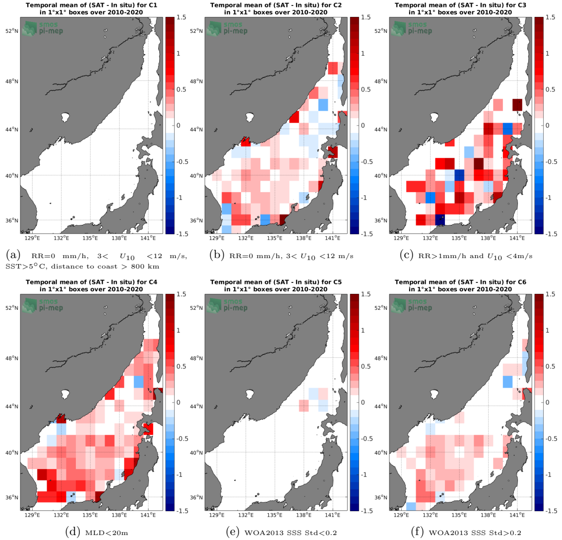
Figure 12: Temporal mean gridded over spatial boxes of size 1^\circ \times 1^\circ of \Delta SSS (SMOS SSS L3 v5 - 18 Days (CATDS-CECOS-LOCEAN) - Argo) for 6 different subdatasets corresponding to:RR=0 mm/h, 3 < U_{10} < 12 m/s, SST>5°C, distance to coast > 800 km (a), RR=0 mm/h, 3 < U_{10} < 12 m/s (b), RR>1mm/h and U_{10} < 4 m/s (c),MLD<20m (d),WOA2013 SSS Std<0.2 (e),WOA2013 SSS Std>0.2 (f).
