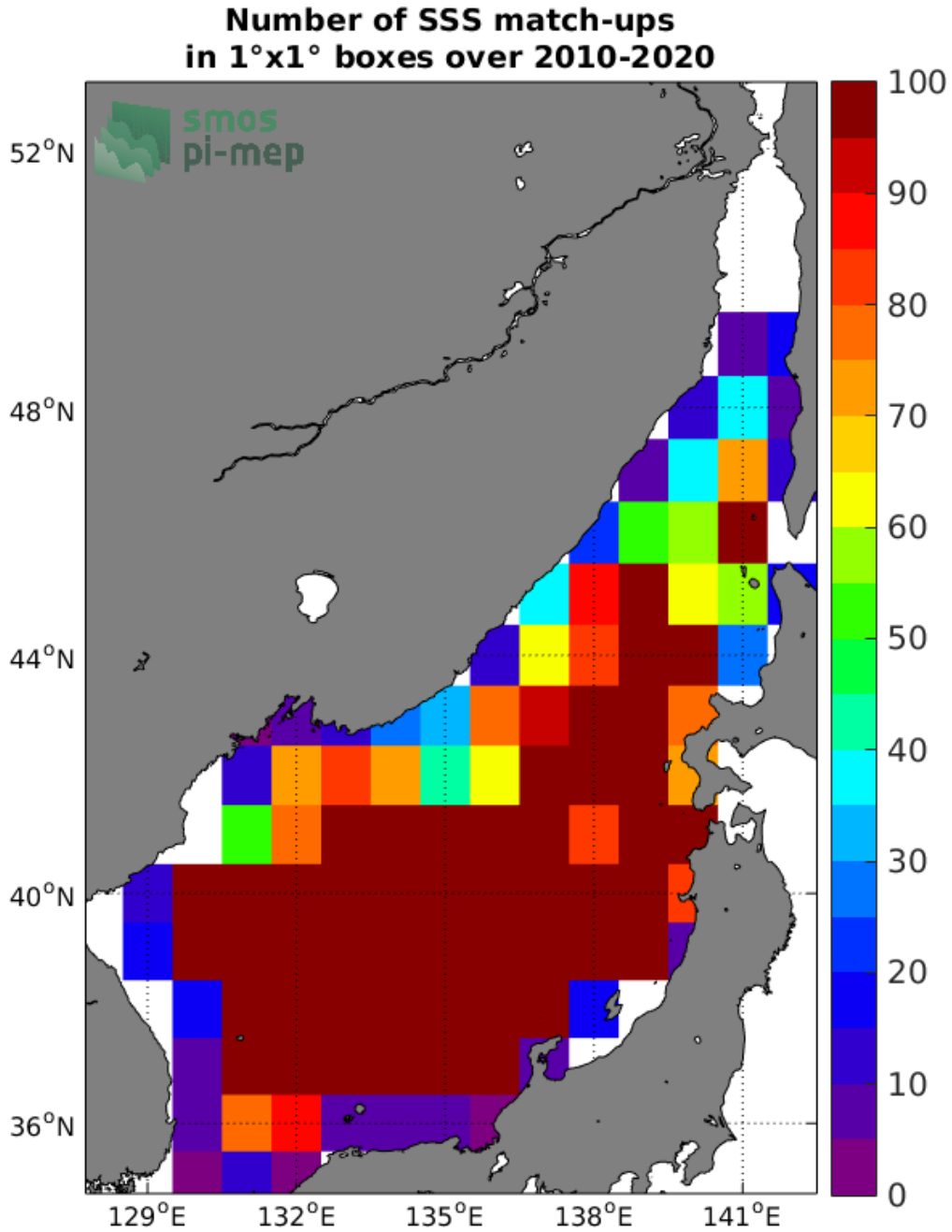
Figure 4: Number of SSS match-ups between Argo SSS and the SMOS SSS L3 v5 - 18 Days (CATDS-CECOS-LOCEAN) SSS product for the Sea of Japan Pi-MEP region over 1°×1° boxes and for the full satellite product period.
