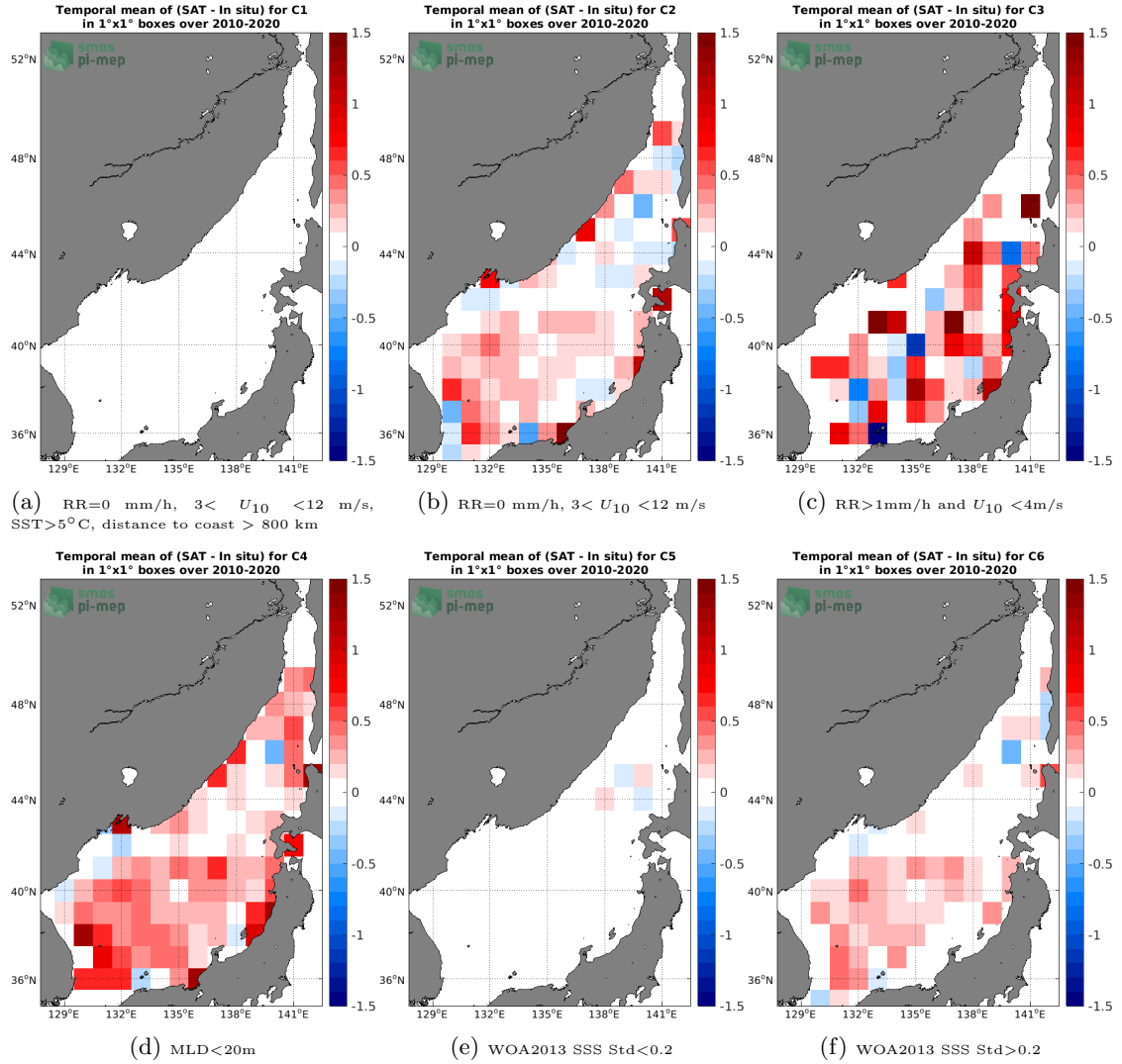
Figure 12: Temporal mean gridded over spatial boxes of size 1°x1° of \Delta\text{SSS} (SMOS SSS L3 v5 - 18 Days (CATDS-CECOS-LOCEAN) - Argo) for 6 different subdatasets corresponding to: RR=0 mm/h, 3 < U_{10} < 12 m/s, SST > 5^\circ\text{C} , distance to coast > 800 km (a), RR=0 mm/h, 3 < U_{10} < 12 m/s (b), RR > 1 mm/h and U_{10} < 4 m/s (c), MLD < 20\text{m} (d), WOA2013 SSS Std < 0.2 (e), WOA2013 SSS Std > 0.2 (f).
