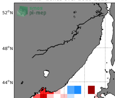
Temporal mean of (Sat - TSG-LEGOS-DM) in 1°x1° boxes over 2010-2018
