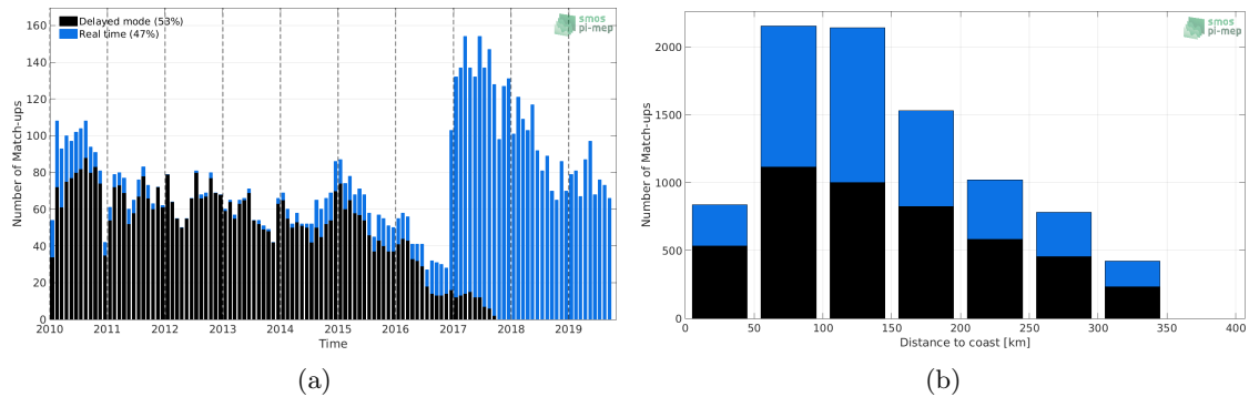
Figure 1: Number of match-ups between Argo and SMOS-L3-CATDS-CECOS-LOCEAN-V4-9DAYS-25KM SSS as a function of time (a) and as function of the distance to coast (b) over the Sea of Japan Pi-MEP region and for the full satellite product period.
