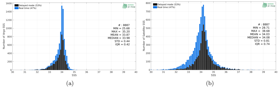
Figure 2: Histograms of SSS from Argo (a) and SMOS-L3-CATDS-CECOS-LOCEAN-V4-9DAYS-25KM (b) considering all match-up pairs per bins of 0.1 over the Sea of Japan Pi-MEP region and for the full satellite product period.
