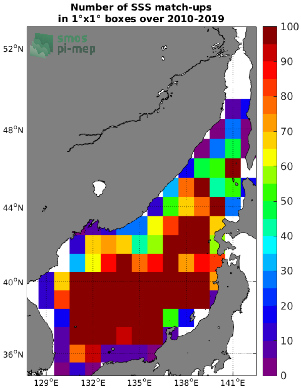
Figure 4: Number of SSS match-ups between Argo SSS and the SMOS-L3-CATDS-CECOS-LOCEAN-V4-9DAYS-25KM SSS product for the Sea of Japan Pi-MEP region over 1°x1° boxes and for the full satellite product period.
