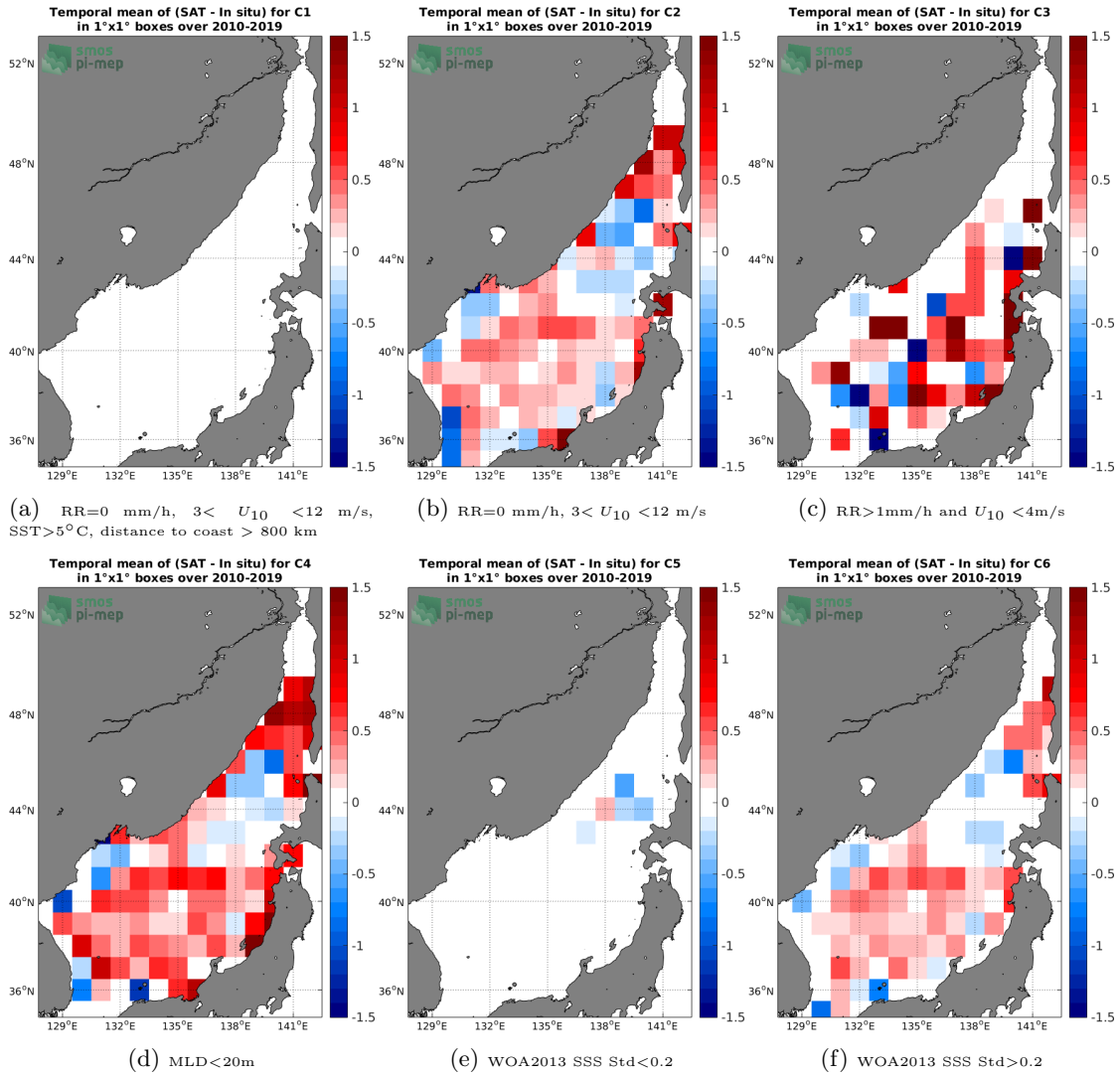
Figure 12: Temporal mean gridded over spatial boxes of size 1°x1° of \Delta SSS (SMOS-L3-CATDS-CECOS-LOCEAN-V4-9DAYS-25KM - Argo) for 6 different subdatasets corresponding to: RR=0 mm/h, 3 < U_{10} < 12 m/s, SST > 5°C, distance to coast > 800 km (a), RR=0 mm/h, 3 < U_{10} < 12 m/s (b), RR > 1mm/h and U_{10} < 4 m/s (c), MLD < 20m (d), WOA2013 SSS Std < 0.2 (e), WOA2013 SSS Std > 0.2 (f).
