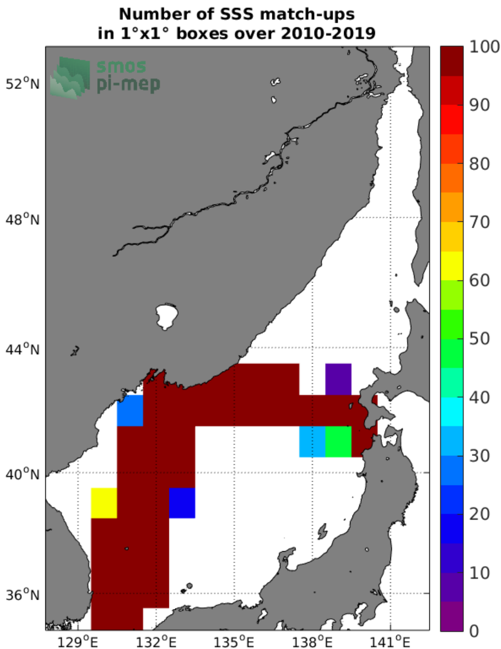
Figure 4: Number of SSS match-ups between TSG (LEGOS-DM) SSS and the SMOS SSS L3 v4 - 18 Days (CATDS-CECOS-LOCEAN) SSS product for the Sea of Japan Pi-MEP region over 1°x1° boxes and for the full satellite product period.
