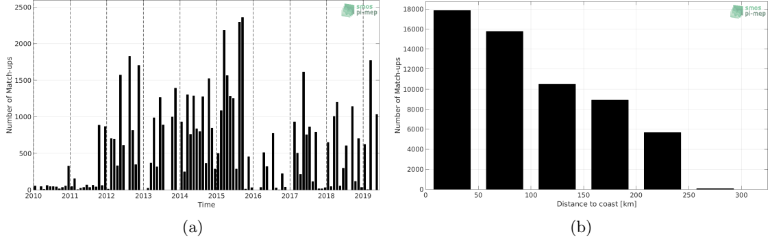
Figure 1: Number of match-ups between TSG (LEGOS-DM) and SMOS SSS L3 v4 - 18 Days (CATDS-CECOS-LOCEAN) SSS as a function of time (a) and as function of the distance to coast (b) over the Sea of Japan Pi-MEP region and for the full satellite product period.
