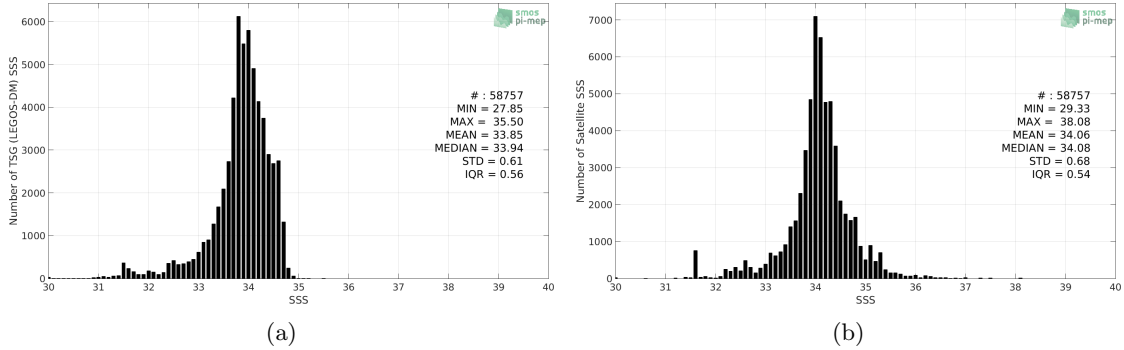
Figure 2: Histograms of SSS from TSG (LEGOS-DM) (a) and SMOS SSS L3 v4 - 18 Days (CATDS-CECOS-LOCEAN) (b) considering all match-up pairs per bins of 0.1 over the Sea of Japan Pi-MEP region and for the full satellite product period.
