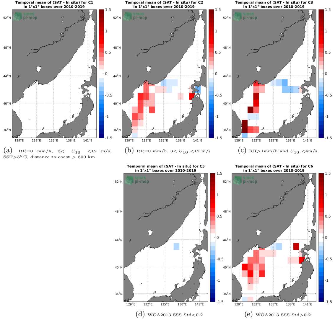
Figure 12: Temporal mean gridded over spatial boxes of size 1°x1° of \Delta\text{SSS} (SMOS SSS L3 v4 - 18 Days (CATDS-CECOS-LOCEAN) - TSG (LEGOS-DM)) for 5 different subdatasets corresponding to: RR=0 mm/h, 3 < U_{10} < 12 m/s, SST > 5^\circ\text{C} , distance to coast > 800 km (a), RR=0 mm/h, 3 < U_{10} < 12 m/s (b), RR > 1 mm/h and U_{10} < 4 m/s (c), WOA2013 SSS Std < 0.2 (d), WOA2013 SSS Std > 0.2 (e).
