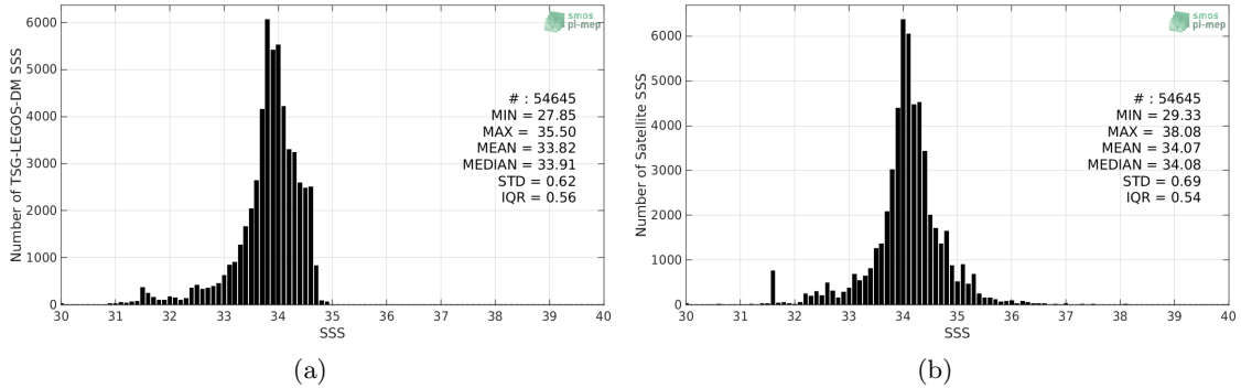
Figure 2: Histograms of SSS from TSG-LEGOS-DM (a) and SMOS-L3-CATDS-CECOS-LOCEAN-V4-18DAYS-25KM (b) considering all match-up pairs per bins of 0.1 over the Sea of Japan Pi-MEP region and for the full satellite product period.
