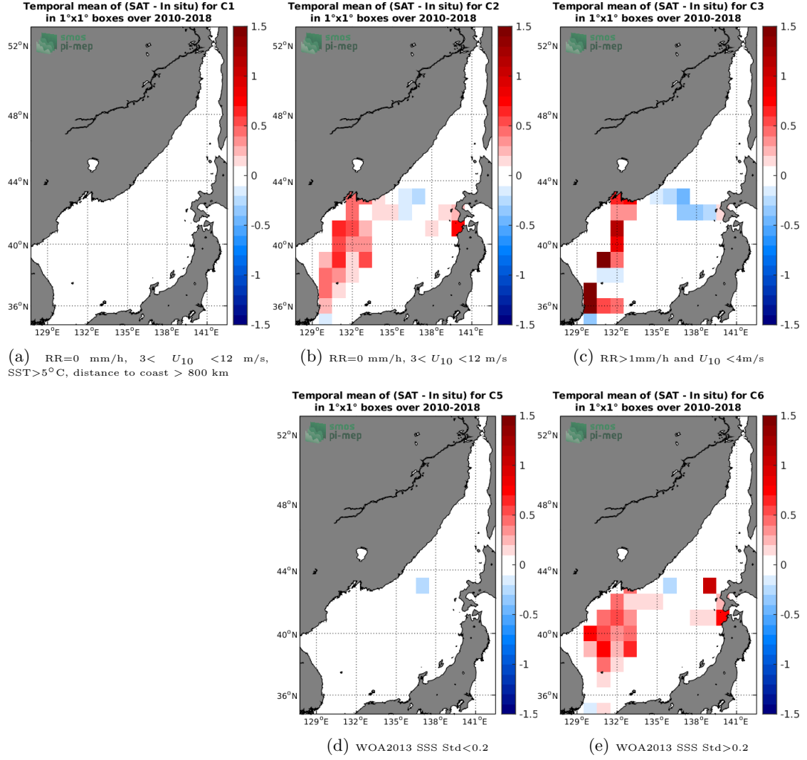
Figure 12: Temporal mean gridded over spatial boxes of size 1°x1° of \Delta\text{SSS} (SMOS-L3-CATDS-CECOS-LOCEAN-V4-18DAYS-25KM - TSG-LEGOS-DM) for 5 different subdatasets corresponding to: RR=0 mm/h, 3 < U_{10} < 12 m/s, SST > 5^\circ\text{C} , distance to coast > 800 km (a), RR=0 mm/h, 3 < U_{10} < 12 m/s (b), RR > 1\text{mm/h} and U_{10} < 4\text{m/s} (c), WOA2013 SSS Std < 0.2 (d), WOA2013 SSS Std > 0.2 (e).
