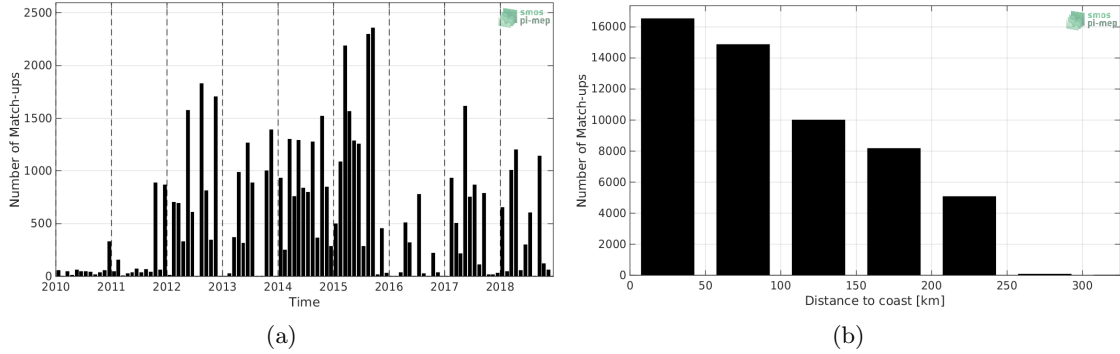
Figure 1: Number of match-ups between TSG-LEGOS-DM and SMOS-L3-CATDS-CECOS-LOCEAN-V4-18DAYS-25KM SSS as a function of time (a) and as function of the distance to coast (b) over the Sea of Japan Pi-MEP region and for the full satellite product period.
