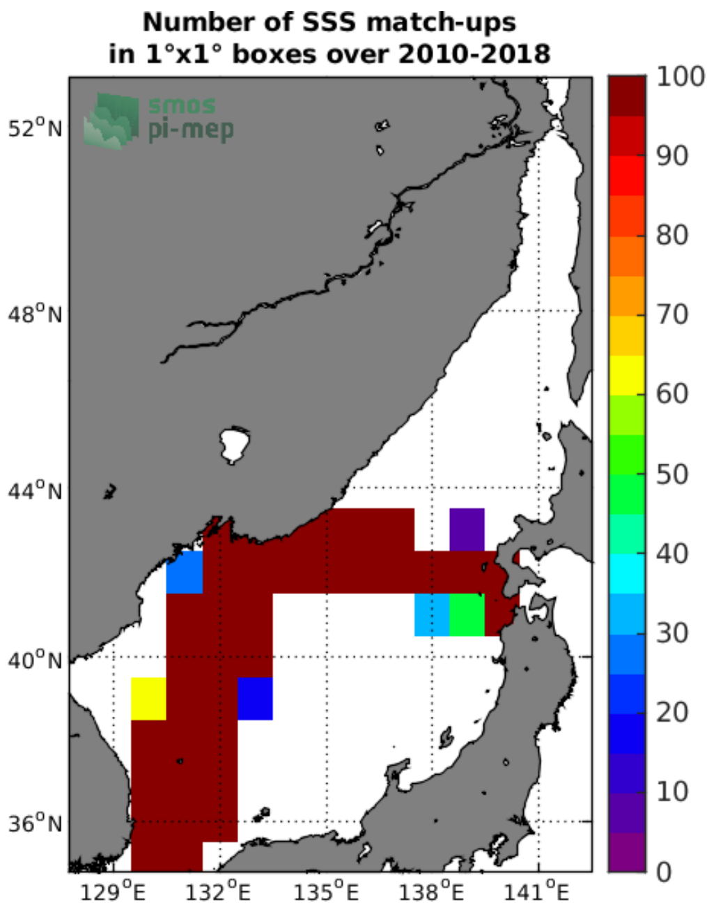
Figure 4: Number of SSS match-ups between TSG-LEGOS-DM SSS and the SMOS-L3-CATDS-CECOS-LOCEAN-V4-18DAYS-25KM SSS product for the Sea of Japan Pi-MEP region over 1°x1° boxes and for the full satellite product period.
