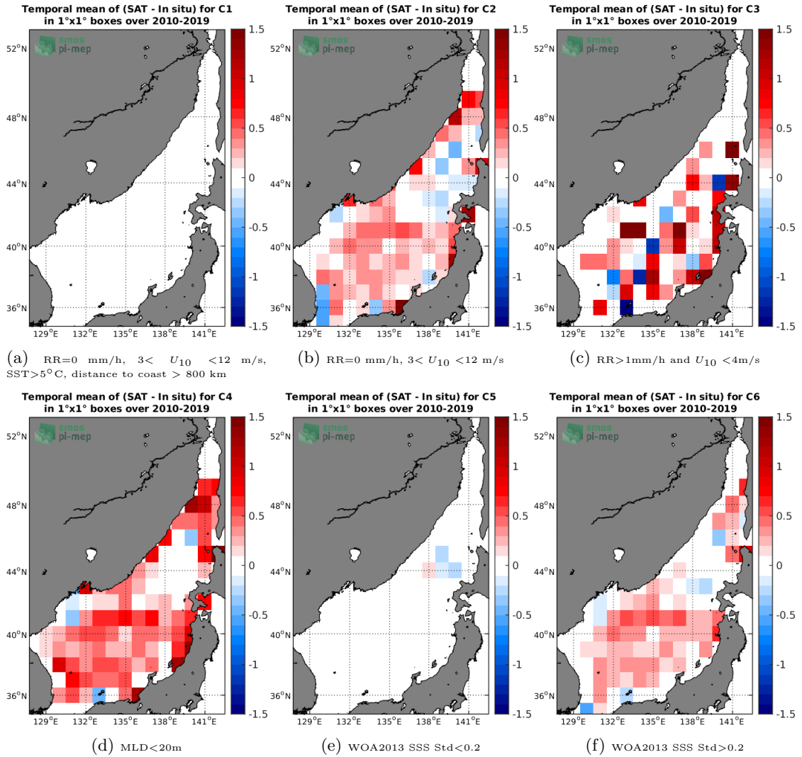
Figure 12: Temporal mean gridded over spatial boxes of size 1^\circ \times 1^\circ of \Delta SSS (SMOS-L3-CATDS-CECOS-LOCEAN-V4-18DAYS-25KM - Argo) for 6 different subdatasets corresponding to: RR=0 mm/h, 3 < U_{10} < 12 m/s, SST > 5^\circ\text{C} , distance to coast > 800 km (a), RR=0 mm/h, 3 < U_{10} < 12 m/s (b), RR > 1 mm/h and U_{10} < 4 m/s (c), MLD < 20 m (d), WOA2013 SSS Std < 0.2 (e), WOA2013 SSS Std > 0.2 (f).
