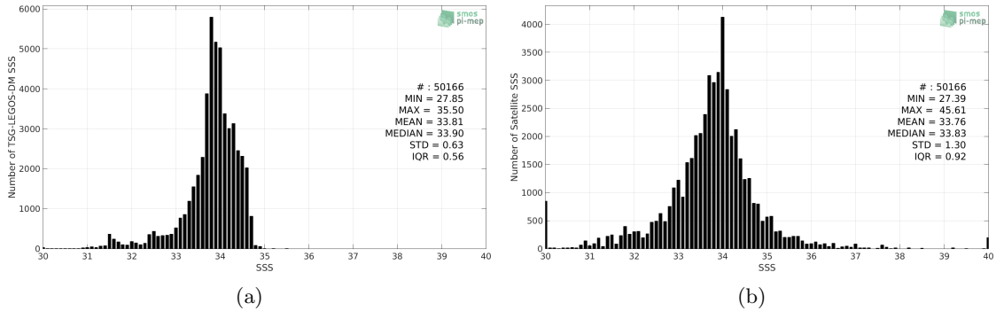
Figure 2: Histograms of SSS from TSG-LEGOS-DM (a) and SMOS-L3-CATDS-CECOS-LOCEAN-V3-9DAYS-25KM (b) considering all match-up pairs per bins of 0.1 over the Sea of Japan Pi-MEP region and for the full satellite product period.
