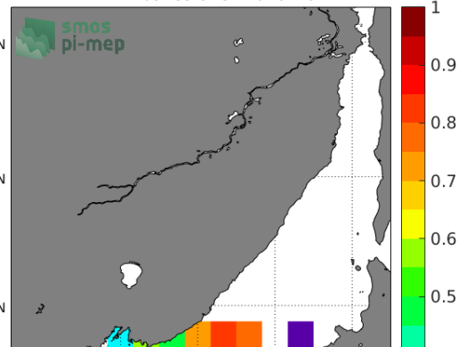
Temporal STD of (Sat - TSG-LEGOS-DM) in 1°x1° boxes over 2010-2017
