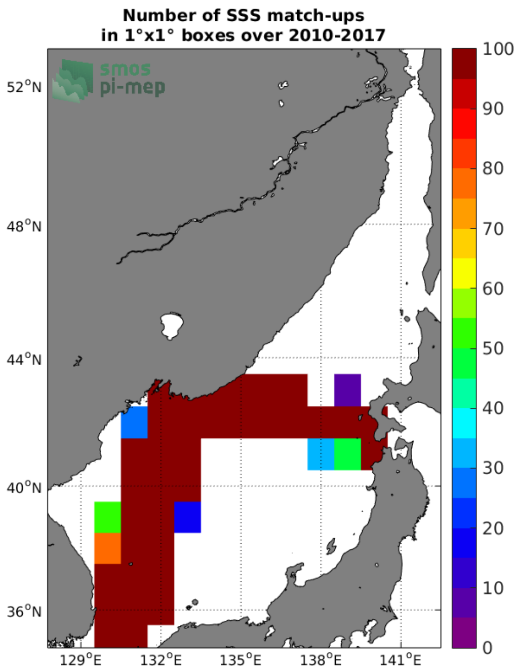
Figure 4: Number of SSS match-ups between TSG-LEGOS-DM SSS and the SMOS-L3-CATDS-CECOS-LOCEAN-V3-9DAYS-25KM SSS product for the Sea of Japan Pi-MEP region over 1°x1° boxes and for the full satellite product period.
