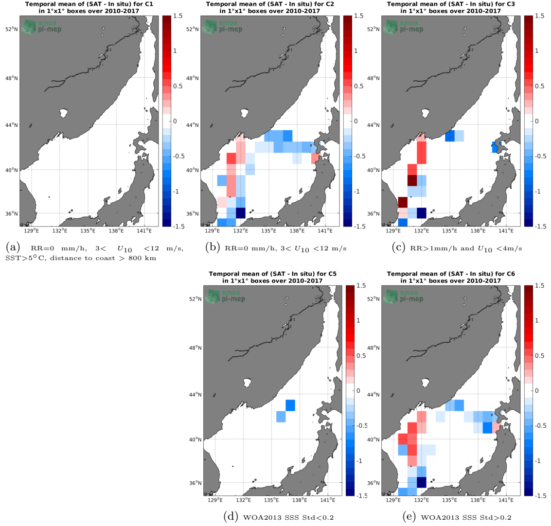
Figure 12: Temporal mean gridded over spatial boxes of size 1°x1° of \Delta\text{SSS} (SMOS-L3-CATDS-CECOS-LOCEAN-V3-9DAYS-25KM - TSG-LEGOS-DM) for 5 different subdatasets corresponding to: RR=0 mm/h, 3 < U_{10} < 12 m/s, SST > 5^\circ\text{C} , distance to coast > 800 km (a), RR=0 mm/h, 3 < U_{10} < 12 m/s (b), RR > 1 mm/h and U_{10} < 4 m/s (c), WOA2013 SSS Std < 0.2 (d), WOA2013 SSS Std > 0.2 (e).
