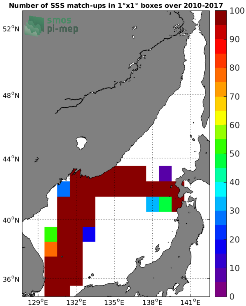
Figure 4: Number of SSS match-ups between TSG-LEGOS-DM SSS and the SMOS-L3-CATDS-CECOS-LOCEAN-V3-9DAYS-25KM SSS product for the Sea of Japan Pi-MEP region over 1°x1° boxes and for the full satellite product period.
