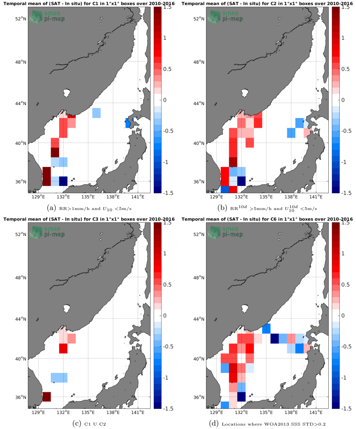
Figure 12: Temporal mean gridded over spatial boxes of size 1°x1° of \Delta\text{SSS} (SMOS-L3-CATDS-CECOS-LOCEAN-V3-9DAYS-25KM - TSG-LEGOS-DM) for 4 different subdatasets corresponding to: RR > 1\text{mm/h} and U_{10} < 5\text{m/s} (a), RR^{10d} > 5\text{mm/h} and U_{10}^{10d} < 5\text{m/s} (b), C1 U C2 (c), Locations where WOA2013 SSS STD > 0.2 (d).
