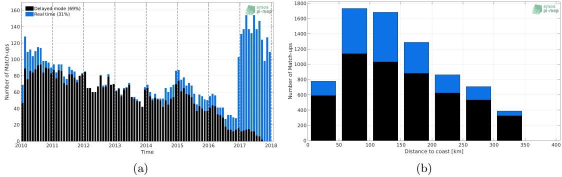
Figure 1: Number of match-ups between Argo and SMOS-L3-CATDS-CECOS-LOCEAN-V3-9DAYS-25KM SSS as a function of time (a) and as function of the distance to coast (b) over the Sea of Japan Pi-MEP region and for the full satellite product period.
