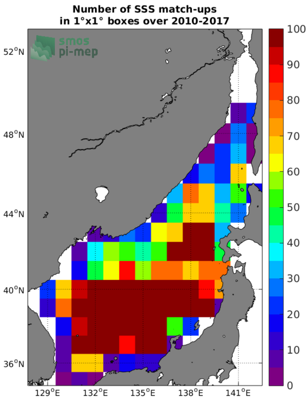
Figure 4: Number of SSS match-ups between Argo SSS and the SMOS-L3-CATDS-CECOS-LOCEAN-V3-9DAYS-25KM SSS product for the Sea of Japan Pi-MEP region over 1°x1° boxes and for the full satellite product period.
