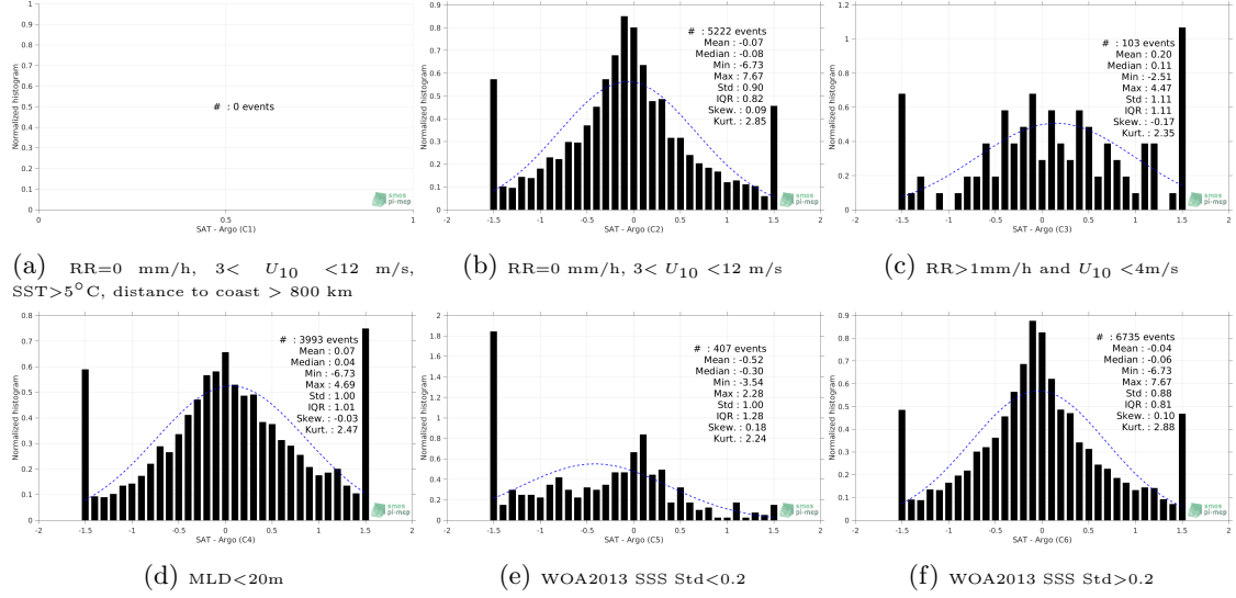
Figure 13: Normalized histogram of \Delta SSS (SMOS-L3-CATDS-CECOS-LOCEAN-V3-9DAYS-25KM - Argo) for 6 different subdatasets corresponding to: RR=0 mm/h, 3 < U_{10} < 12 m/s, SST > 5^{\circ}\text{C} , distance to coast > 800 km (a), RR=0 mm/h, 3 < U_{10} < 12 m/s (b), RR > 1\text{mm/h} and U_{10} < 4\text{m/s} (c), MLD < 20\text{m} (d), WOA2013 SSS Std < 0.2 (e), WOA2013 SSS Std > 0.2 (f).
