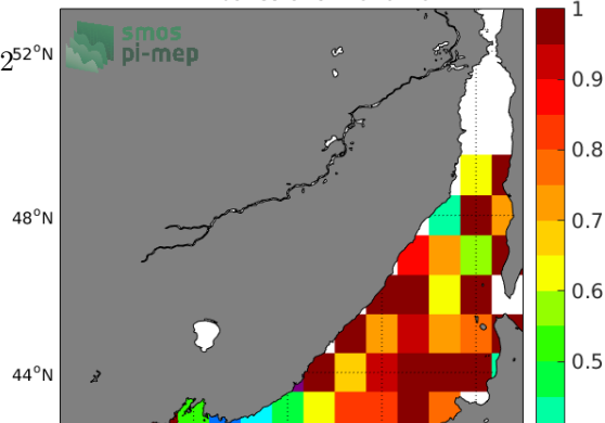
Temporal STD of (Sat - Argo) in 1°x1° boxes over 2010-2017
