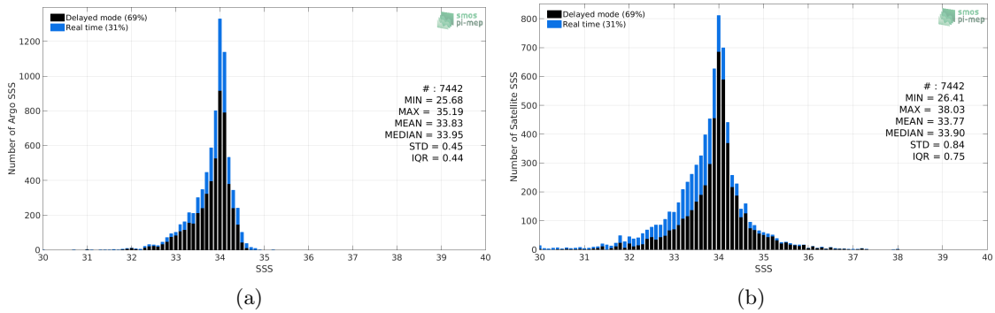
Figure 2: Histograms of SSS from Argo (a) and SMOS-L3-CATDS-CECOS-LOCEAN-V3-9DAYS-25KM (b) considering all match-up pairs per bins of 0.1 over the Sea of Japan Pi-MEP region and for the full satellite product period.
