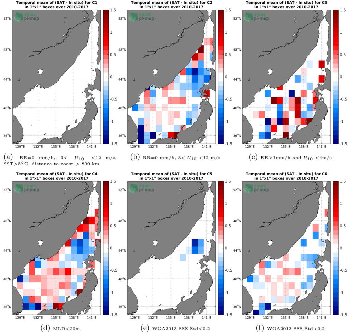
Figure 12: Temporal mean gridded over spatial boxes of size 1°x1° of \Delta SSS (SMOS-L3-CATDS-CECOS-LOCEAN-V3-9DAYS-25KM - Argo) for 6 different subdatasets corresponding to: RR=0 mm/h, 3 < U_{10} < 12 m/s, SST > 5^\circ\text{C} , distance to coast > 800 km (a), RR=0 mm/h, 3 < U_{10} < 12 m/s (b), RR > 1 mm/h and U_{10} < 4 m/s (c), MLD < 20 m (d), WOA2013 SSS Std < 0.2 (e), WOA2013 SSS Std > 0.2 (f).
