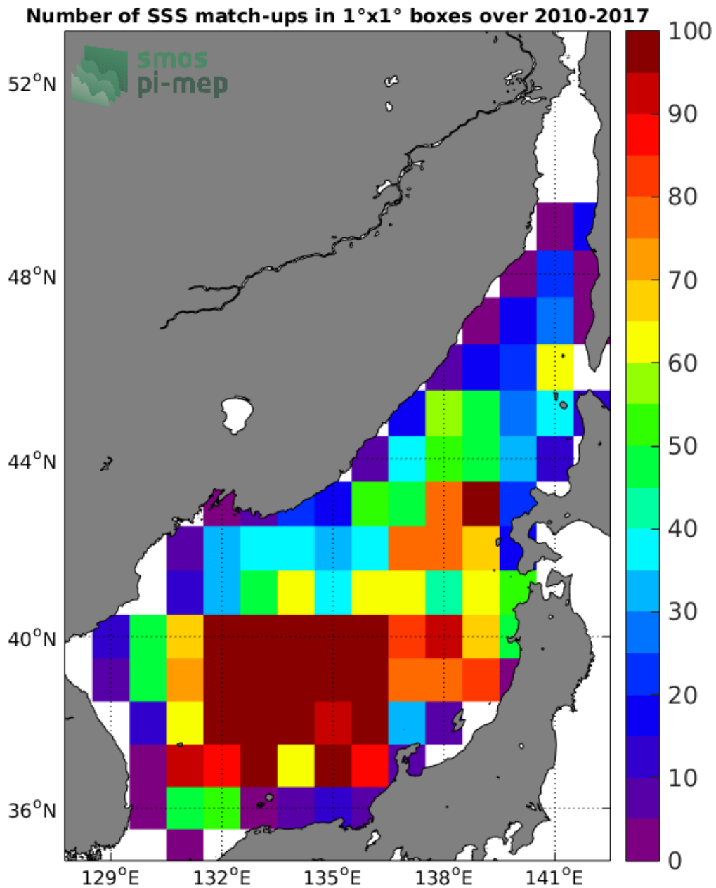
Figure 4: Number of SSS match-ups between Argo SSS and the SMOS-L3-CATDS-CECOS-LOCEAN-V3-9DAYS-25KM SSS product for the Sea of Japan Pi-MEP region over 1°x1° boxes and for the full satellite product period.
