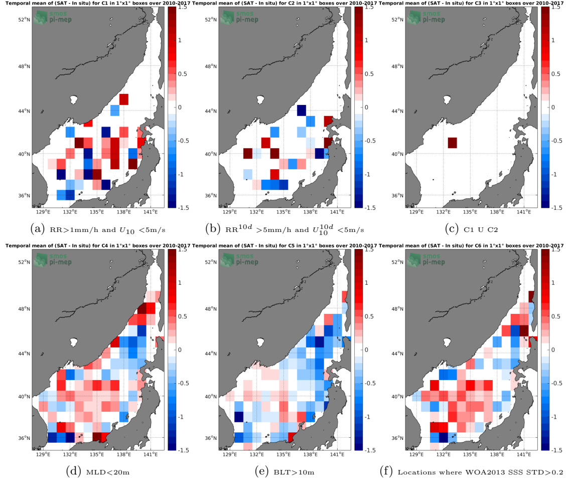
Figure 12: Temporal mean gridded over spatial boxes of size 1^\circ \times 1^\circ of \Delta\text{SSS} (SMOS-L3-CATDS-CECOS-LOCEAN-V3-9DAYS-25KM - Argo) for 6 different subdatasets corresponding to: \text{RR} > 1\text{mm/h} and U_{10} < 5\text{m/s} (a), \text{RR}^{10d} > 5\text{mm/h} and U_{10}^{10d} < 5\text{m/s} (b), C1 U C2 (c), \text{MLD} < 20\text{m} (d), \text{BLT} > 10\text{m} (e), Locations where WOA2013 SSS STD > 0.2 (f).
