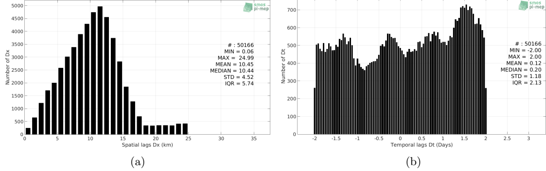
Figure 5: Histograms of the spatial (a) and temporal (b) lags between the time of the TSG-LEGOS-DM measurements and the date of the corresponding SMOS-L3-CATDS-CECOS-LOCEAN-V3-18DAYS-25KM SSS product.
