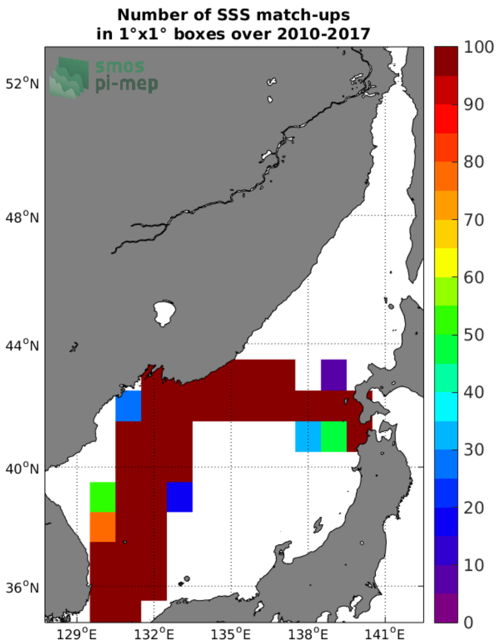
Figure 4: Number of SSS match-ups between TSG-LEGOS-DM SSS and the SMOS-L3-CATDS-CECOS-LOCEAN-V3-18DAYS-25KM SSS product for the Sea of Japan Pi-MEP region over 1°x1° boxes and for the full satellite product period.
