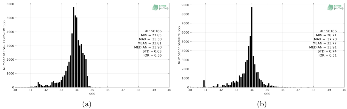
Figure 2: Histograms of SSS from TSG-LEGOS-DM (a) and SMOS-L3-CATDS-CECOS-LOCEAN-V3-18DAYS-25KM (b) considering all match-up pairs per bins of 0.1 over the Sea of Japan Pi-MEP region and for the full satellite product period.
