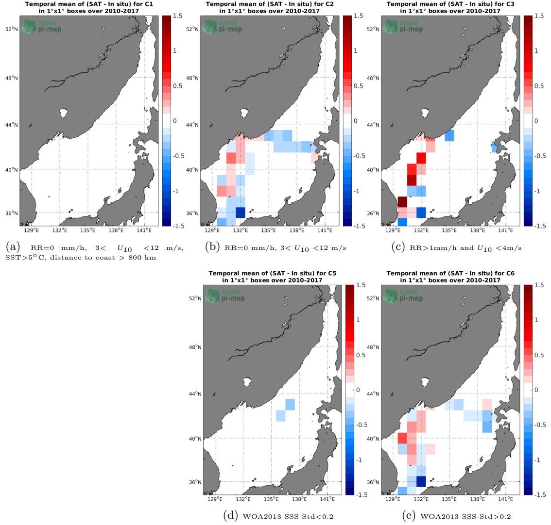
Figure 12: Temporal mean gridded over spatial boxes of size 1°x1° of \Delta\text{SSS} (SMOS-L3-CATDS-CECOS-LOCEAN-V3-18DAYS-25KM - TSG-LEGOS-DM) for 5 different subdatasets corresponding to: RR=0 mm/h, 3 < U_{10} < 12 m/s, SST > 5^\circ\text{C} , distance to coast > 800 km (a), RR=0 mm/h, 3 < U_{10} < 12 m/s (b), RR > 1 mm/h and U_{10} < 4 m/s (c), WOA2013 SSS Std < 0.2 (d), WOA2013 SSS Std > 0.2 (e).
