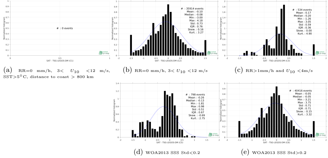
Figure 13: Normalized histogram of \Delta\text{SSS} (SMOS-L3-CATDS-CECOS-LOCEAN-V3-18DAYS-25KM - TSG-LEGOS-DM) for 5 different subdatasets corresponding to: RR=0 mm/h, 3 < U_{10} < 12 m/s, SST > 5^{\circ}\text{C} , distance to coast > 800 km (a), RR=0 mm/h, 3 < U_{10} < 12 m/s (b), RR > 1\text{mm/h} and U_{10} < 4\text{m/s} (c), WOA2013 SSS Std < 0.2 (d), WOA2013 SSS Std > 0.2 (e).
