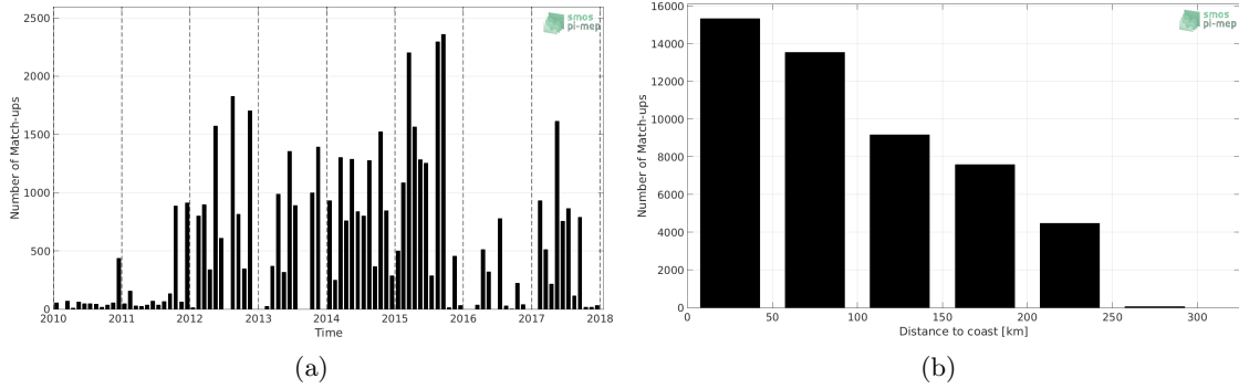
Figure 1: Number of match-ups between TSG-LEGOS-DM and SMOS-L3-CATDS-CECOS-LOCEAN-V3-18DAYS-25KM SSS as a function of time (a) and as function of the distance to coast (b) over the Sea of Japan Pi-MEP region and for the full satellite product period.
