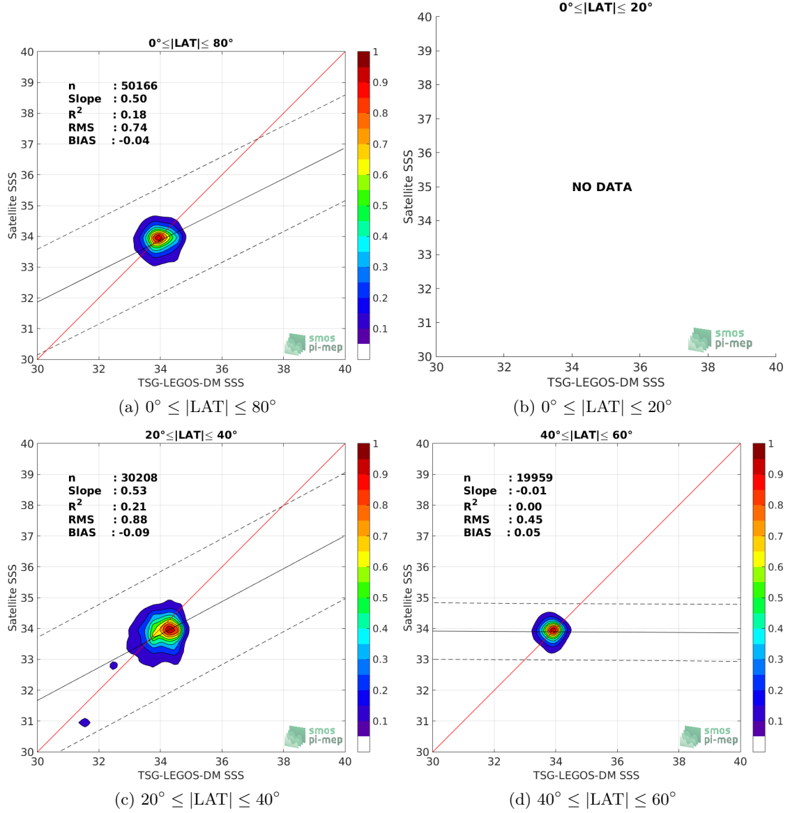
Figure 9: Contour maps of the concentration of SMOS-L3-CATDS-CECOS-LOCEAN-V3-18DAYS-25KM SSS (y-axis) versus TSG-LEGOS-DM SSS (x-axis) at match-up pairs for different latitude bands. For each plot, the red line shows x=y . The black thin and dashed lines indicate a linear fit through the data cloud and the \pm 95\% confidence levels, respectively. The number match-up pairs n , the slope and R^2 coefficient of the linear fit, the root mean square (RMS) and the mean bias between satellite and in situ data are indicated for each latitude band in each plots.
