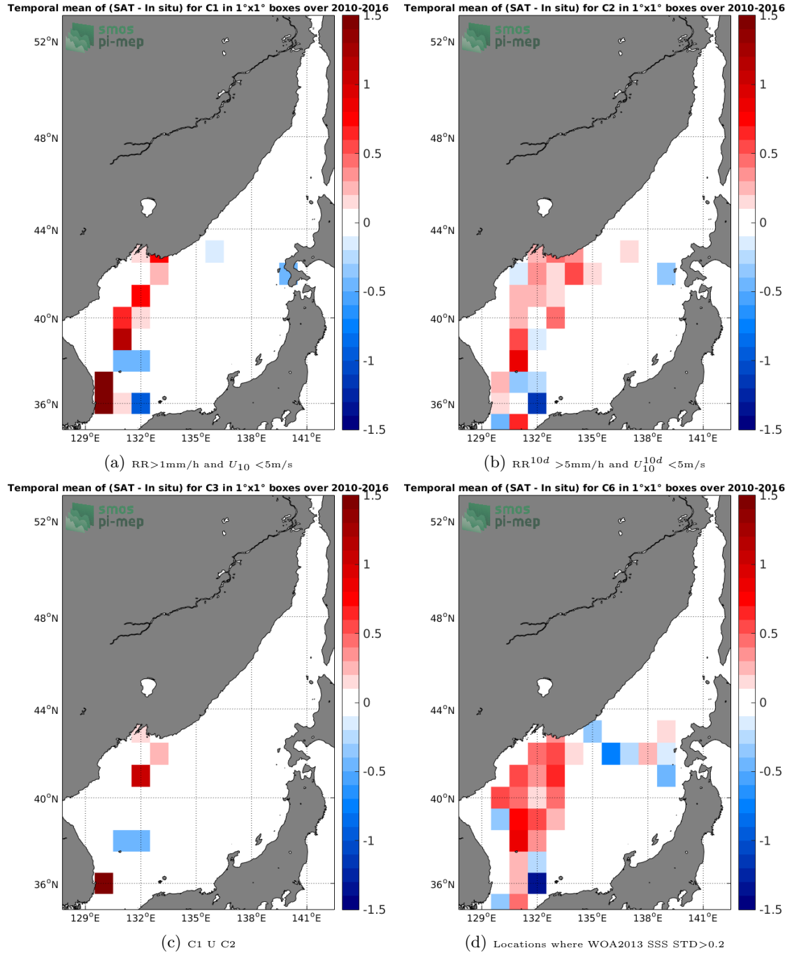
Figure 12: Temporal mean gridded over spatial boxes of size 1^\circ \times 1^\circ of \Delta\text{SSS} (SMOS-L3-CATDS-CECOS-LOCEAN-V3-18DAYS-25KM - TSG-LEGOS-DM) for 4 different subdatasets corresponding to: RR > 1\text{mm/h} and U_{10} < 5\text{m/s} (a), RR^{10d} > 5\text{mm/h} and U_{10}^{10d} < 5\text{m/s} (b), C1 U C2 (c), Locations where WOA2013 SSS STD > 0.2 (d).
