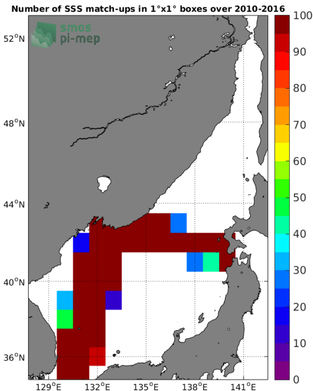
Figure 4: Number of SSS match-ups between TSG-LEGOS-DM SSS and the SMOS-L3-CATDS-CECOS-LOCEAN-V3-18DAYS-25KM SSS product for the Sea of Japan Pi-MEP region over 1°x1° boxes and for the full satellite product period.
