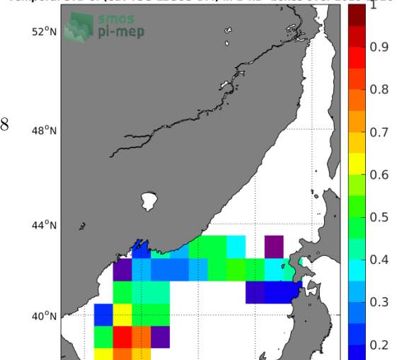
Temporal STD of (Sat-TSG-LEGOS-DM) in 1^{\circ} \times 1^{\circ} boxes over 2010-2016
