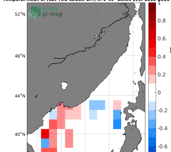
Temporal mean of (Sat-TSG-LEGOS-DM) in 1^{\circ} \times 1^{\circ} boxes over 2010-2016
