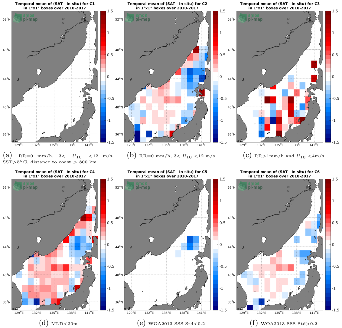
Figure 12: Temporal mean gridded over spatial boxes of size 1°x1° of \Delta\text{SSS} (SMOS-L3-CATDS-CECOS-LOCEAN-V3-18DAYS-25KM - Argo) for 6 different subdatasets corresponding to: RR=0 mm/h, 3 < U_{10} < 12 m/s, SST > 5^\circ\text{C} , distance to coast > 800 km (a), RR=0 mm/h, 3 < U_{10} < 12 m/s (b), RR > 1 mm/h and U_{10} < 4 m/s (c), MLD < 20\text{m} (d), WOA2013 SSS Std < 0.2 (e), WOA2013 SSS Std > 0.2 (f).
