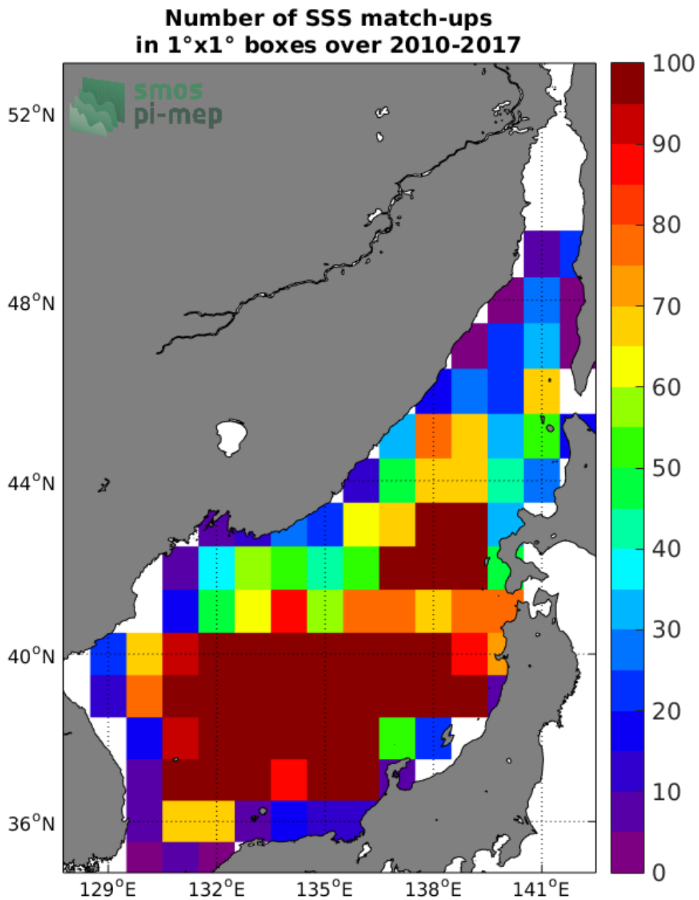
Figure 4: Number of SSS match-ups between Argo SSS and the SMOS-L3-CATDS-CECOS-LOCEAN-V3-18DAYS-25KM SSS product for the Sea of Japan Pi-MEP region over 1°x1° boxes and for the full satellite product period.
