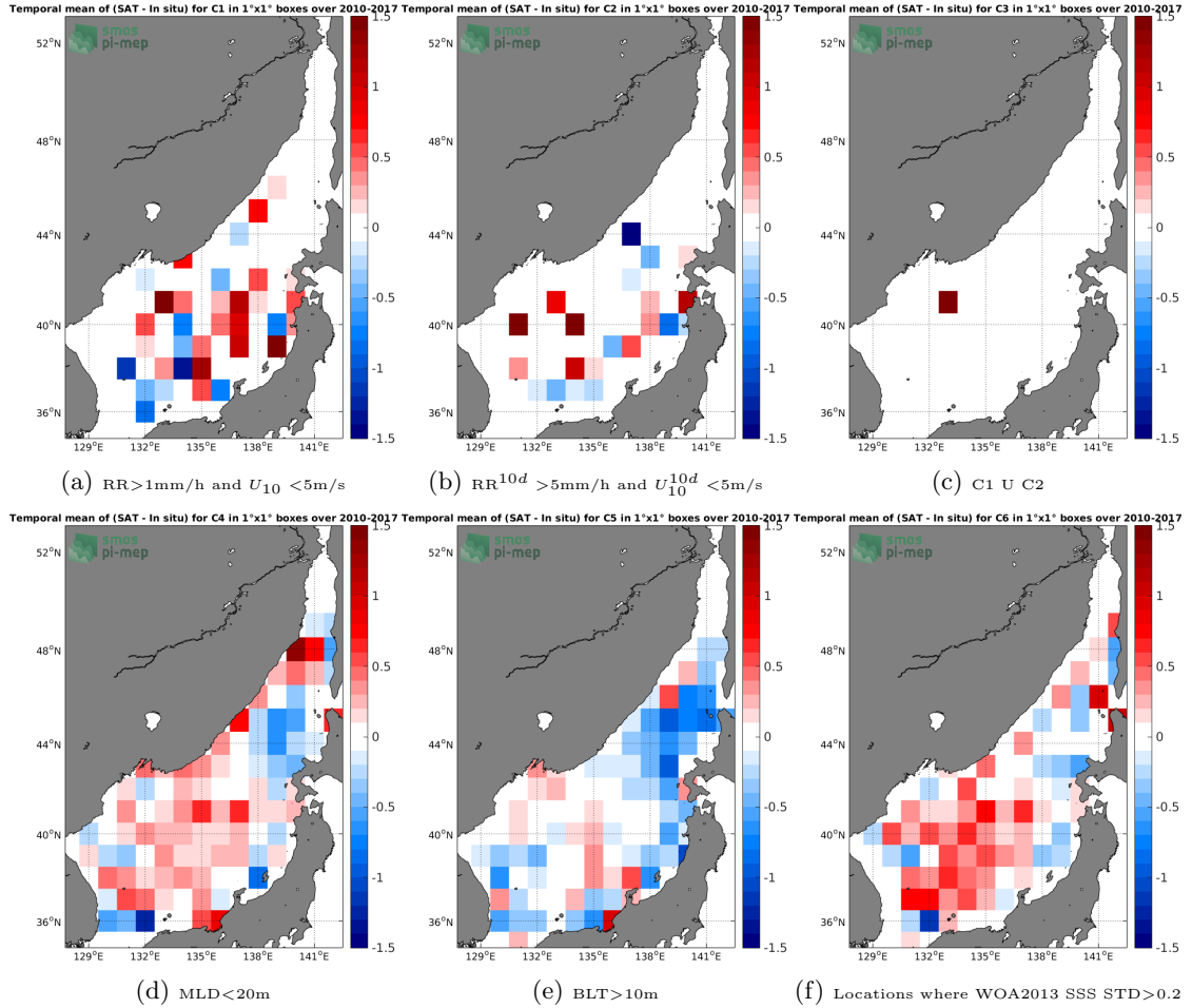
Figure 12: Temporal mean gridded over spatial boxes of size 1°x1° of \Delta SSS (SMOS-L3-CATDS-CECOS-LOCEAN-V3-18DAYS-25KM - Argo) for 6 different subdatasets corresponding to:RR>1mm/h and U_{10} < 5 m/s (a), RR^{10d} > 5 mm/h and U_{10}^{10d} < 5 m/s (b), C1 U C2 (c),MLD<20m (d),BLT>10m (e),Locations where WOA2013 SSS STD>0.2 (f).
