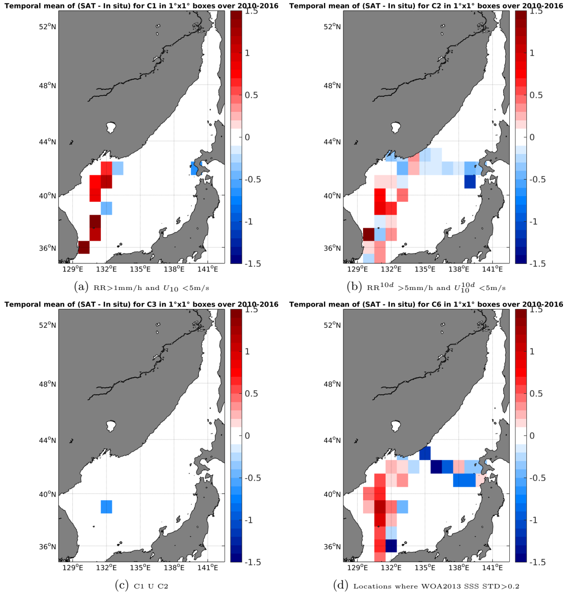
Figure 12: Temporal mean gridded over spatial boxes of size 1°x1° of \Delta SSS (SMOS-L3-CATDS-CECOS-LOCEAN-V2.1-9DAYS-25KM - TSG-LEGOS-DM) for 4 different subdatasets corresponding to: RR > 1\text{mm/h} and U_{10} < 5\text{m/s} (a), RR^{10d} > 5\text{mm/h} and U_{10}^{10d} < 5\text{m/s} (b), C1 U C2 (c), Locations where WOA2013 SSS STD > 0.2 (d).
