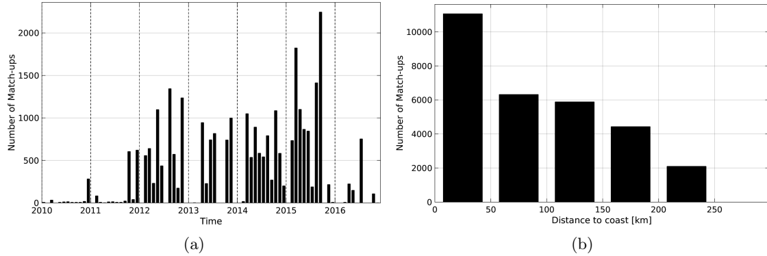
Figure 1: Number of match-ups between TSG-LEGOS-DM and SMOS-L3-CATDS-CECOS-LOCEAN-V2.1-9DAYS-25KM SSS as a function of time (a) and as function of the distance to coast (b) over the Sea of Japan Pi-MEP region and for the full satellite product period.
