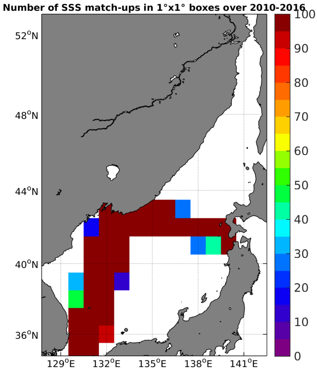
Figure 4: Number of SSS match-ups between TSG-LEGOS-DM SSS and the SMOS-L3-CATDS-CECOS-LOCEAN-V2.1-9DAYS-25KM SSS product for the Sea of Japan Pi-MEP region over 1°x1° boxes and for the full satellite product period.
