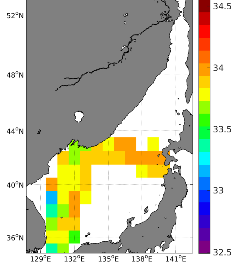
(c) MEAN(TSG-LEGOS-DM SSS)
