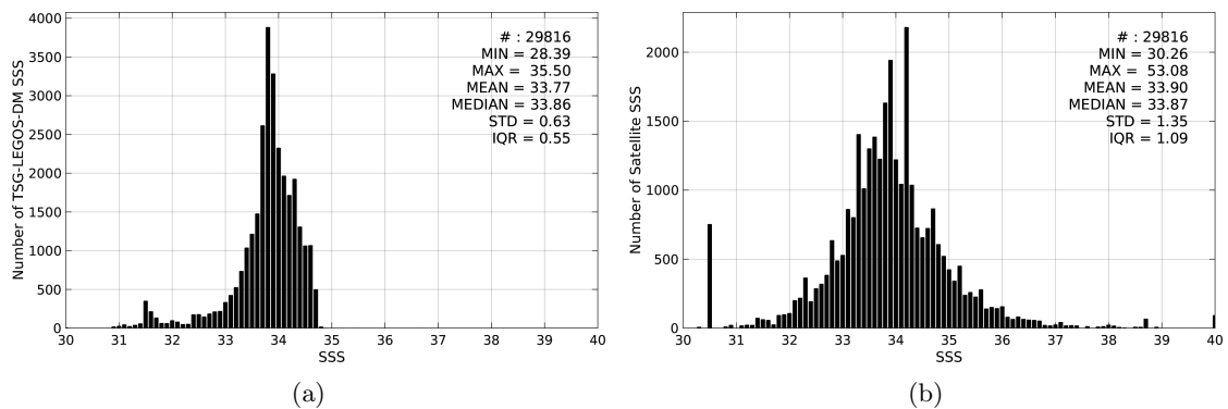
Figure 2: Histograms of SSS from TSG-LEGOS-DM (a) and SMOS-L3-CATDS-CECOS-LOCEAN-V2.1-9DAYS-25KM (b) considering all match-up pairs per bins of 0.1 over the Sea of Japan Pi-MEP region and for the full satellite product period.
