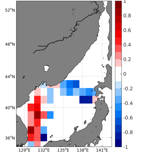
(e) MEAN( \Delta SSS) (Satellite - TSG-LEGOS-DM)
