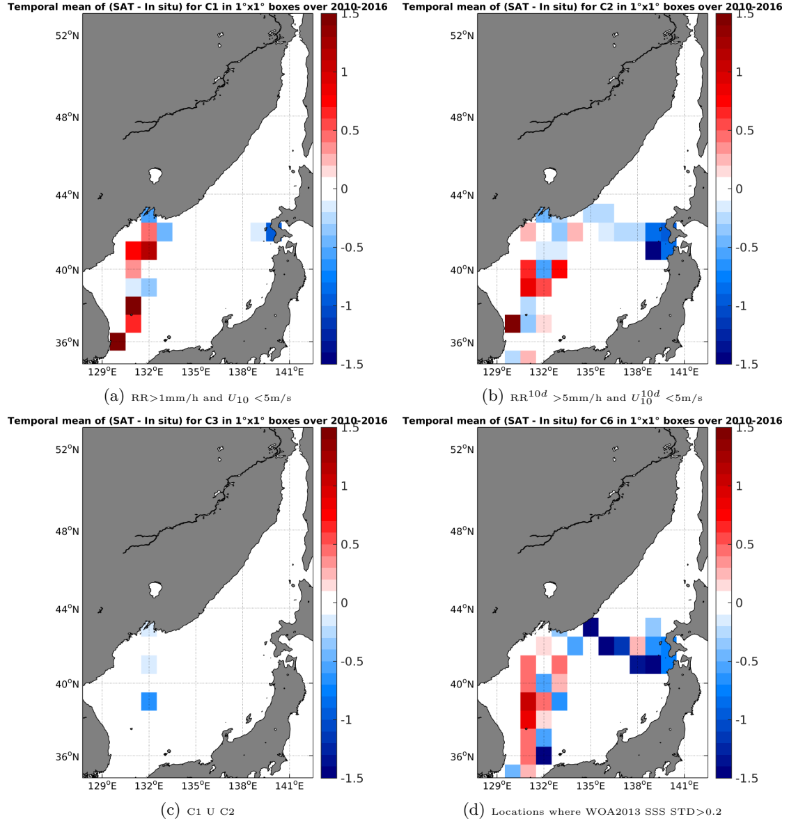
Figure 12: Temporal mean gridded over spatial boxes of size 1^\circ \times 1^\circ of \Delta SSS (SMOS-L3-CATDS-CECOS-LOCEAN-V2-9DAYS-25KM - TSG-LEGOS-DM) for 4 different subdatasets corresponding to: RR>1mm/h and U_{10} < 5\text{m/s} (a), RR^{10d} > 5\text{mm/h} and U_{10}^{10d} < 5\text{m/s} (b), C1 U C2 (c), Locations where WOA2013 SSS STD>0.2 (d).
