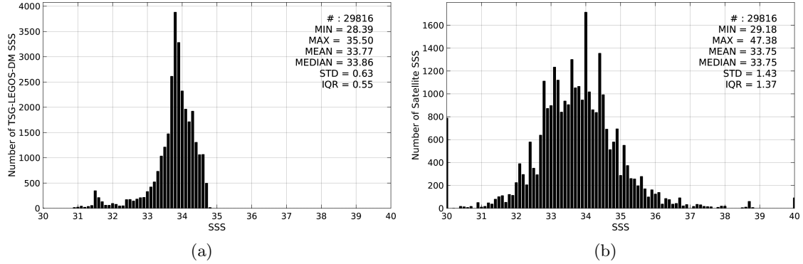
Figure 2: Histograms of SSS from TSG-LEGOS-DM (a) and SMOS-L3-CATDS-CECOS-LOCEAN-V2-9DAYS-25KM (b) considering all match-up pairs per bins of 0.1 over the Sea of Japan Pi-MEP region and for the full satellite product period.
