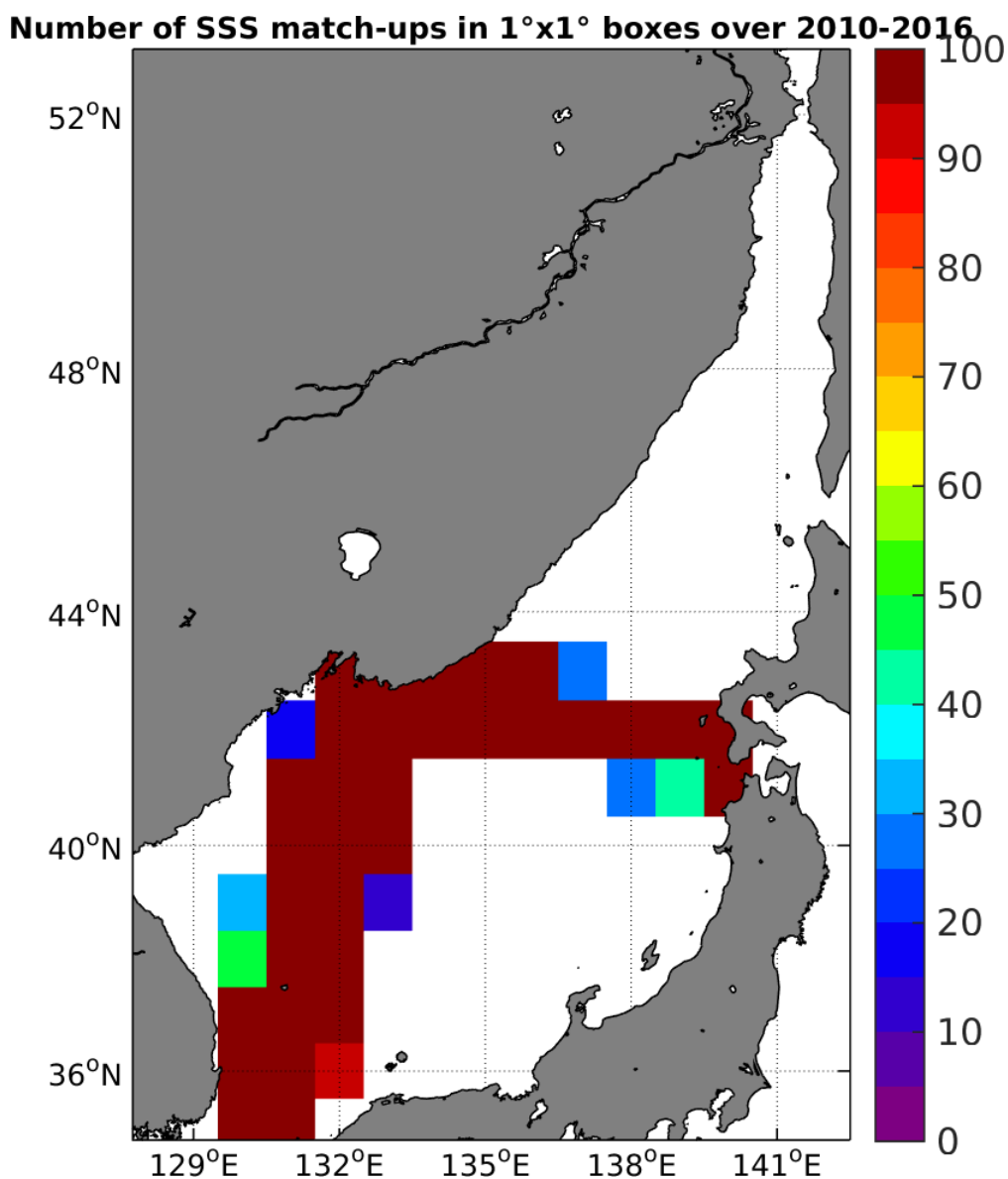
Figure 4: Number of SSS match-ups between TSG-LEGOS-DM SSS and the SMOS-L3-CATDS-CECOS-LOCEAN-V2-9DAYS-25KM SSS product for the Sea of Japan Pi-MEP region over 1°x1° boxes and for the full satellite product period.
