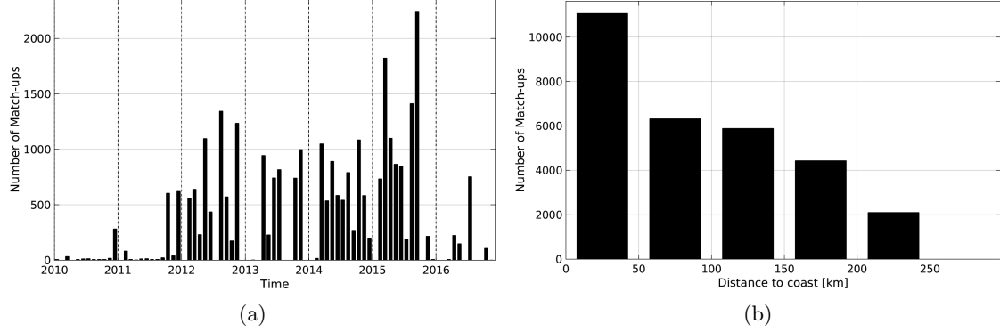
Figure 1: Number of match-ups between TSG-LEGOS-DM and SMOS-L3-CATDS-CECOS-LOCEAN-V2-9DAYS-25KM SSS as a function of time (a) and as function of the distance to coast (b) over the Sea of Japan Pi-MEP region and for the full satellite product period.
