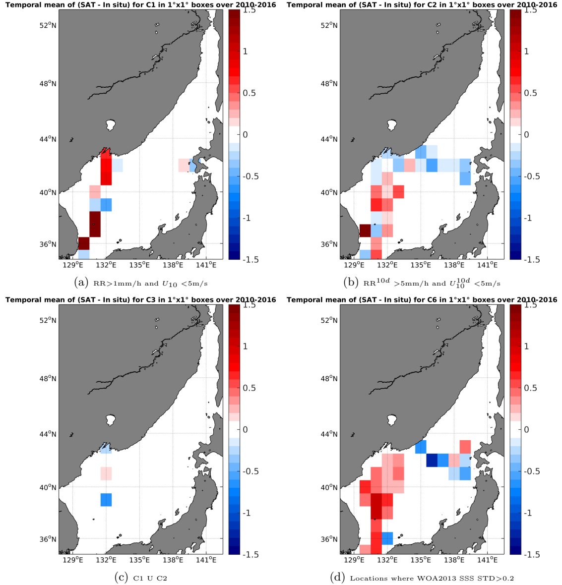
Figure 12: Temporal mean gridded over spatial boxes of size 1^\circ \times 1^\circ of \Delta SSS (SMOS-L3-CATDS-CECOS-LOCEAN-V2-18DAYS-25KM - TSG-LEGOS-DM) for 4 different subdatasets corresponding to: RR > 1 mm/h and U_{10} < 5 m/s (a), RR^{10d} > 5 mm/h and U_{10}^{10d} < 5 m/s (b), C1 U C2 (c), Locations where WOA2013 SSS STD > 0.2 (d).
