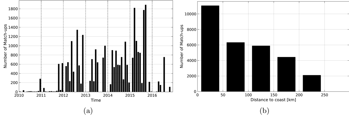
Figure 1: Number of match-ups between TSG-LEGOS-DM and SMOS-L3-CATDS-CECOS-LOCEAN-V2-18DAYS-25KM SSS as a function of time (a) and as function of the distance to coast (b) over the Sea of Japan Pi-MEP region and for the full satellite product period.
