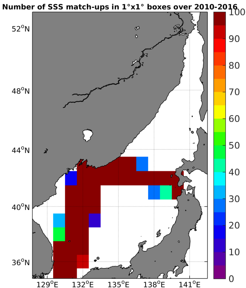
Figure 4: Number of SSS match-ups between TSG-LEGOS-DM SSS and the SMOS-L3-CATDS-CECOS-LOCEAN-V2-18DAYS-25KM SSS product for the Sea of Japan Pi-MEP region over 1°x1° boxes and for the full satellite product period.
