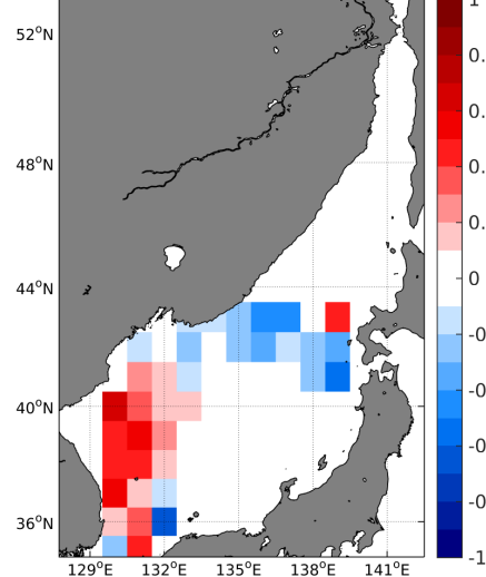
(e) MEAN( \Delta SSS) (Satellite - TSG-LEGOS-DM)
