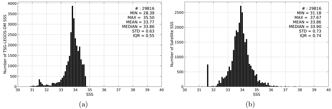
Figure 2: Histograms of SSS from TSG-LEGOS-DM (a) and SMOS-L3-CATDS-CECOS-LOCEAN-V2-18DAYS-25KM (b) considering all match-up pairs per bins of 0.1 over the Sea of Japan Pi-MEP region and for the full satellite product period.
