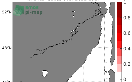
Temporal mean of (Sat - TSG (LEGOS-DM)) in 1°x1° boxes over 2011-2017
