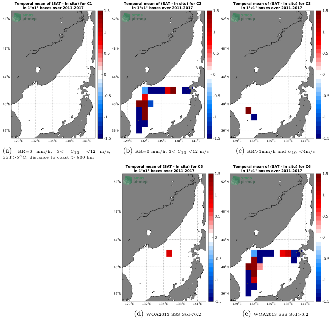
Figure 12: Temporal mean gridded over spatial boxes of size 1°x1° of \Delta SSS (SMOS SSS L3 v2 - Monthly - 0.25 Deg (CATDS-CECOS-IFREMER) - TSG (LEGOS-DM)) for 5 different subdatasets corresponding to:RR=0 mm/h, 3 < U_{10} < 12 m/s, SST>5°C, distance to coast > 800 km (a), RR=0 mm/h, 3 < U_{10} < 12 m/s (b), RR>1mm/h and U_{10} < 4 m/s (c), WOA2013 SSS Std<0.2 (d), WOA2013 SSS Std>0.2 (e).
