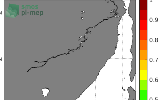
Temporal STD of (Sat - TSG (LEGOS-DM)) in 1°x1° boxes over 2011-2017
