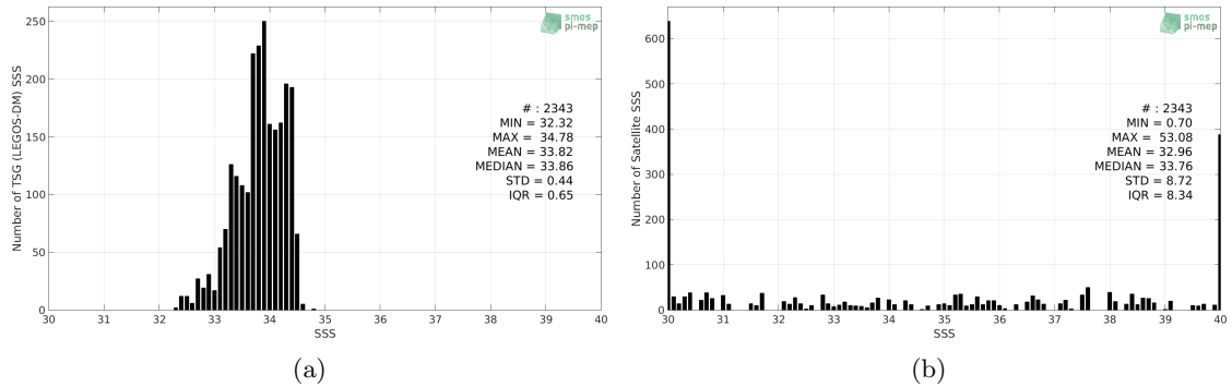
Figure 2: Histograms of SSS from TSG (LEGOS-DM) (a) and SMOS SSS L3 v2 - Monthly - 0.25 Deg (CATDS-CECOS-IFREMER) (b) considering all match-up pairs per bins of 0.1 over the Sea of Japan Pi-MEP region and for the full satellite product period.
