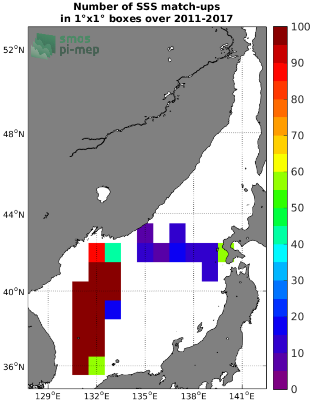
Figure 4: Number of SSS match-ups between TSG (LEGOS-DM) SSS and the SMOS SSS L3 v2 - Monthly - 0.25 Deg (CATDS-CECOS-IFREMER) SSS product for the Sea of Japan Pi-MEP region over 1°x1° boxes and for the full satellite product period.
