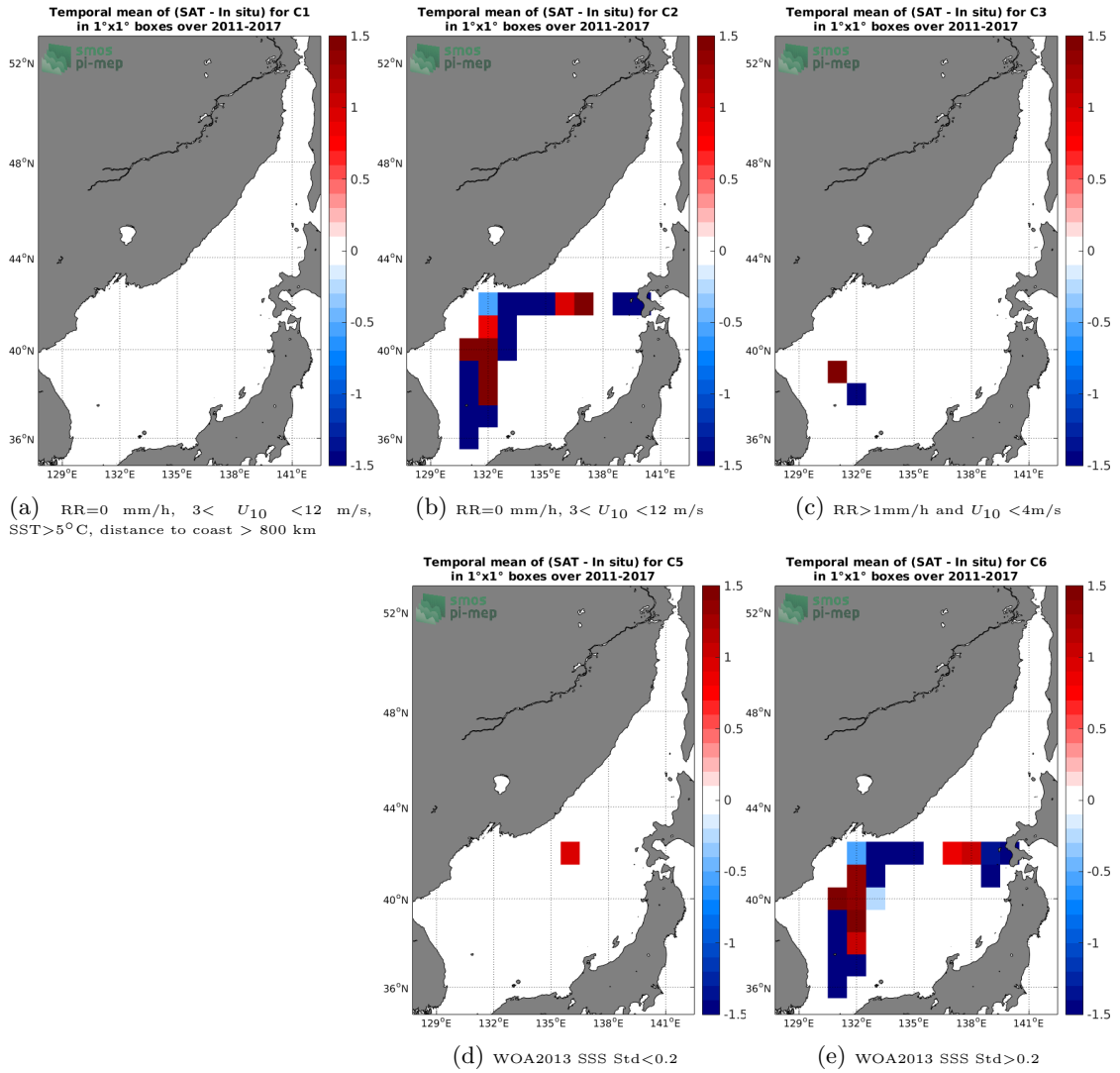
Figure 12: Temporal mean gridded over spatial boxes of size 1°x1° of \Delta\text{SSS} (SMOS L3 v2 - Monthly - 0.25 Deg (CATDS-CECOS-IFREMER) - TSG-LEGOS-DM) for 5 different subdatasets corresponding to:RR=0 mm/h, 3 < U_{10} < 12 m/s, SST>5°C, distance to coast > 800 km (a), RR=0 mm/h, 3 < U_{10} < 12 m/s (b), RR>1mm/h and U_{10} < 4\text{m/s} (c), WOA2013 SSS Std<0.2 (d), WOA2013 SSS Std>0.2 (e).
