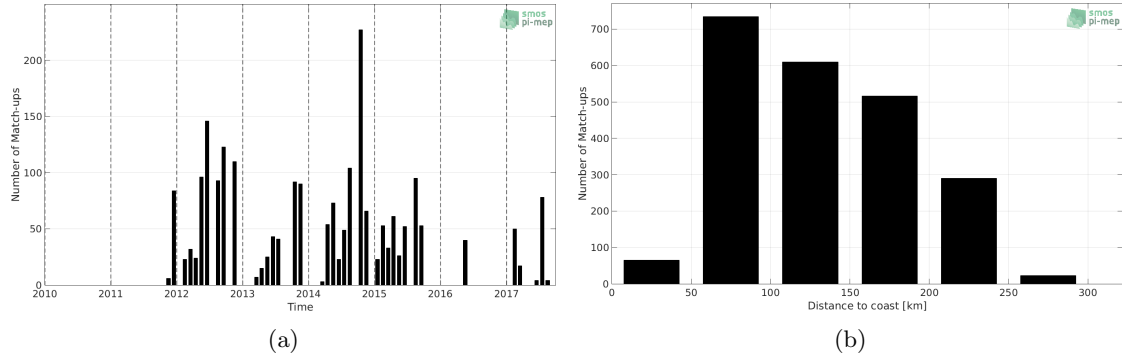
Figure 1: Number of match-ups between TSG-LEGOS-DM and SMOS L3 v2 - Monthly - 0.25 Deg (CATDS-CECOS-IFREMER) SSS as a function of time (a) and as function of the distance to coast (b) over the Sea of Japan Pi-MEP region and for the full satellite product period.
