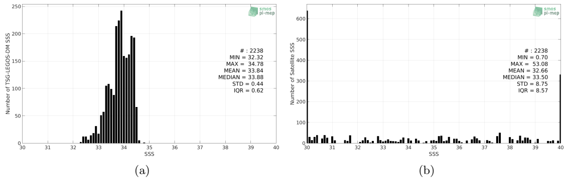
Figure 2: Histograms of SSS from TSG-LEGOS-DM (a) and SMOS L3 v2 - Monthly - 0.25 Deg (CATDS-CECOS-IFREMER) (b) considering all match-up pairs per bins of 0.1 over the Sea of Japan Pi-MEP region and for the full satellite product period.
