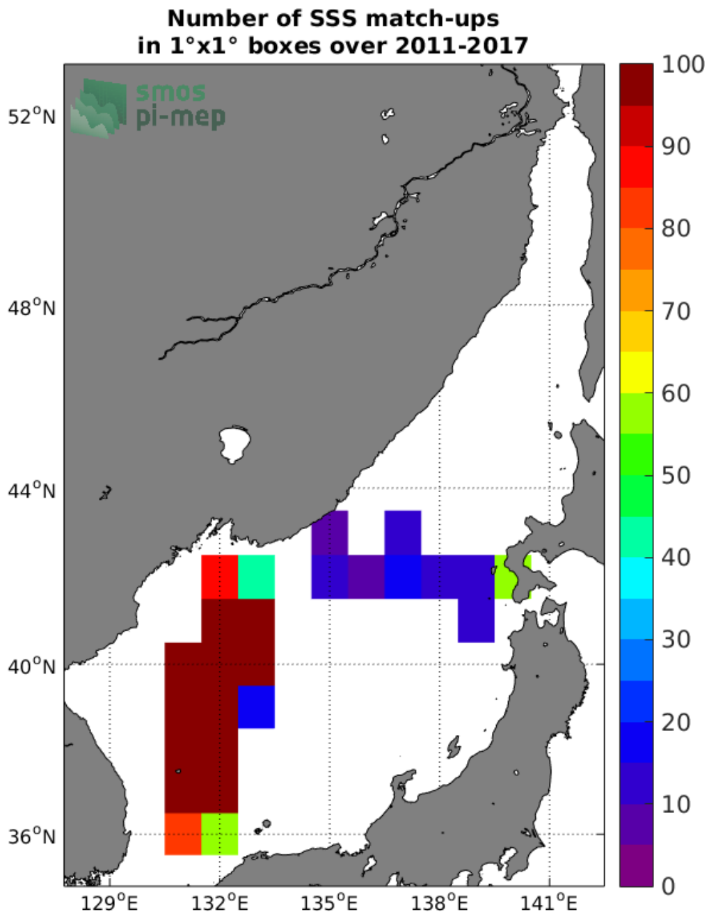
Figure 4: Number of SSS match-ups between TSG-LEGOS-DM SSS and the SMOS L3 v2 - Monthly - 0.25 Deg (CATDS-CECOS-IFREMER) SSS product for the Sea of Japan Pi-MEP region over 1°x1° boxes and for the full satellite product period.
