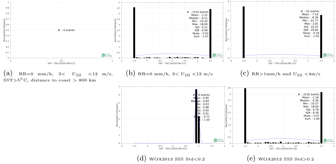
Figure 13: Normalized histogram of \Delta SSS (SMOS L3 v2 - Monthly - 0.25 Deg (CATDS-CECOS-IFREMER) - TSG-LEGOS-DM) for 5 different subdatasets corresponding to: RR=0 mm/h, 3 < U_{10} < 12 m/s, SST > 5°C, distance to coast > 800 km (a), RR=0 mm/h, 3 < U_{10} < 12 m/s (b), RR > 1mm/h and U_{10} < 4 m/s (c), WOA2013 SSS Std < 0.2 (d), WOA2013 SSS Std > 0.2 (e).
