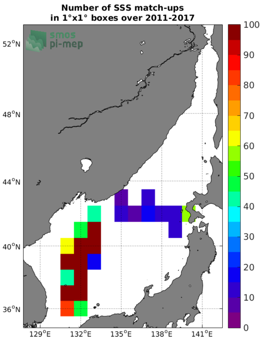
Figure 4: Number of SSS match-ups between TSG-LEGOS-DM SSS and the SMOS-L3-CATDS-IFREMER-CECOS-V2-MONTHLY-0.25DEG SSS product for the Sea of Japan Pi-MEP region over 1°x1° boxes and for the full satellite product period.
