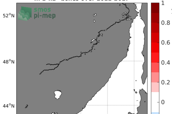
Temporal mean of (Sat - TSG-LEGOS-DM) in 1°x1° boxes over 2011-2017
