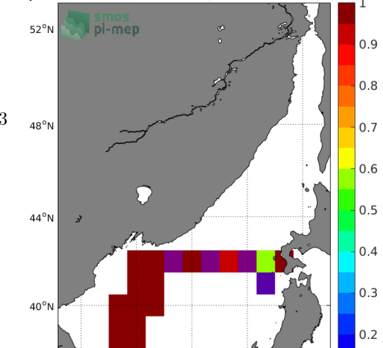
Temporal STD of (Sat-TSG-LEGOS-DM) in 1°x1° boxes over 2011-2017
