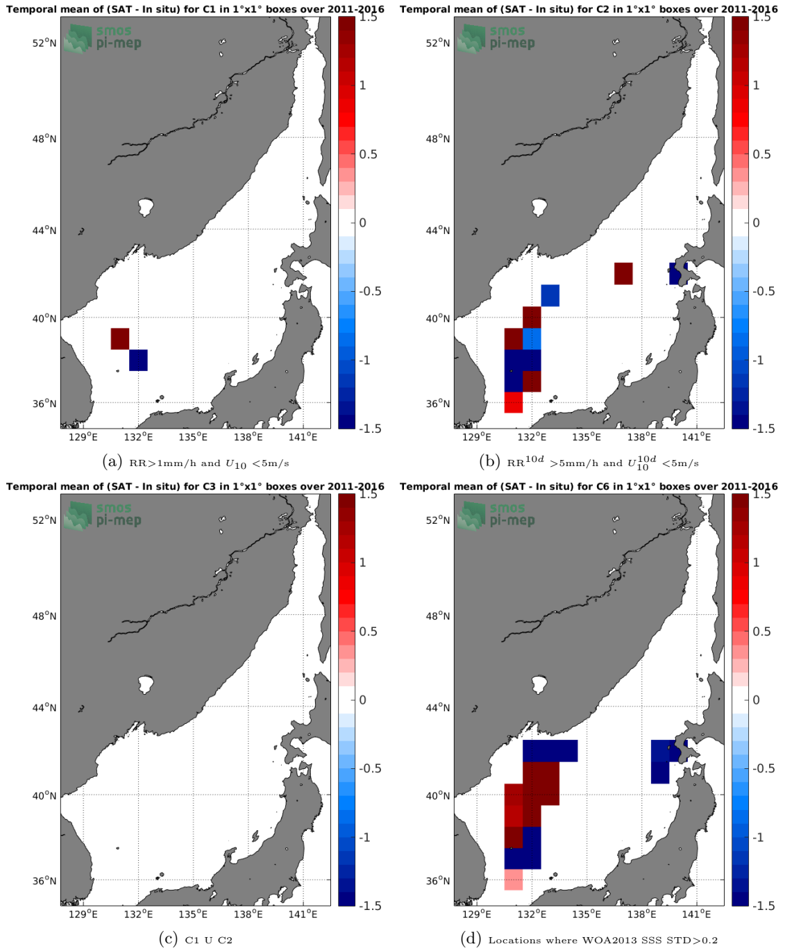
Figure 12: Temporal mean gridded over spatial boxes of size 1°x1° of \Delta\text{SSS} (SMOS-L3-CATDS-IFREMER-CECOS-V2-MONTHLY-0.25DEG - TSG-LEGOS-DM) for 4 different subdatasets corresponding to: RR > 1\text{mm/h} and U_{10} < 5\text{m/s} (a), RR^{10d} > 5\text{mm/h} and U_{10}^{10d} < 5\text{m/s} (b), C1 U C2 (c), Locations where WOA2013 SSS STD > 0.2 (d).
