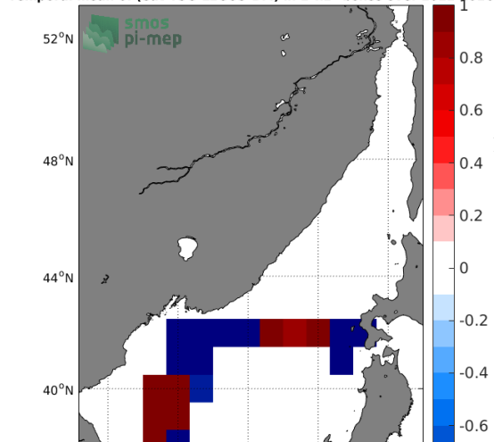
Temporal mean of (Sat-TSG-LEGOS-DM) in 1°x1° boxes over 2011-2016
