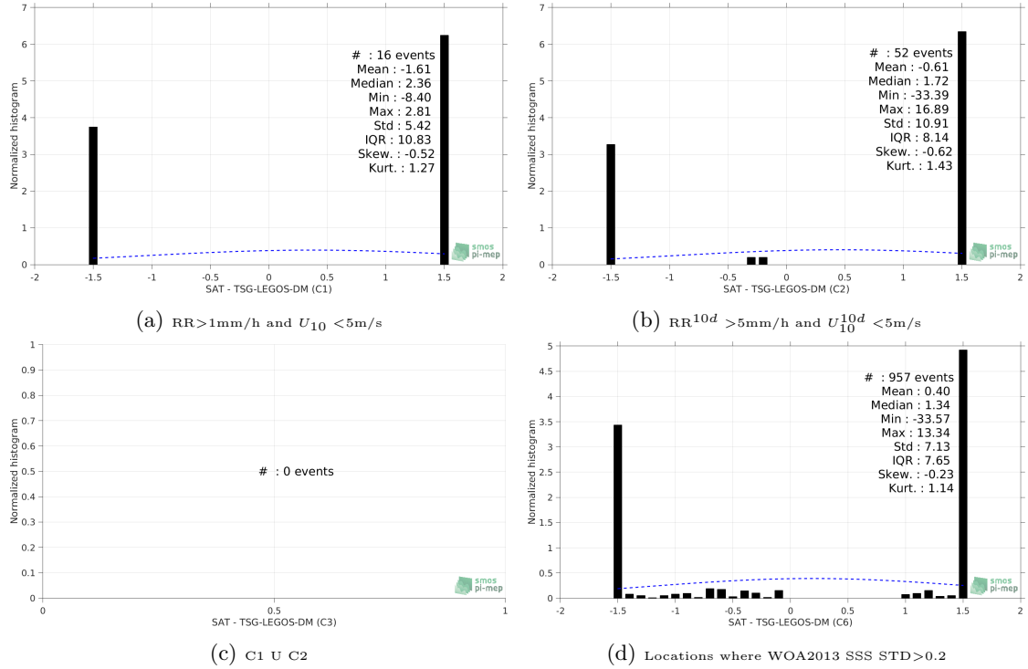
Figure 13: Normalized histogram of \Delta\text{SSS} (SMOS-L3-CATDS-IFREMER-CECOS-V2-MONTHLY-0.25DEG - TSG-LEGOS-DM) for 6 different subdatasets corresponding to: RR > 1\text{mm/h} and U_{10} < 5\text{m/s} (a), RR^{10d} > 5\text{mm/h} and U_{10}^{10d} < 5\text{m/s} (b), C1 U C2 (c), Locations where WOA2013 SSS STD > 0.2 (d).
