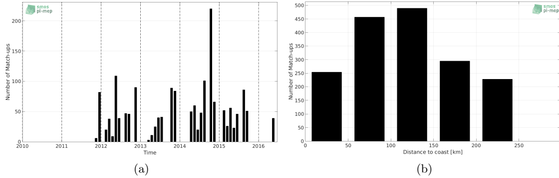
Figure 1: Number of match-ups between TSG-LEGOS-DM and SMOS-L3-CATDS-IFREMER-CECOS-V2-MONTHLY-0.25DEG SSS as a function of time (a) and as function of the distance to coast (b) over the Sea of Japan Pi-MEP region and for the full satellite product period.
