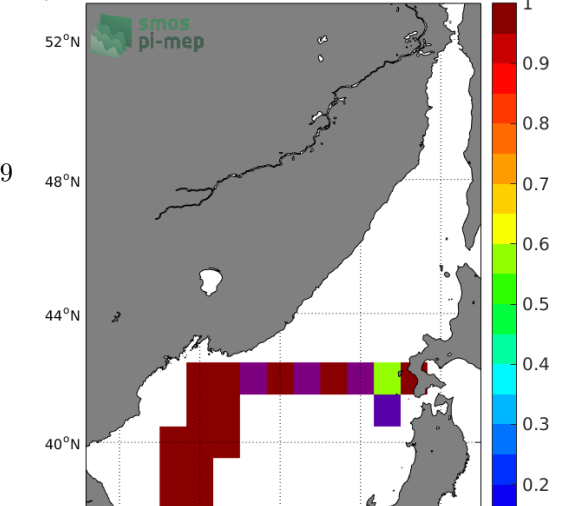
Temporal STD of (Sat-TSG-LEGOS-DM) in 1°x1° boxes over 2011-2016
