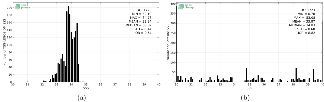
Figure 2: Histograms of SSS from TSG-LEGOS-DM (a) and SMOS-L3-CATDS-IFREMER-CECOS-V2-MONTHLY-0.25DEG (b) considering all match-up pairs per bins of 0.1 over the Sea of Japan Pi-MEP region and for the full satellite product period.
