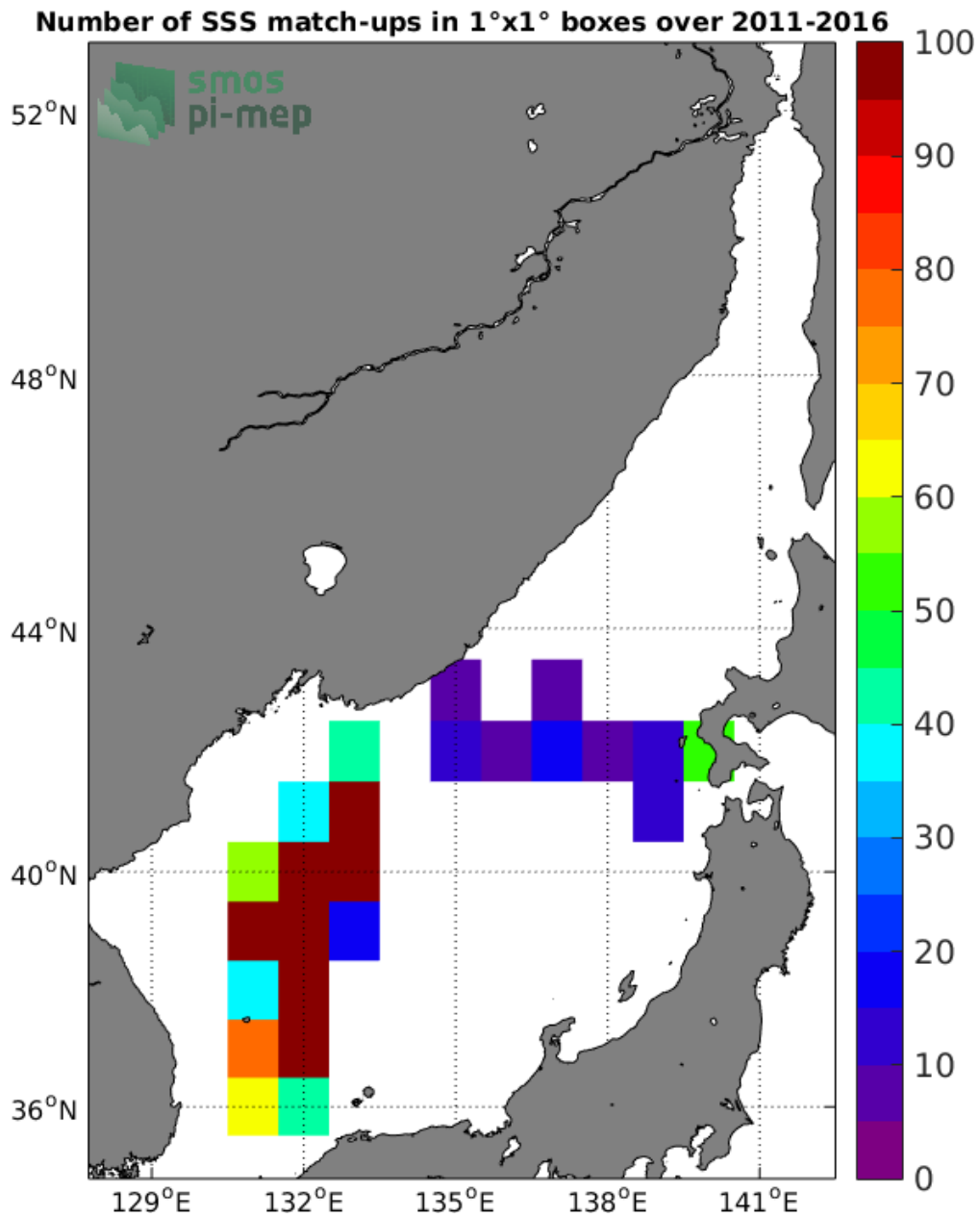
Figure 4: Number of SSS match-ups between TSG-LEGOS-DM SSS and the SMOS-L3-CATDS-IFREMER-CECOS-V2-MONTHLY-0.25DEG SSS product for the Sea of Japan Pi-MEP region over 1°x1° boxes and for the full satellite product period.
