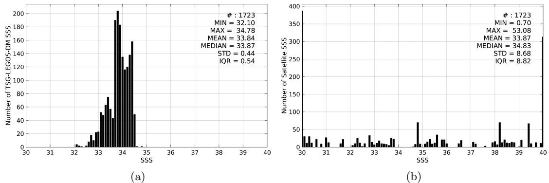
Figure 2: Histograms of SSS from TSG-LEGOS-DM (a) and SMOS-L3-CATDS-IFREMER-CECOS-V2-MONTHLY-0.25DEG (b) considering all match-up pairs per bins of 0.1 over the Sea of Japan Pi-MEP region and for the full satellite product period.
