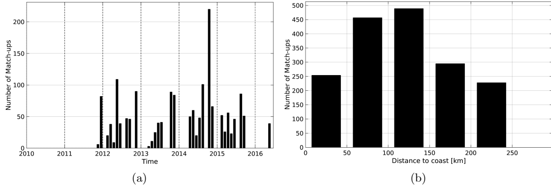
Figure 1: Number of match-ups between TSG-LEGOS-DM and SMOS-L3-CATDS-IFREMER-CECOS-V2-MONTHLY-0.25DEG SSS as a function of time (a) and as function of the distance to coast (b) over the Sea of Japan Pi-MEP region and for the full satellite product period.
