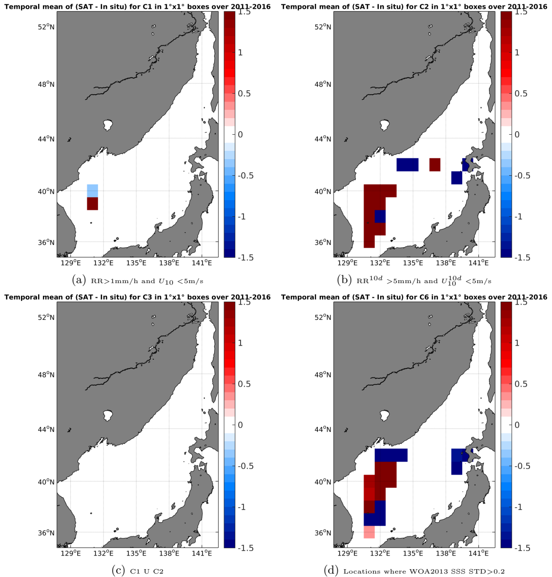
Figure 12: Temporal mean gridded over spatial boxes of size 1°x1° of \Delta SSS (SMOS-L3-CATDS-IFREMER-CECOS-V2-MONTHLY-0.25DEG - TSG-LEGOS-DM) for 4 different subdatasets corresponding to: RR > 1\text{mm/h} and U_{10} < 5\text{m/s} (a), RR^{10d} > 5\text{mm/h} and U_{10}^{10d} < 5\text{m/s} (b), C1 \cup C2 (c), Locations where WOA2013 SSS STD > 0.2 (d).
