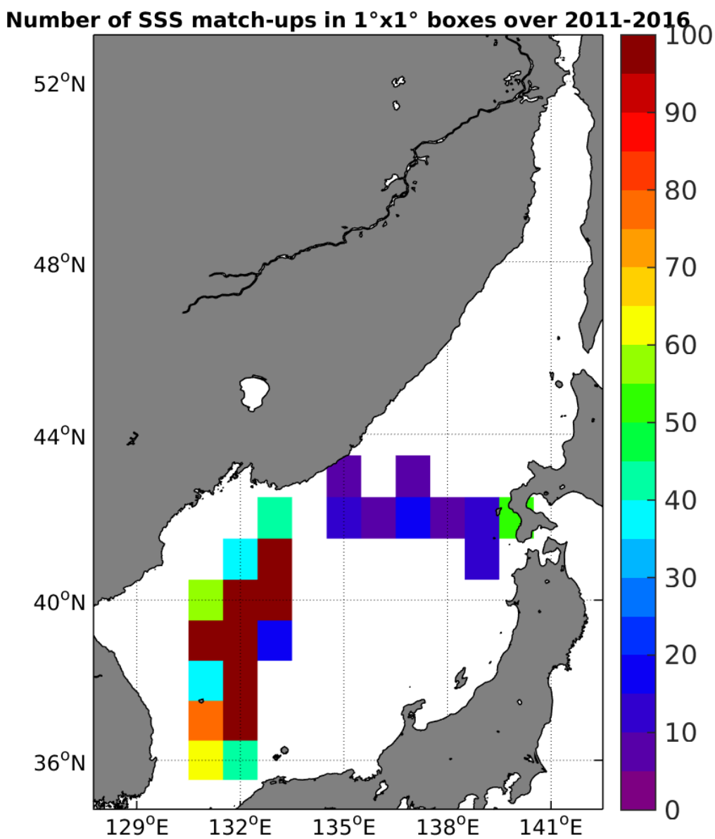
Figure 4: Number of SSS match-ups between TSG-LEGOS-DM SSS and the SMOS-L3-CATDS-IFREMER-CECOS-V2-MONTHLY-0.25DEG SSS product for the Sea of Japan Pi-MEP region over 1°x1° boxes and for the full satellite product period.
