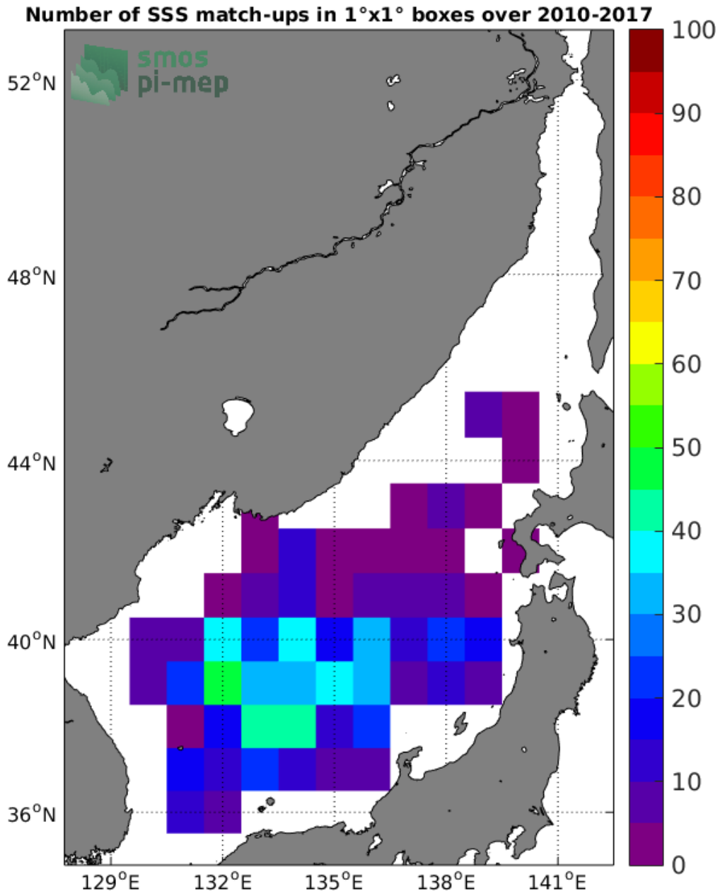
Figure 4: Number of SSS match-ups between Argo SSS and the SMOS-L3-CATDS-IFREMER-CECOS-V2-MONTHLY-0.25DEG SSS product for the Sea of Japan Pi-MEP region over 1°x1° boxes and for the full satellite product period.
