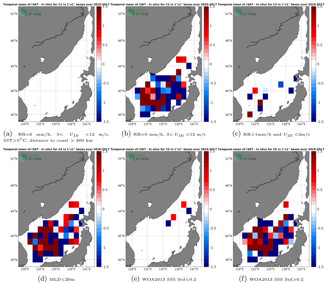
Figure 12: Temporal mean gridded over spatial boxes of size 1^\circ \times 1^\circ of \Delta SSS (SMOS-L3-CATDS-IFREMER-CECOS-V2-MONTHLY-0.25DEG - Argo) for 6 different subdatasets corresponding to: RR=0 mm/h, 3 < U_{10} < 12 m/s, SST > 5^\circ C , distance to coast > 800 km (a), RR=0 mm/h, 3 < U_{10} < 12 m/s (b), RR > 1 mm/h and U_{10} < 4 m/s (c), MLD < 20 m (d), WOA2013 SSS Std < 0.2 (e), WOA2013 SSS Std > 0.2 (f).
