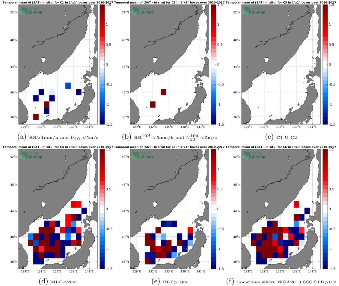
Figure 12: Temporal mean gridded over spatial boxes of size 1°x1° of \Delta SSS (SMOS-L3-CATDS-IFREMER-CECOS-V2-MONTHLY-0.25DEG - Argo) for 6 different subdatasets corresponding to:RR>1mm/h and U_{10} < 5\text{m/s} (a), RR^{10d} > 5\text{mm/h} and U_{10}^{10d} < 5\text{m/s} (b), C1 U C2 (c),MLD<20m (d),BLT>10m (e),Locations where WOA2013 SSS STD>0.2 (f).
