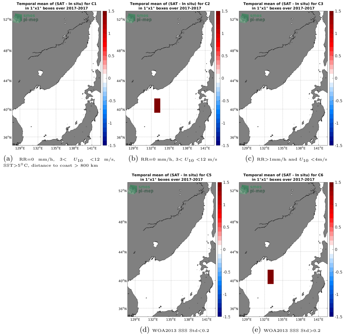
Figure 12: Temporal mean gridded over spatial boxes of size 1°x1° of \Delta SSS (SMOS SSS L3 v2 - Daily - 0.5 Deg (CATDS-CECOS-IFREMER) - TSG (LEGOS-DM)) for 5 different subdatasets corresponding to:RR=0 mm/h, 3 < U_{10} < 12 m/s, SST>5°C, distance to coast > 800 km (a), RR=0 mm/h, 3 < U_{10} < 12 m/s (b), RR>1mm/h and U_{10} < 4 m/s (c), WOA2013 SSS Std<0.2 (d), WOA2013 SSS Std>0.2 (e).
