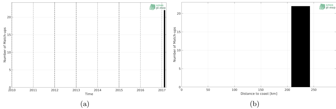
Figure 1: Number of match-ups between TSG (LEGOS-DM) and SMOS SSS L3 v2 - Daily - 0.5 Deg (CATDS-CECOS-IFREMER) SSS as a function of time (a) and as function of the distance to coast (b) over the Sea of Japan Pi-MEP region and for the full satellite product period.
