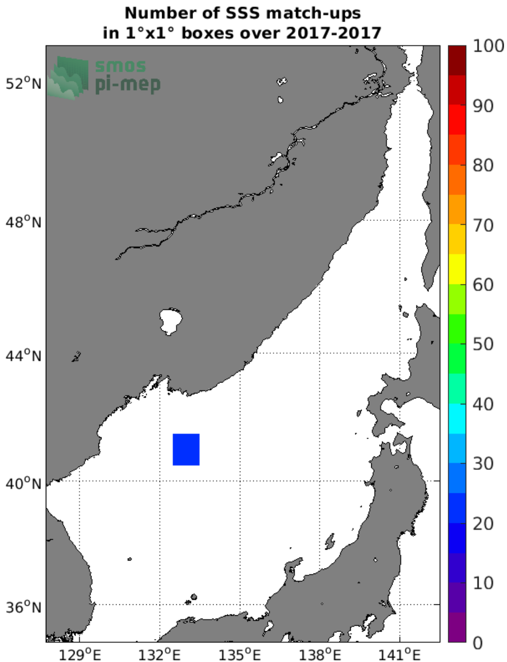
Figure 4: Number of SSS match-ups between TSG (LEGOS-DM) SSS and the SMOS SSS L3 v2 - Daily - 0.5 Deg (CATDS-CECOS-IFREMER) SSS product for the Sea of Japan Pi-MEP region over 1°x1° boxes and for the full satellite product period.
