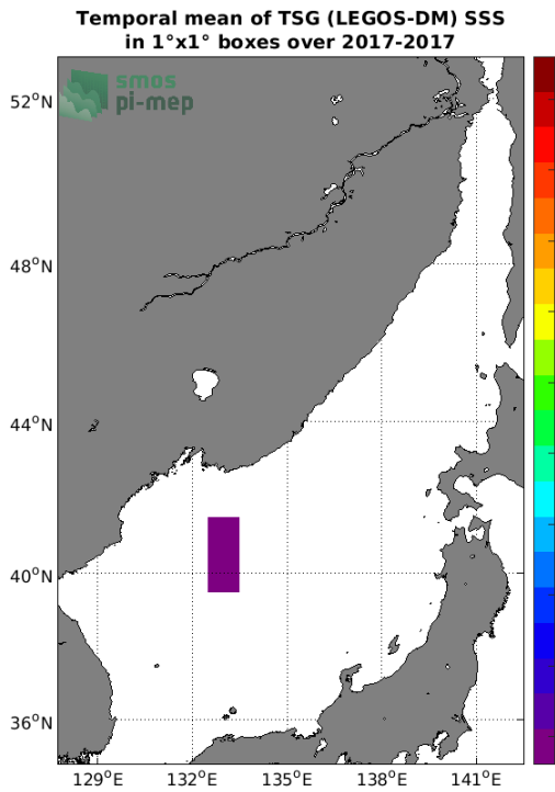
(c) MEAN(TSG (LEGOS-DM) SSS)
