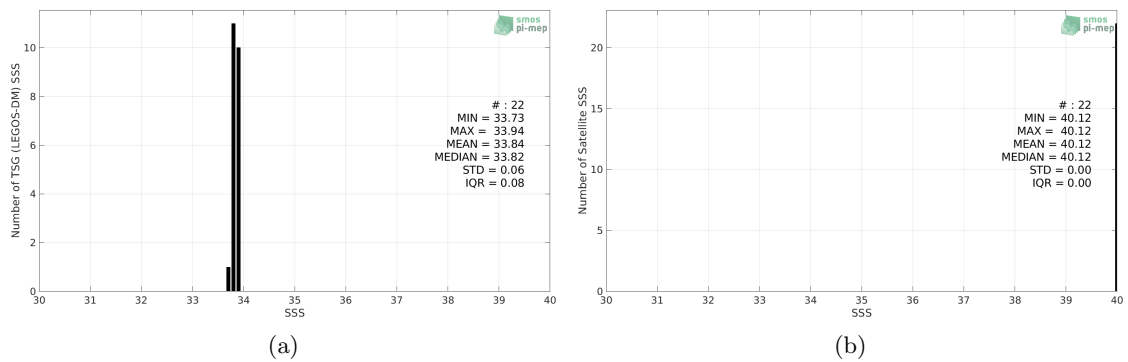
Figure 2: Histograms of SSS from TSG (LEGOS-DM) (a) and SMOS SSS L3 v2 - Daily - 0.5 Deg (CATDS-CECOS-IFREMER) (b) considering all match-up pairs per bins of 0.1 over the Sea of Japan Pi-MEP region and for the full satellite product period.
