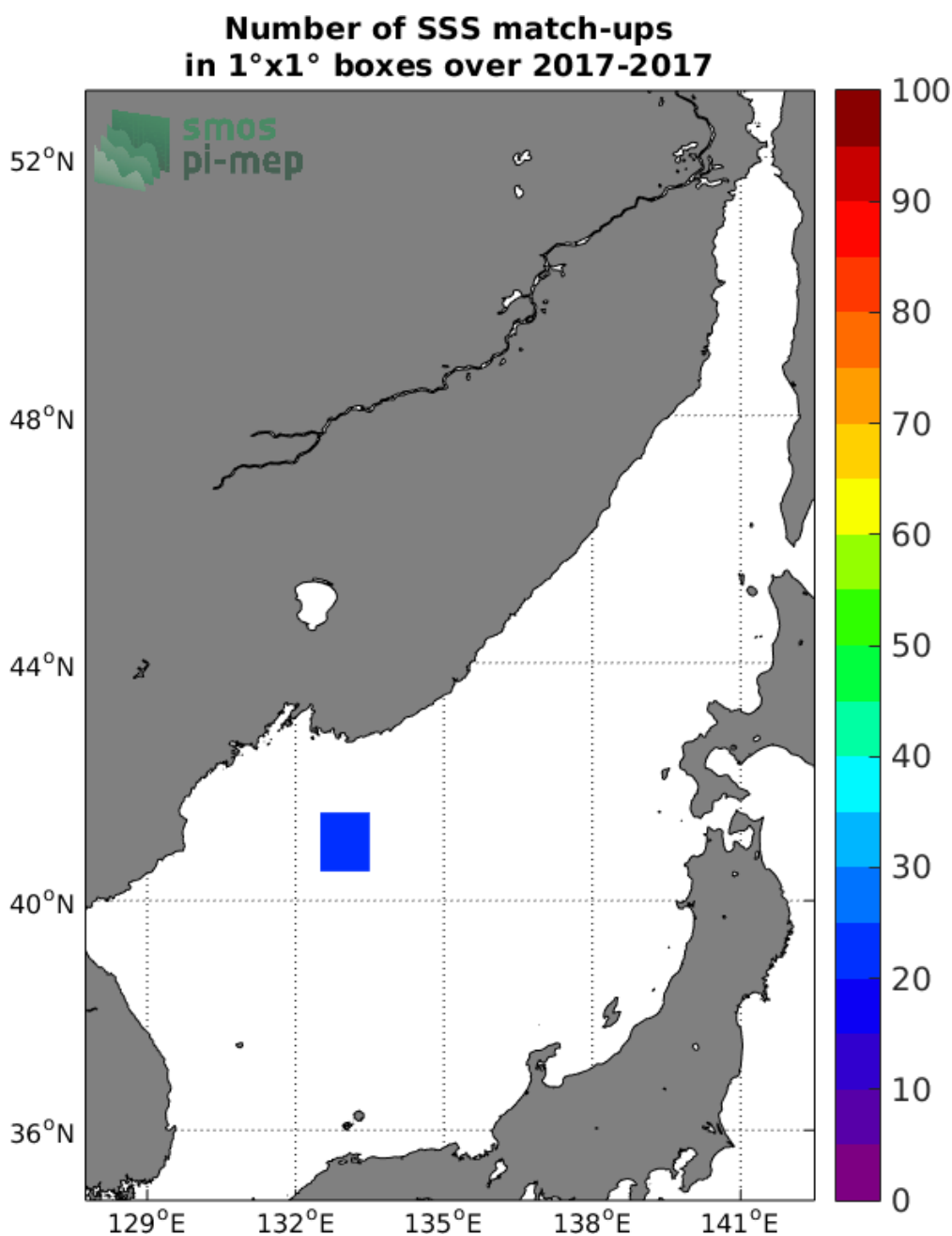
Figure 4: Number of SSS match-ups between TSG-LEGOS-DM SSS and the SMOS L3 v2 - Daily - 0.5 Deg (CATDS-CECOS-IFREMER) SSS product for the Sea of Japan Pi-MEP region over 1°x1° boxes and for the full satellite product period.
