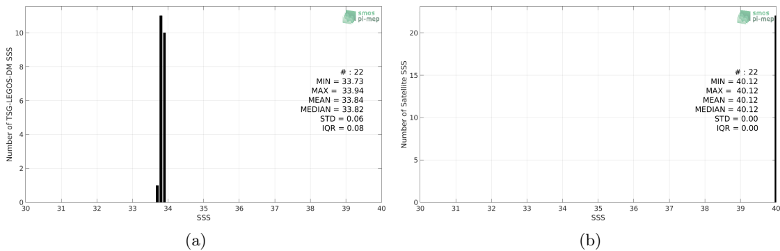
Figure 2: Histograms of SSS from TSG-LEGOS-DM (a) and SMOS L3 v2 - Daily - 0.5 Deg (CATDS-CECOS-IFREMER) (b) considering all match-up pairs per bins of 0.1 over the Sea of Japan Pi-MEP region and for the full satellite product period.
