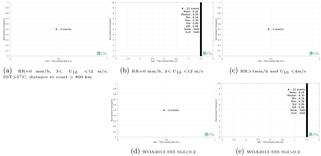
Figure 13: Normalized histogram of \Delta SSS (SMOS L3 v2 - Daily - 0.5 Deg (CATDS-CECOS-IFREMER) - TSG-LEGOS-DM) for 5 different subdatasets corresponding to: RR=0 mm/h, 3 < U_{10} < 12 m/s, SST>5°C, distance to coast > 800 km (a), RR=0 mm/h, 3 < U_{10} < 12 m/s (b), RR>1mm/h and U_{10} < 4 m/s (c), WOA2013 SSS Std<0.2 (d), WOA2013 SSS Std>0.2 (e).
