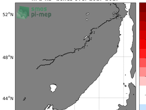
Temporal mean of (Sat - TSG-LEGOS-DM) in 1°x1° boxes over 2017-2017
