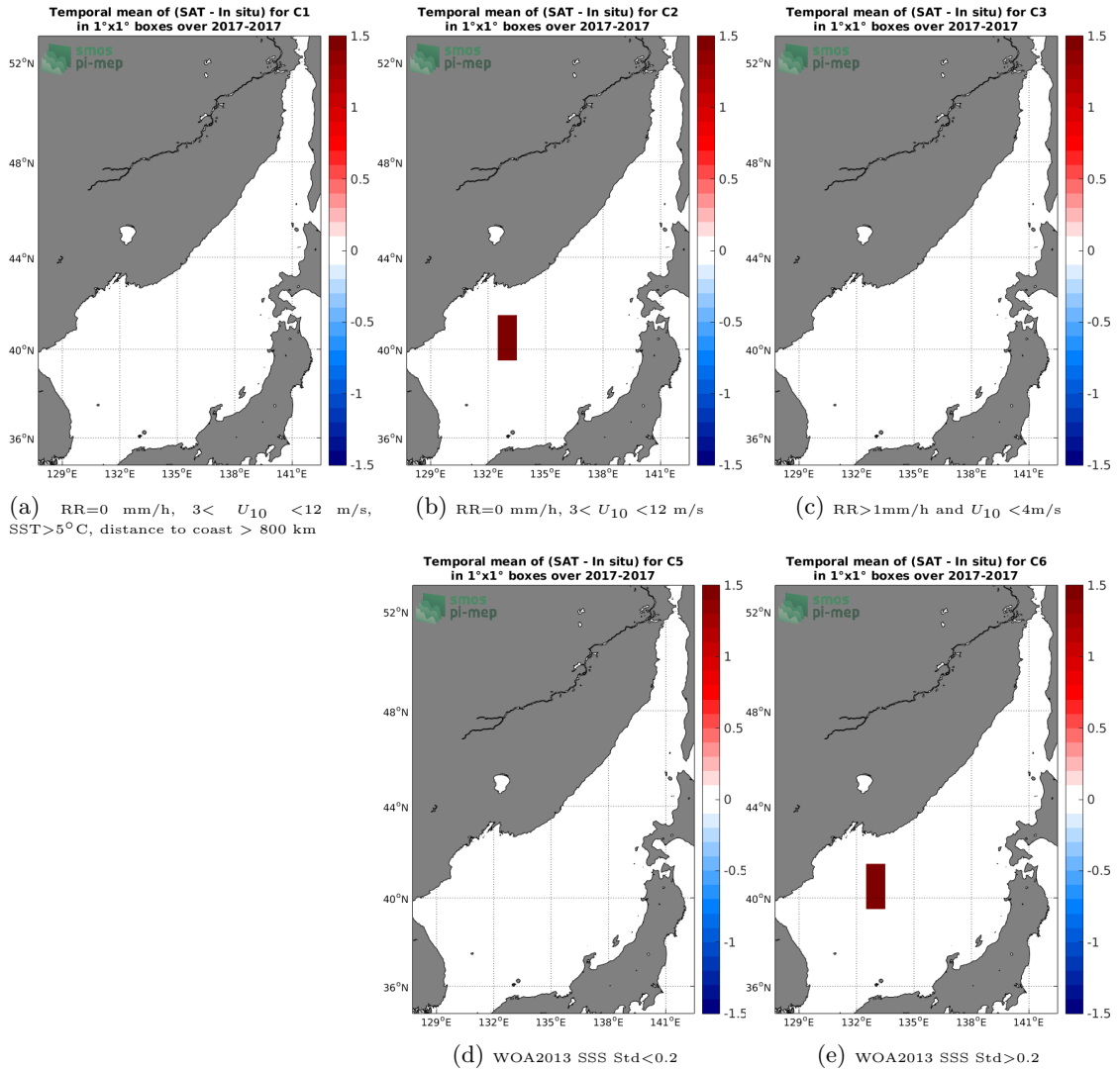
Figure 12: Temporal mean gridded over spatial boxes of size 1°x1° of \Delta SSS (SMOS L3 v2 - Daily - 0.5 Deg (CATDS-CECOS-IFREMER) - TSG-LEGOS-DM) for 5 different subdatasets corresponding to:RR=0 mm/h, 3 < U_{10} < 12 m/s, SST>5°C, distance to coast > 800 km (a), RR=0 mm/h, 3 < U_{10} < 12 m/s (b), RR>1mm/h and U_{10} < 4 m/s (c), WOA2013 SSS Std<0.2 (d), WOA2013 SSS Std>0.2 (e).
