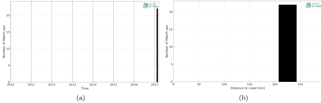
Figure 1: Number of match-ups between TSG-LEGOS-DM and SMOS L3 v2 - Daily - 0.5 Deg (CATDS-CECOS-IFREMER) SSS as a function of time (a) and as function of the distance to coast (b) over the Sea of Japan Pi-MEP region and for the full satellite product period.
