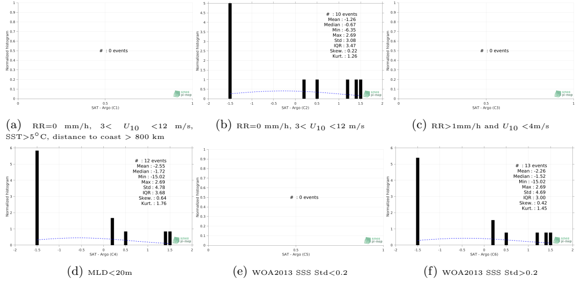
Figure 13: Normalized histogram of \Delta SSS (SMOS SSS L3 v2 - Daily - 0.5 Deg (CATDS-CECOS-IFREMER) - Argo) for 6 different subdatasets corresponding to: RR=0 mm/h, 3 < U_{10} < 12 m/s, SST > 5°C, distance to coast > 800 km (a), RR=0 mm/h, 3 < U_{10} < 12 m/s (b), RR > 1mm/h and U_{10} < 4 m/s (c), MLD < 20m (d), WOA2013 SSS Std < 0.2 (e), WOA2013 SSS Std > 0.2 (f).
