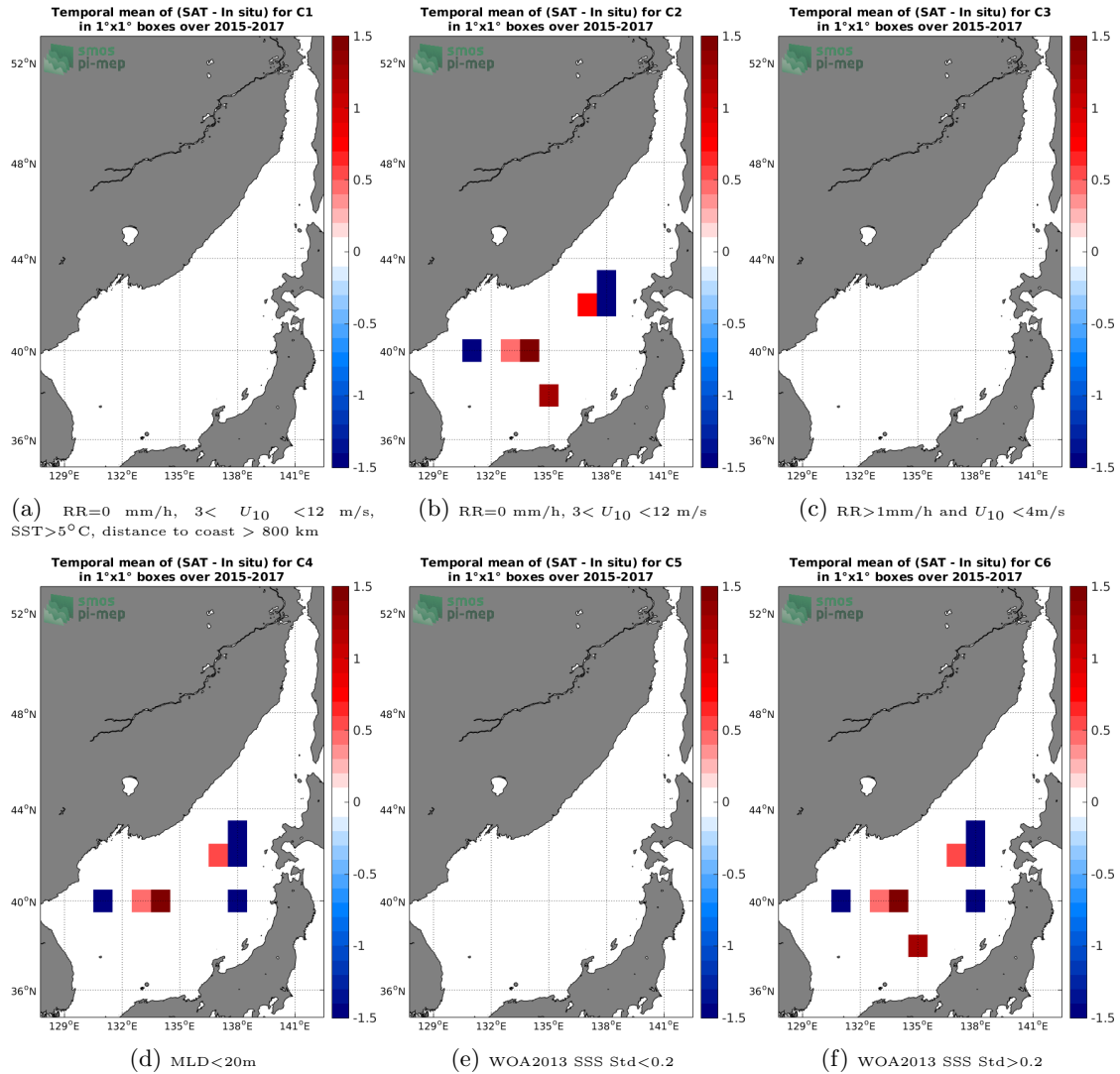
Figure 12: Temporal mean gridded over spatial boxes of size 1°x1° of \Delta SSS (SMOS SSS L3 v2 - Daily - 0.5 Deg (CATDS-CECOS-IFREMER) - Argo) for 6 different subdatasets corresponding to:RR=0 mm/h, 3 < U_{10} < 12 m/s, SST>5°C, distance to coast > 800 km (a), RR=0 mm/h, 3 < U_{10} < 12 m/s (b), RR>1mm/h and U_{10} < 4 m/s (c),MLD<20m (d),WOA2013 SSS Std<0.2 (e),WOA2013 SSS Std>0.2 (f).
