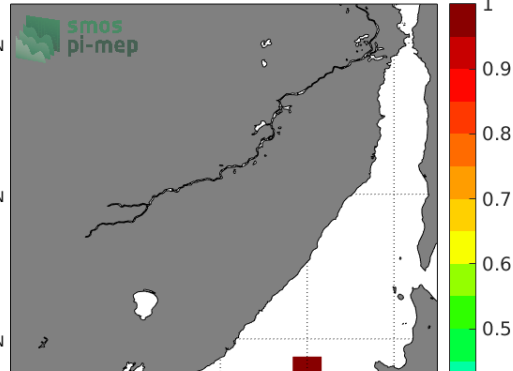
Temporal STD of (Sat - Argo) in 1°x1° boxes over 2015-2017
