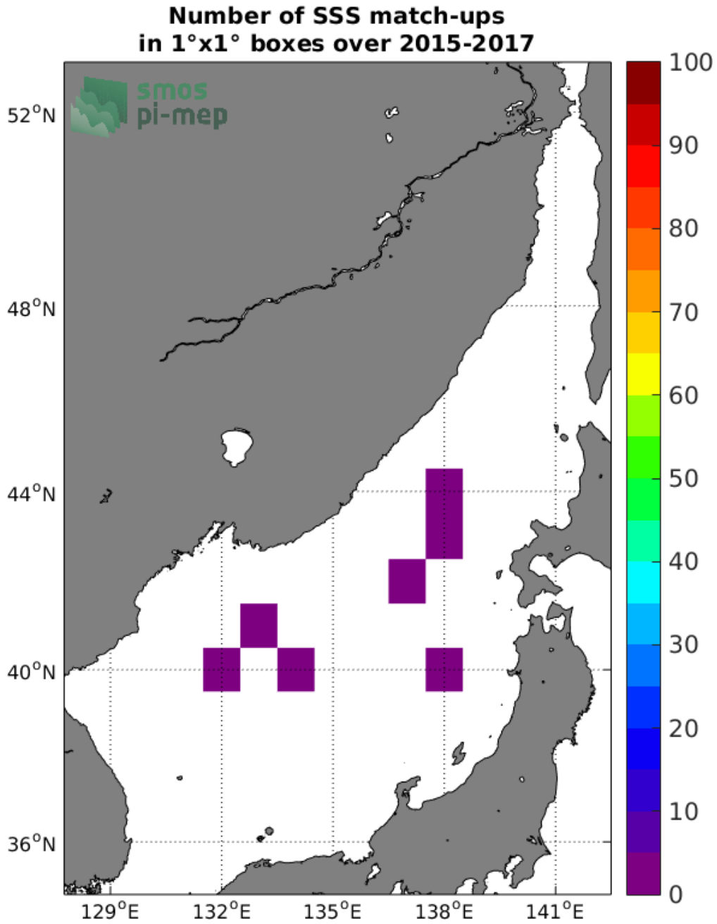
Figure 4: Number of SSS match-ups between Argo SSS and the SMOS L3 v2 - Daily - 0.5 Deg (CATDS-CECOS-IFREMER) SSS product for the Sea of Japan Pi-MEP region over 1°x1° boxes and for the full satellite product period.
