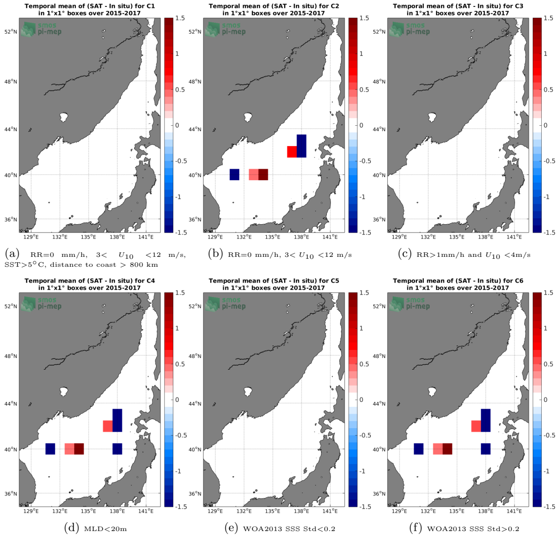
Figure 12: Temporal mean gridded over spatial boxes of size 1^\circ \times 1^\circ of \Delta\text{SSS} (SMOS L3 v2 - Daily - 0.5 Deg (CATDS-CECOS-IFREMER) - Argo) for 6 different subdatasets corresponding to: RR=0 mm/h, 3 < U_{10} < 12 m/s, SST > 5^\circ\text{C} , distance to coast > 800 km (a), RR=0 mm/h, 3 < U_{10} < 12 m/s (b), RR > 1 mm/h and U_{10} < 4 m/s (c), MLD < 20 m (d), WOA2013 SSS Std < 0.2 (e), WOA2013 SSS Std > 0.2 (f).
