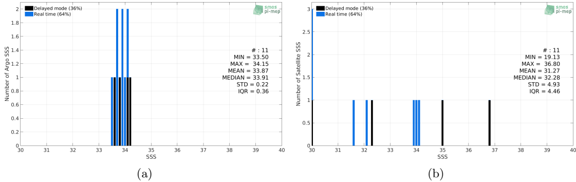
Figure 2: Histograms of SSS from Argo (a) and SMOS L3 v2 - Daily - 0.5 Deg (CATDS-CECOS-IFREMER) (b) considering all match-up pairs per bins of 0.1 over the Sea of Japan Pi-MEP region and for the full satellite product period.
