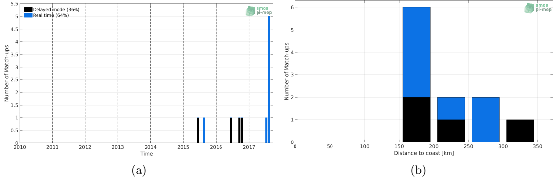
Figure 1: Number of match-ups between Argo and SMOS L3 v2 - Daily - 0.5 Deg (CATDS-CECOS-IFREMER) SSS as a function of time (a) and as function of the distance to coast (b) over the Sea of Japan Pi-MEP region and for the full satellite product period.
