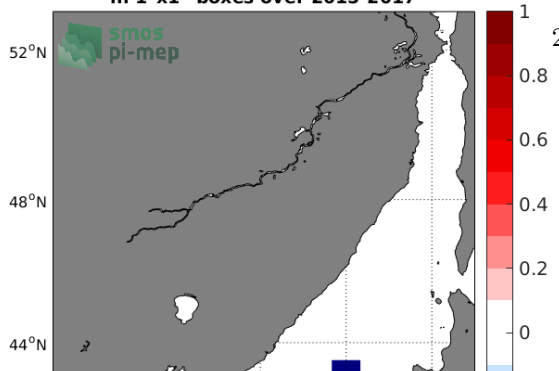
Temporal mean of (Sat - Argo) in 1°x1° boxes over 2015-2017
