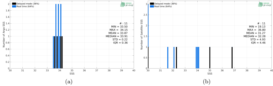
Figure 2: Histograms of SSS from Argo (a) and SMOS-L3-CATDS-CECOS-IFREMER-V2-1DAY-0.5DEG (b) considering all match-up pairs per bins of 0.1 over the Sea of Japan Pi-MEP region and for the full satellite product period.
