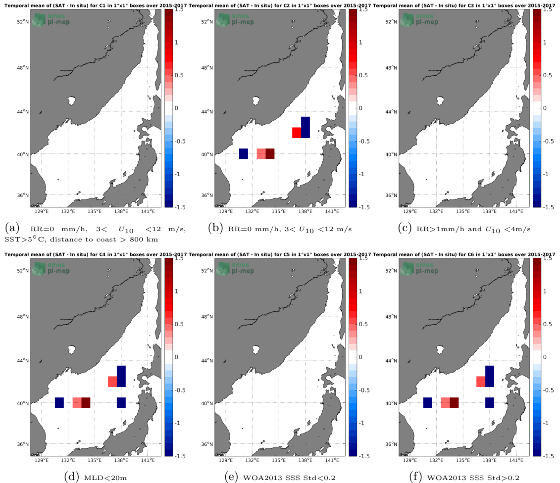
Figure 12: Temporal mean gridded over spatial boxes of size 1^\circ \times 1^\circ of \Delta SSS (SMOS-L3-CATDS-CECOS-IFREMER-V2-1DAY-0.5DEG - Argo) for 6 different subdatasets corresponding to:RR=0 mm/h, 3 < U_{10} < 12 m/s, SST >5^\circ C, distance to coast > 800 km (a), RR=0 mm/h, 3 < U_{10} < 12 m/s (b), RR >1 mm/h and U_{10} < 4 m/s (c),MLD <20 m (d),WOA2013 SSS Std <0.2 (e),WOA2013 SSS Std >0.2 (f).
