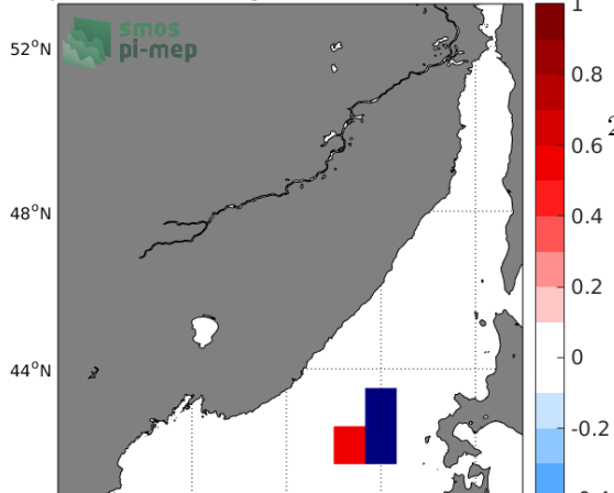
Temporal mean of (Sat-Argo) in 1°x1° boxes over 2015-2017
