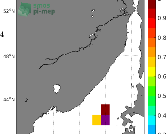
Temporal STD of (Sat-Argo) in 1°x1° boxes over 2015-2017
