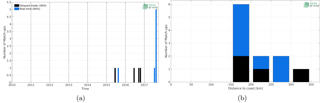
Figure 1: Number of match-ups between Argo and SMOS-L3-CATDS-CECOS-IFREMER-V2-1DAY-0.5DEG SSS as a function of time (a) and as function of the distance to coast (b) over the Sea of Japan Pi-MEP region and for the full satellite product period.
