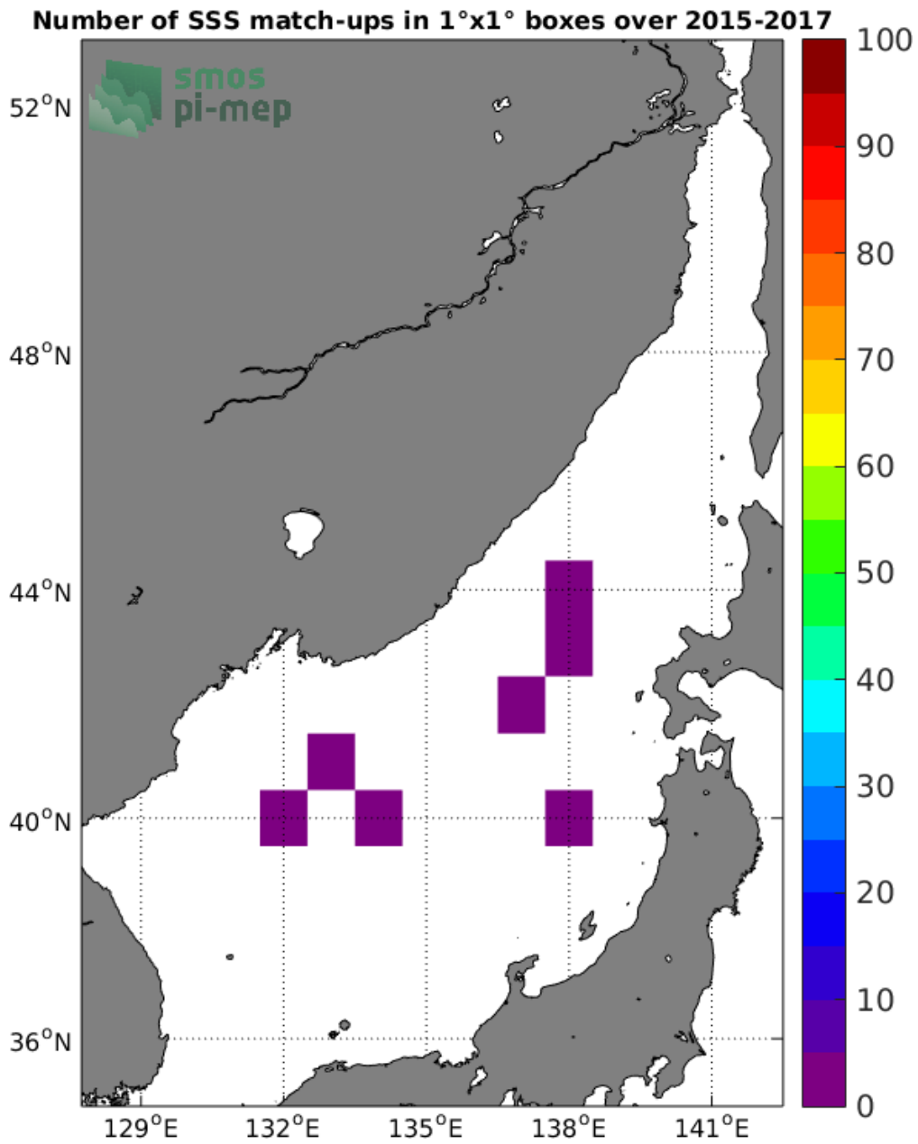
Figure 4: Number of SSS match-ups between Argo SSS and the SMOS-L3-CATDS-CECOS-IFREMER-V2-1DAY-0.5DEG SSS product for the Sea of Japan Pi-MEP region over 1°x1° boxes and for the full satellite product period.
