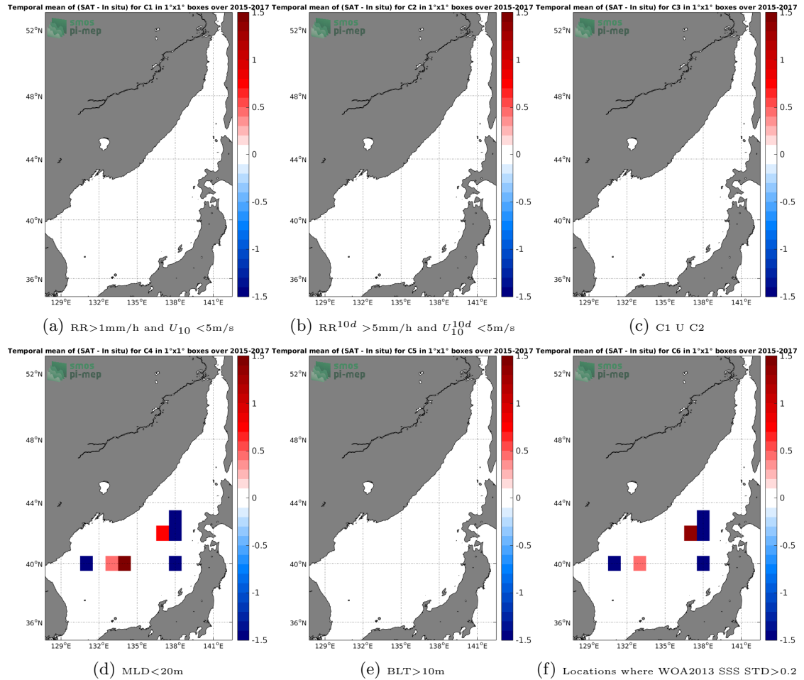
Figure 12: Temporal mean gridded over spatial boxes of size 1^\circ \times 1^\circ of \Delta SSS (SMOS-L3-CATDS-CECOS-IFREMER-V2-1DAY-0.5DEG - Argo) for 6 different subdatasets corresponding to: RR > 1mm/h and U_{10} < 5 m/s (a), RR^{10d} > 5 mm/h and U_{10}^{10d} < 5 m/s (b), C1 U C2 (c), MLD < 20m (d), BLT > 10m (e), Locations where WOA2013 SSS STD > 0.2 (f).
