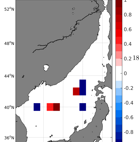
Temporal mean of (Sat-Argo) in 1°x1° boxes over 2015-2017
