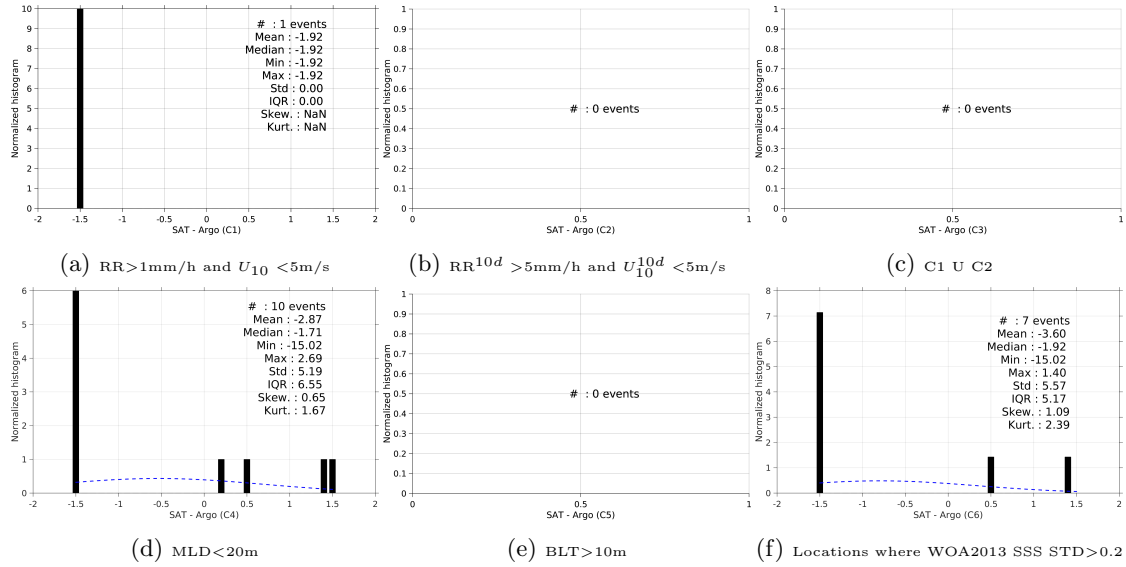
Figure 13: Normalized histogram of \Delta\text{SSS} (SMOS-L3-CATDS-CECOS-IFREMER-V2-1DAY-0.5deg - Argo) for 6 different subdatasets corresponding to: RR > 1\text{mm/h} and U_{10} < 5\text{m/s} (a), RR^{10d} > 5\text{mm/h} and U_{10}^{10d} < 5\text{m/s} (b), C1 U C2 (c), MLD < 20\text{m} (d), BLT > 10\text{m} (e), Locations where WOA2013 SSS STD > 0.2 (f).
