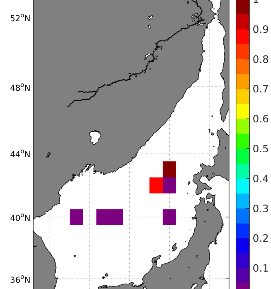
Temporal STD of (Sat-Argo) in 1°x1° boxes over 2015-2017
